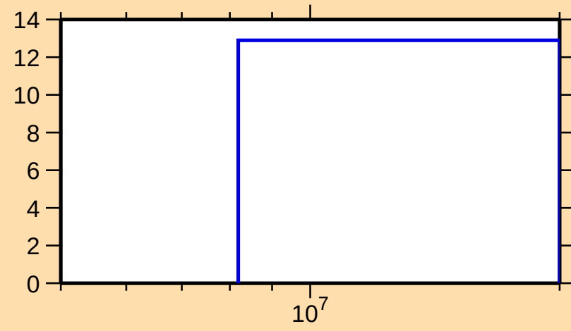
\Delta\sigma/\sigma vs. E for ^{122}\text{Ba}(n,\text{nonel.})
