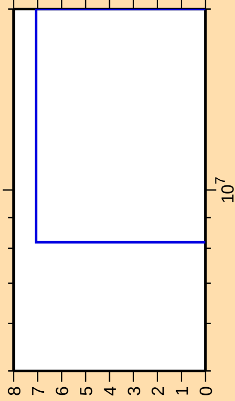
\Delta\sigma/\sigma vs. E for ^{122}\text{Ba}(\text{mt } 34)
