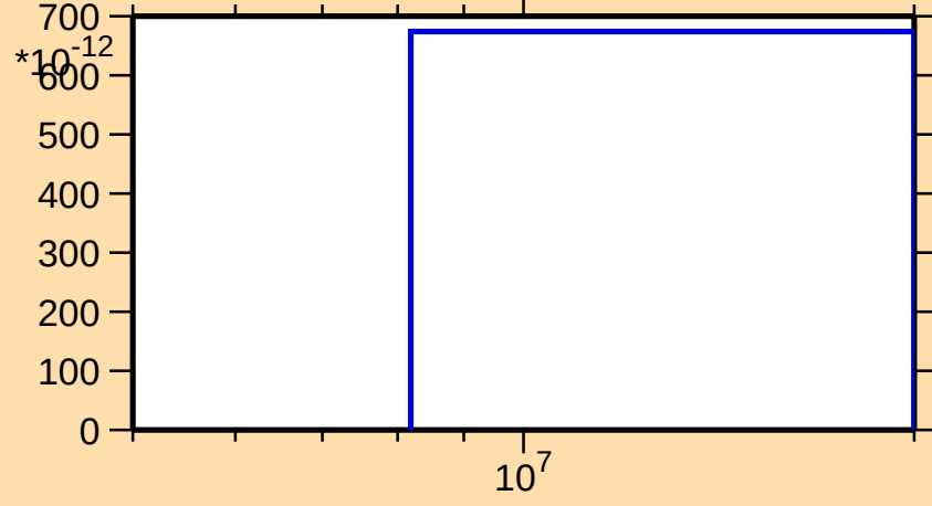
\sigma vs. E for ^{122}\text{Ba}(n,\text{pt})
