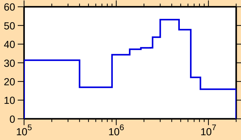
\Delta\sigma/\sigma vs. E for ^{122}\text{Ba}(n,\text{el.})
