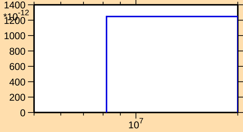
\sigma vs. E for ^{122}\text{Ba}(\text{mt117})
