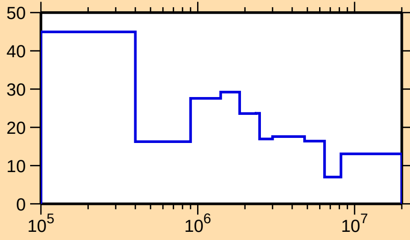
\Delta\sigma/\sigma vs. E for ^{122}\text{Ba}(n,\text{tot.})
