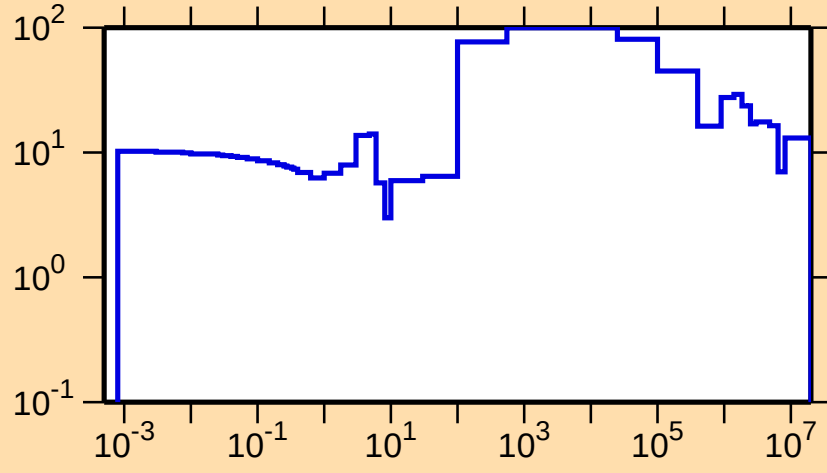
\Delta\sigma/\sigma vs. E for ^{122}\text{Ba}(n,\text{tot.})
