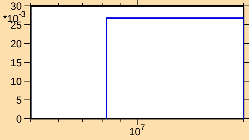
\sigma vs. E for ^{122}\text{Ba}(n,2n)
