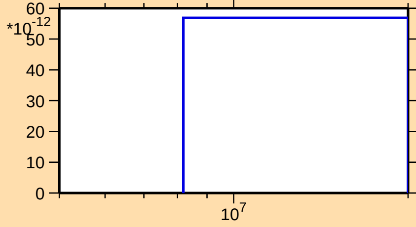
\sigma vs. E for ^{122}\text{Ba}(n,2n\alpha)
