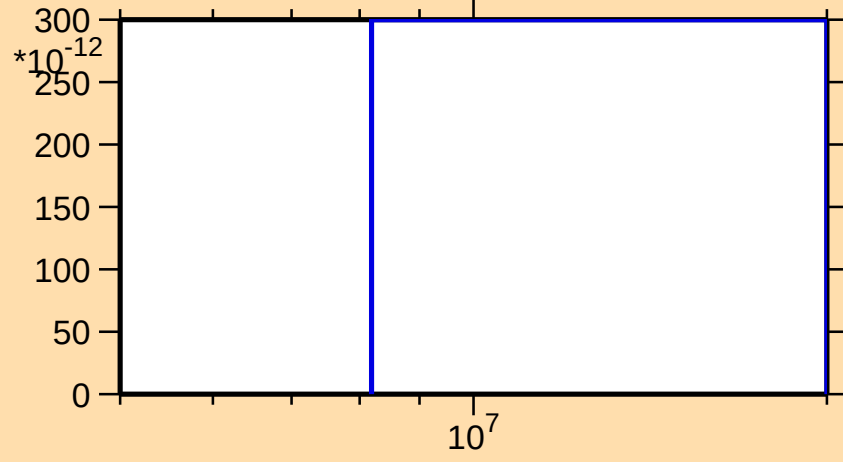
\sigma vs. E for ^{122}\text{Ba}(n,\text{nd})
