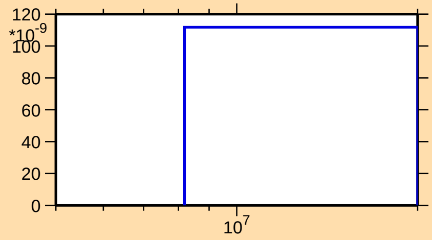
\sigma vs. E for ^{122}\text{Ba} (mt 45)
