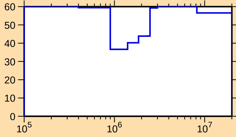
\Delta\sigma/\sigma vs. E for ^{122}\text{Ba}(n,\text{inel.})
