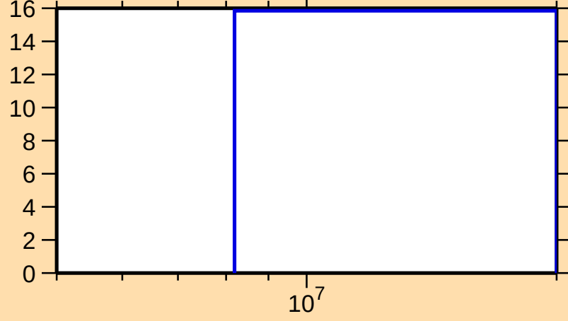
\Delta\sigma/\sigma vs. E for ^{122}\text{Ba}(n,\text{el.})
