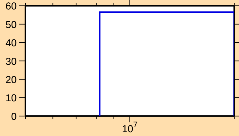
\Delta\sigma/\sigma vs. E for ^{122}\text{Ba}(n,\text{inel.})
