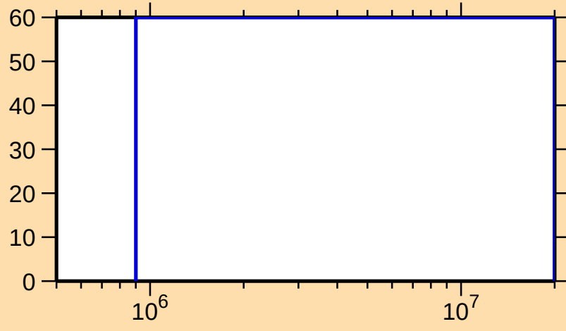
\Delta\sigma/\sigma vs. E for ^{122}\text{Ba}(n,n\text{cont.})
