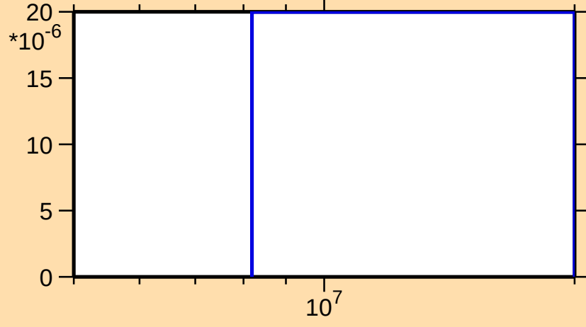
\sigma vs. E for ^{122}\text{Ba}(n,\text{pd})
