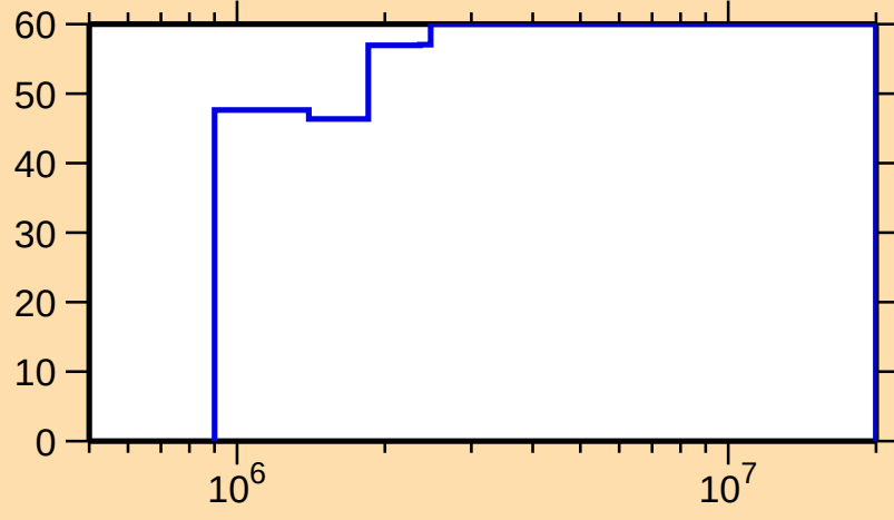
\Delta\sigma/\sigma vs. E for ^{122}\text{Ba}(n,n_1)
