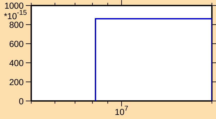
\sigma vs. E for ^{122}\text{Ba}(\text{mt } 34)
