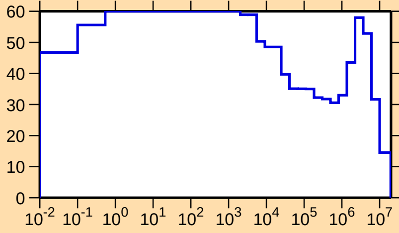
\Delta\sigma/\sigma vs. E for ^{127}\text{Ba}(n,p)
