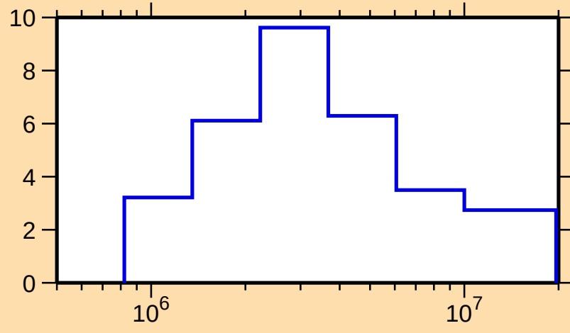
\Delta\sigma/\sigma vs. E for ^{127}\text{Ba}(n,\text{el.})
