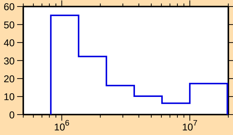
\Delta\sigma/\sigma vs. E for ^{127}\text{Ba}(n,n\text{cont.})
