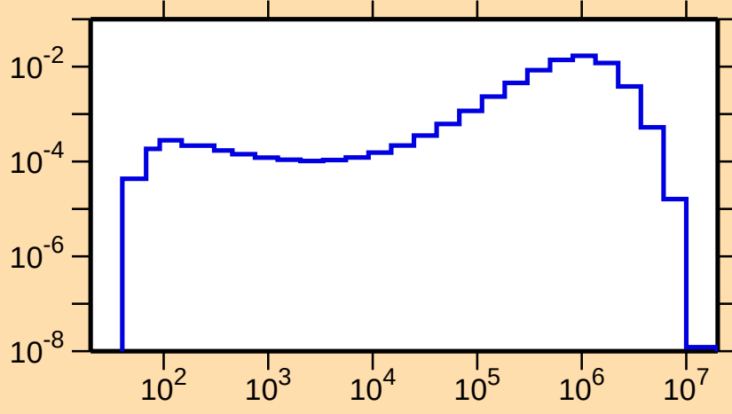
\sigma vs. E for ^{127}\text{Ba}(n,n_1)
