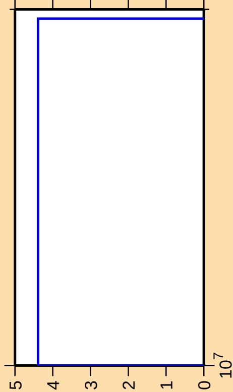
\Delta\sigma/\sigma vs. E for ^{127}\text{Ba} (mt 34)
