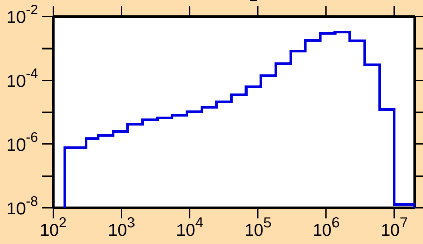
\sigma vs. E for ^{133}\text{Ba}(n,n_1)
