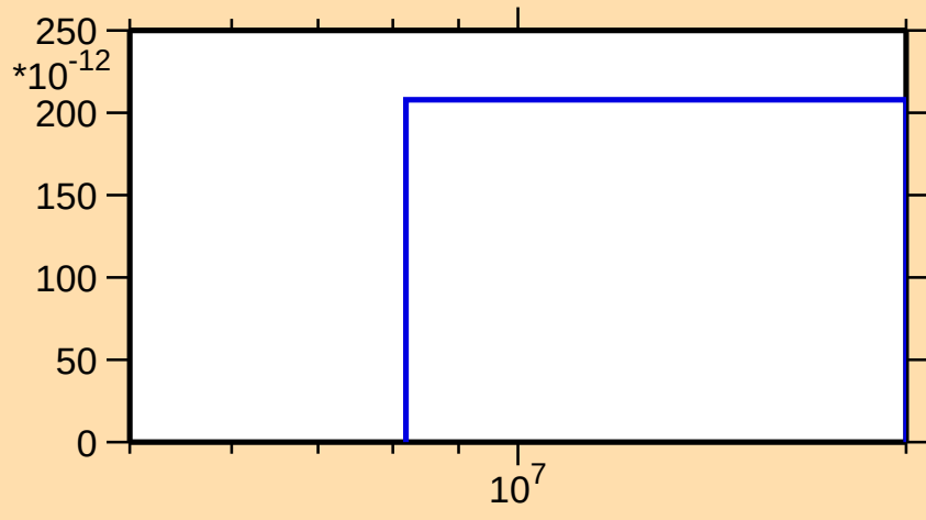
\sigma vs. E for ^{133}\text{Ba}(n,p\alpha)
