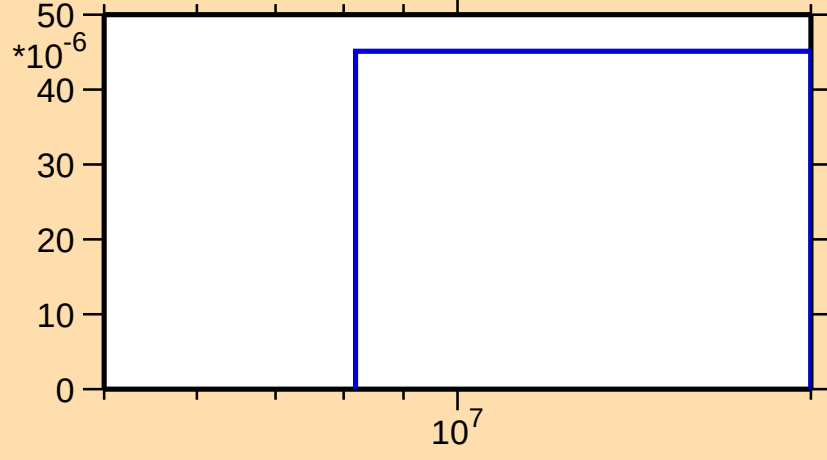
\sigma vs. E for ^{133}\text{Ba}(n,t)
