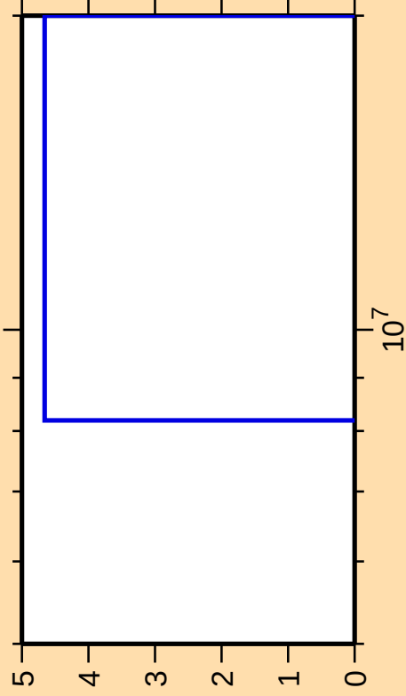
\Delta\sigma/\sigma vs. E for ^{133}\text{Ba}(n,nt)
