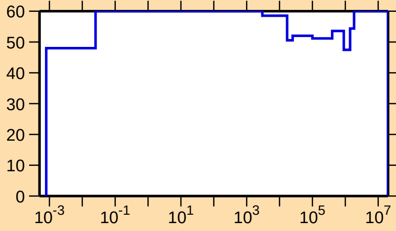
\Delta\sigma/\sigma vs. E for ^{133}\text{Ba}(n,p)
