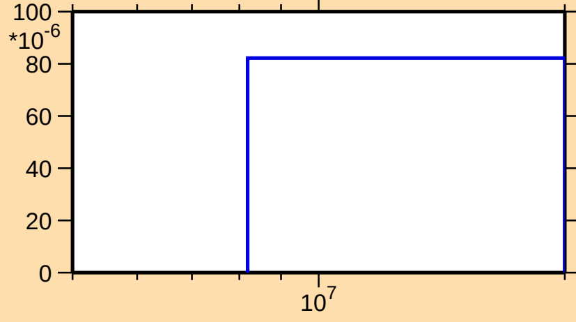
\sigma vs. E for ^{133}\text{Ba}(n,3n)
