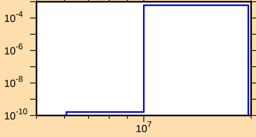
\sigma vs. E for ^{134}\text{Ba}(n,d)
