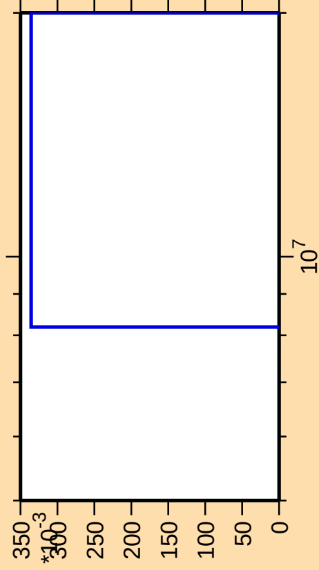
\Delta\sigma/\sigma vs. E for ^{134}\text{Ba}(n,2np)
