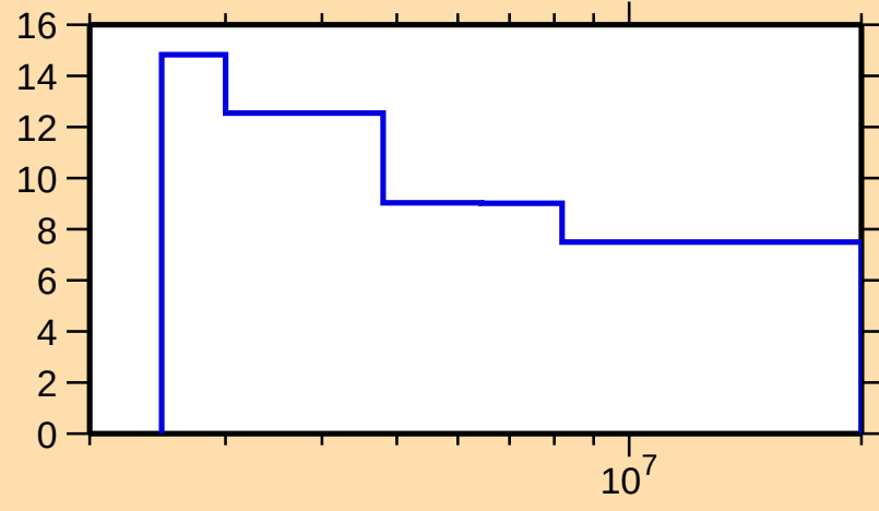
\Delta\sigma/\sigma vs. E for ^{134}\text{Ba}(n,n\text{onel.})
