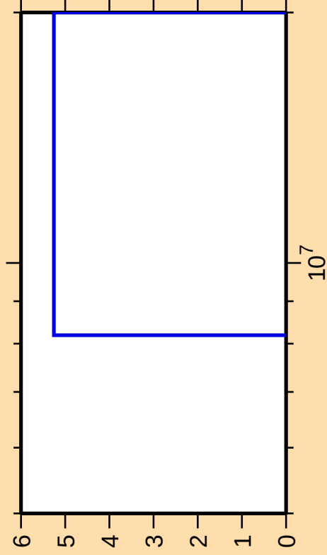
\Delta\sigma/\sigma vs. E for ^{134}\text{Ba}(n,2n)
