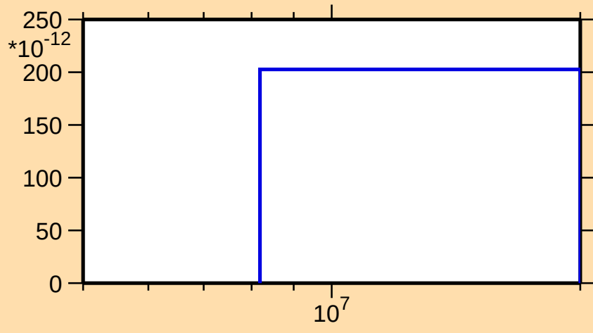
\sigma vs. E for ^{134}\text{Ba}(n,\text{He}3)
