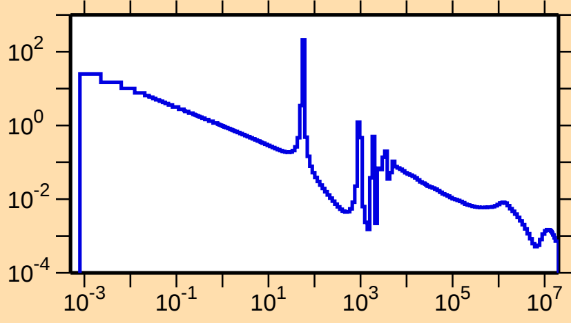
\sigma vs. E for ^{139}\text{Ba}(n,\gamma)
