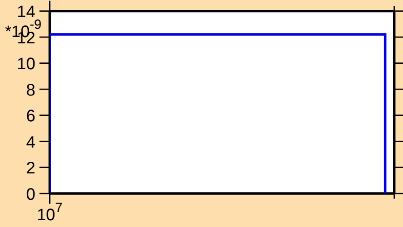
\sigma vs. E for ^{139}\text{Ba}(n,2np)
