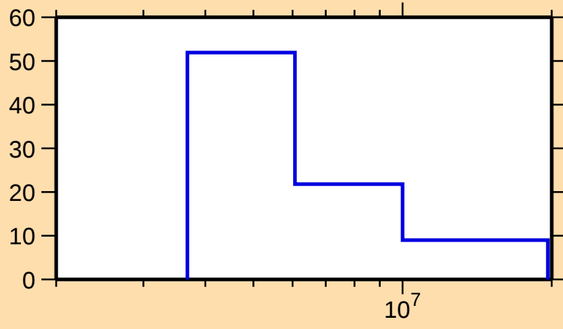
\Delta\sigma/\sigma vs. E for ^{139}\text{Ba}(n,2n)
