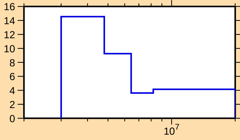
\Delta\sigma/\sigma vs. E for ^{139}\text{Ba}(n,\text{tot.})
