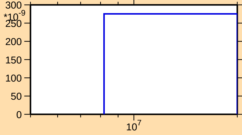
\sigma vs. E for ^{139}\text{Ba}(n,\text{nd})
