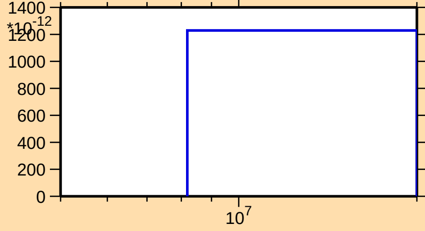
\sigma vs. E for ^{139}\text{Ba}(n,nt)
