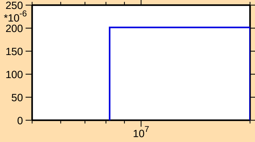
\sigma vs. E for ^{139}\text{Ba}(n,d)
