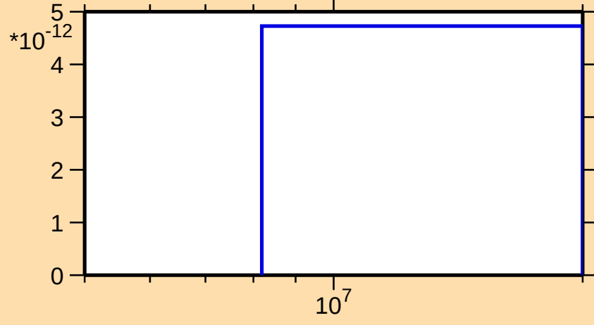
\sigma vs. E for ^{139}\text{Ba}(n,p\alpha)
