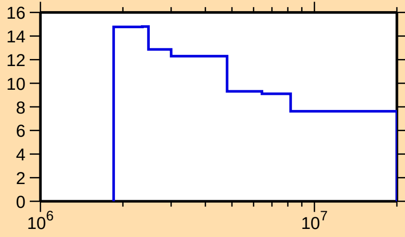
\Delta\sigma/\sigma vs. E for ^{139}\text{Ba}(n,\text{nonel.})
