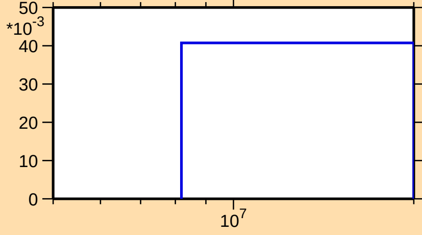
\sigma vs. E for ^{139}\text{Ba}(n,3n)
