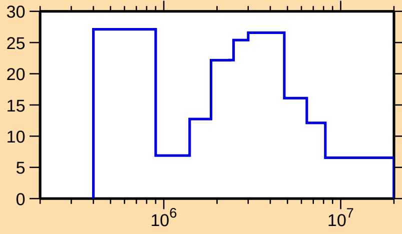
\Delta\sigma/\sigma vs. E for ^{139}\text{Ba}(n,\text{el.})
