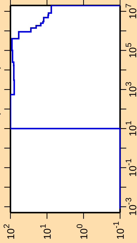
\Delta\sigma/\sigma vs. E for ^{139}\text{Ba}(n,\text{nonel.})
