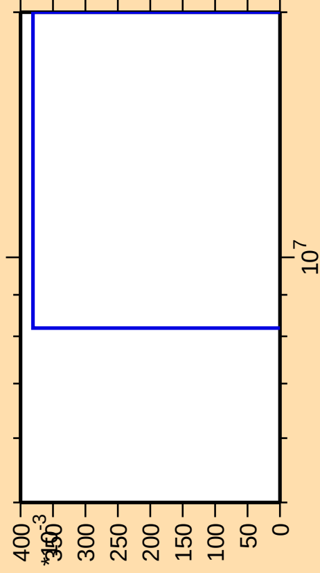
\Delta\sigma/\sigma vs. E for ^{139}\text{Ba}(n,\text{He}3)
