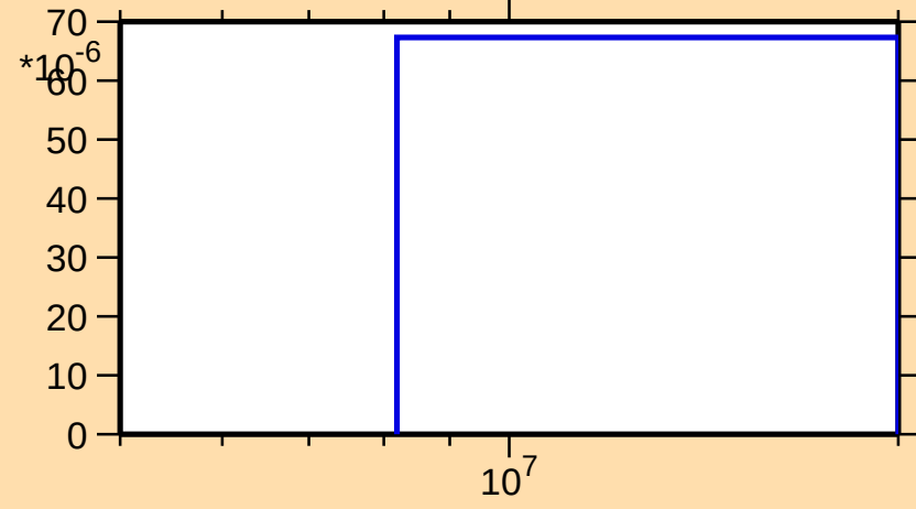
\sigma vs. E for ^{139}\text{Ba}(n,np)
