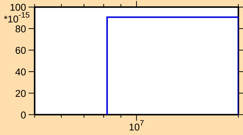
\sigma vs. E for ^{139}\text{Ba}(n,\text{He}3)
