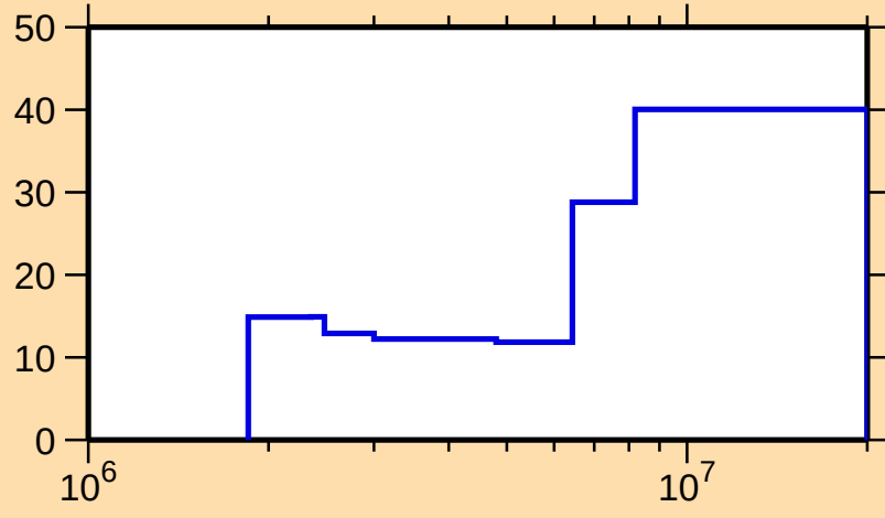
\Delta\sigma/\sigma vs. E for ^{139}\text{Ba}(n,\text{inel.})
