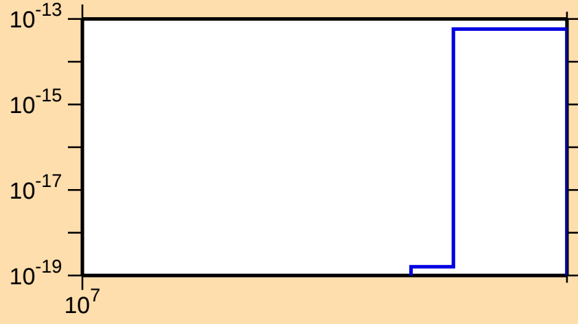
\sigma vs. E for ^{141}\text{Ba}(n,\text{He}3)
