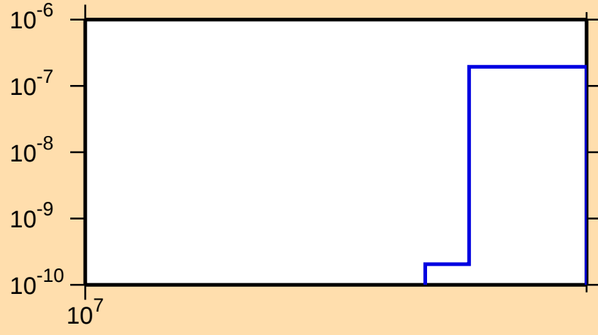
\sigma vs. E for ^{141}\text{Ba}(n,2np)
