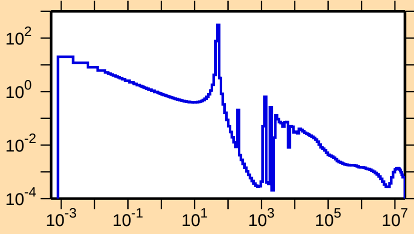
\sigma vs. E for ^{141}\text{Ba}(n,\gamma)
