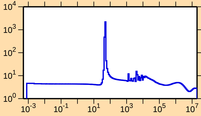
\sigma vs. E for ^{141}\text{Ba}(n,\text{el.})
