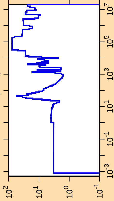
\Delta\sigma/\sigma vs. E for ^{141}\text{Ba}(n,\text{el.})
