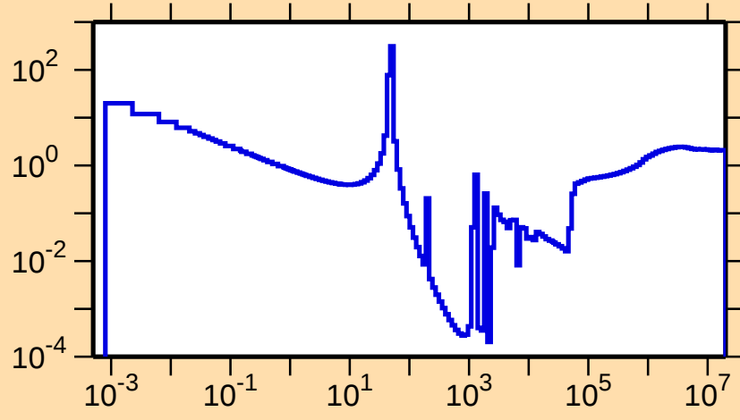
\sigma vs. E for ^{141}\text{Ba}(n,\text{nonel.})
