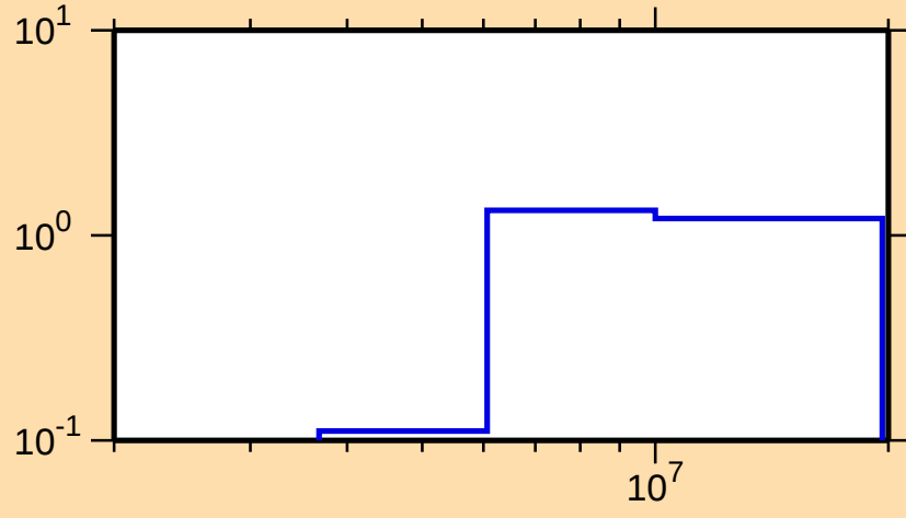
\sigma vs. E for ^{141}\text{Ba}(n,2n)
