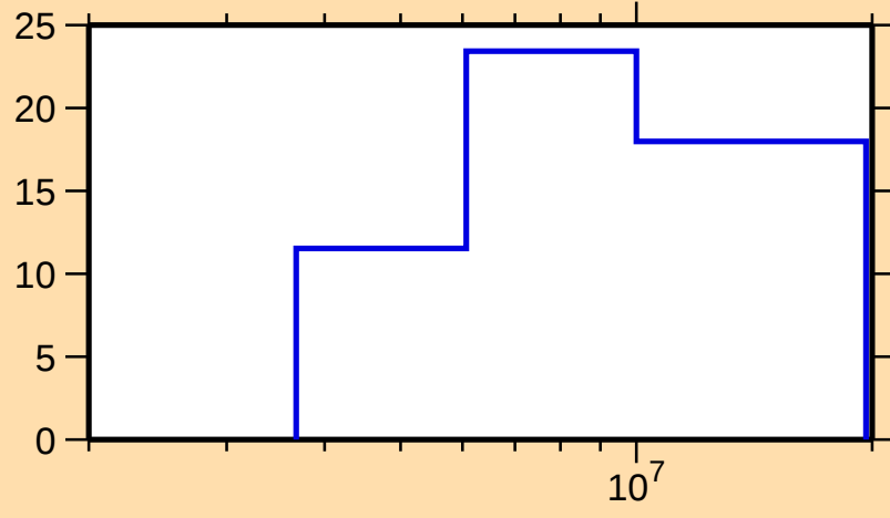
\Delta\sigma/\sigma vs. E for ^{141}\text{Ba}(n,\text{el.})
