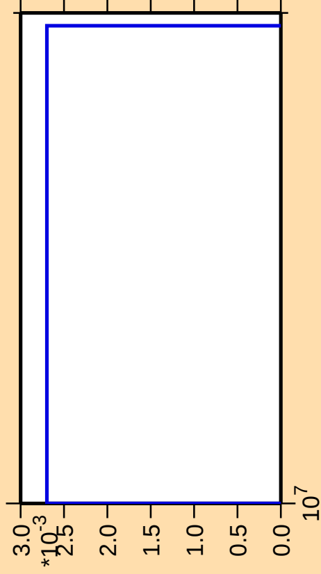
\Delta\sigma/\sigma vs. E for ^{141}\text{Ba}(n,\text{He3})
