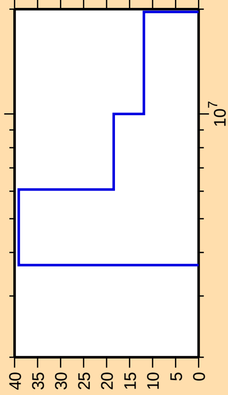
\Delta\sigma/\sigma vs. E for ^{141}\text{Ba}(n,2n)
