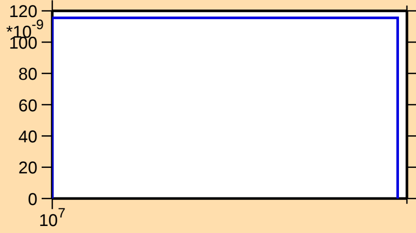
\sigma vs. E for ^{141}\text{Ba}(n,\text{nt})
