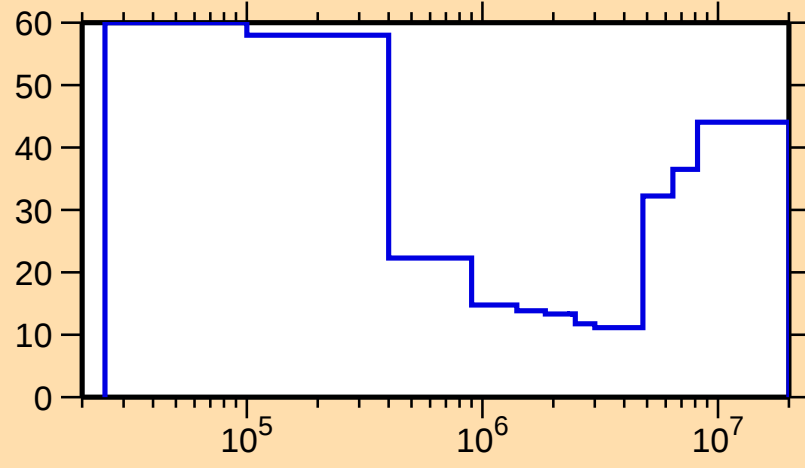
\Delta\sigma/\sigma vs. E for ^{141}\text{Ba}(n,\text{inel.})
