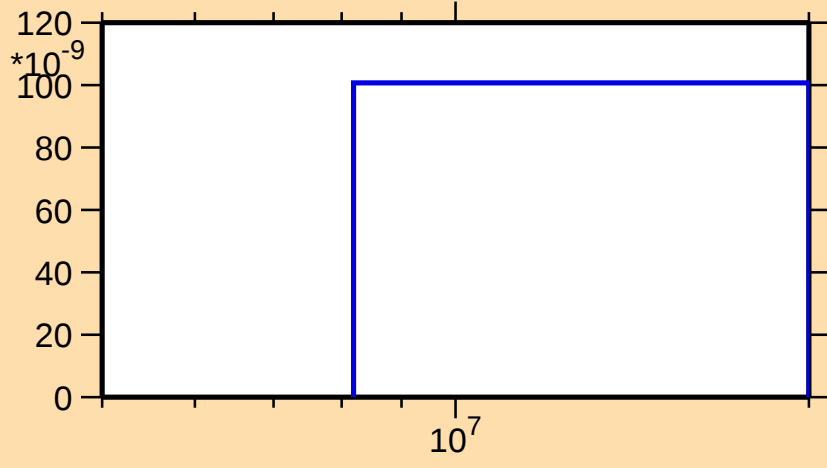
\sigma vs. E for ^{141}\text{Ba}(n,nt)
