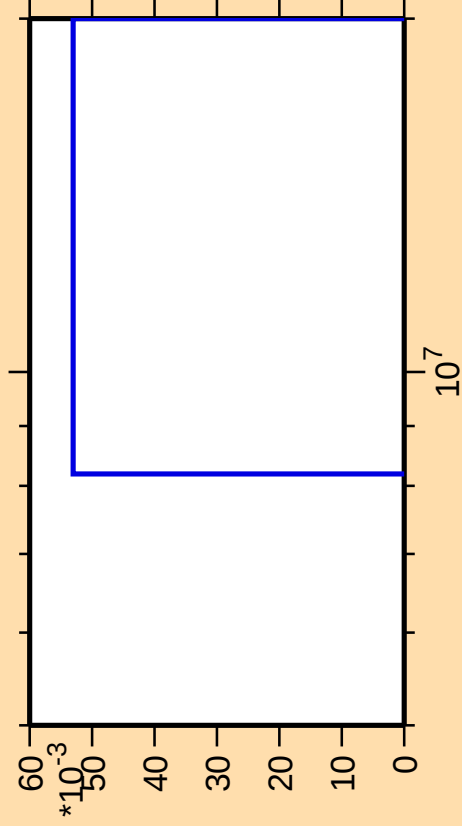
\Delta\sigma/\sigma vs. E for ^{141}\text{Ba}(n,3n\alpha)
