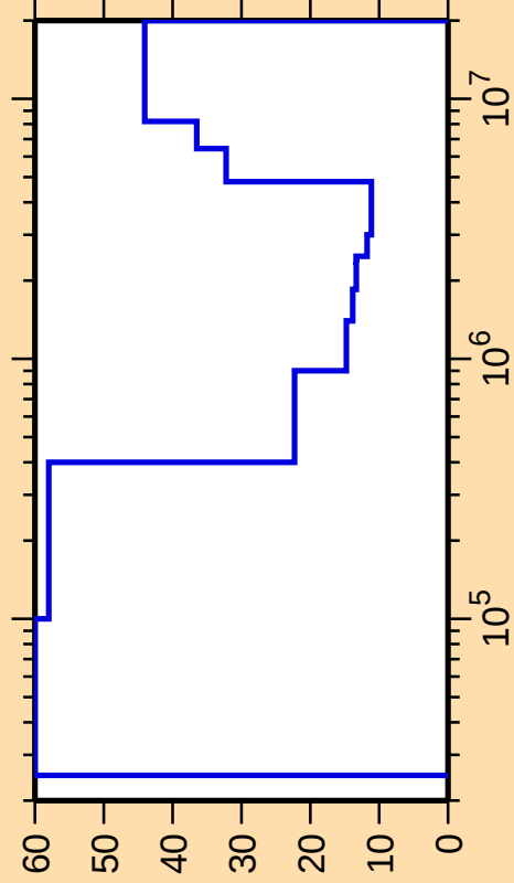
\Delta\sigma/\sigma vs. E for ^{141}\text{Ba}(n,\text{inel.})
