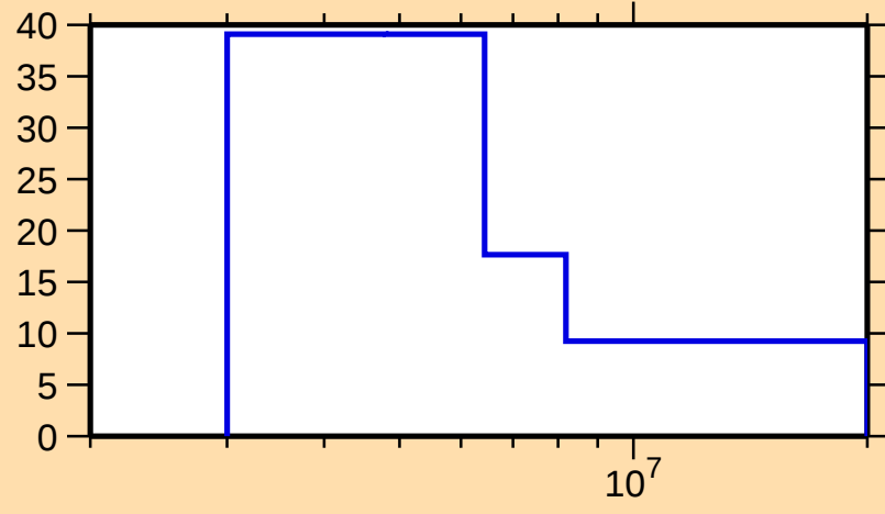
\Delta\sigma/\sigma vs. E for ^{141}\text{Ba}(n,2n)
