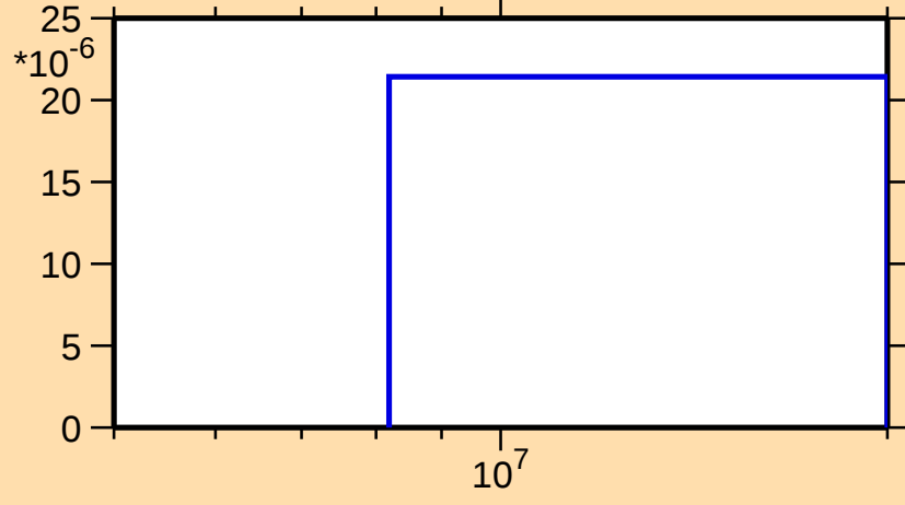
\sigma vs. E for ^{141}\text{Ba}(n,np)
