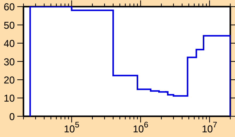
\Delta\sigma/\sigma vs. E for ^{141}\text{Ba}(n,\text{inel.})
