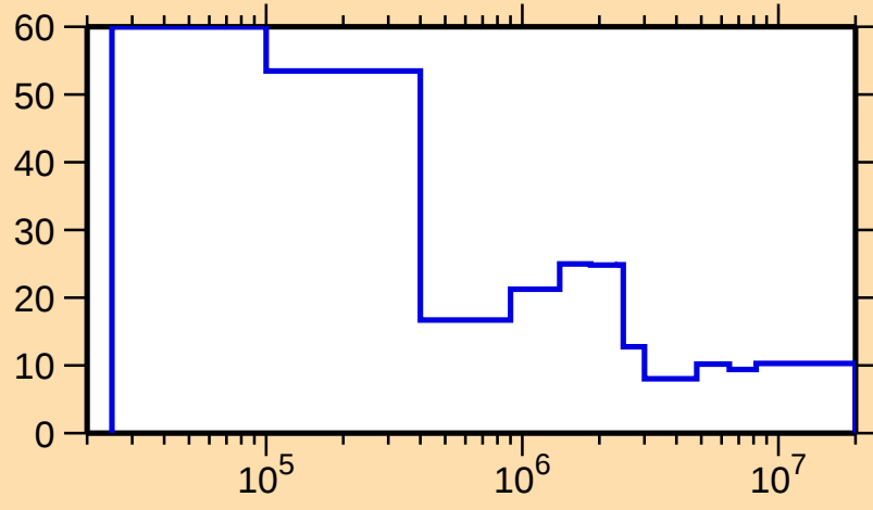
\Delta\sigma/\sigma vs. E for ^{141}\text{Ba}(n,\text{tot.})
