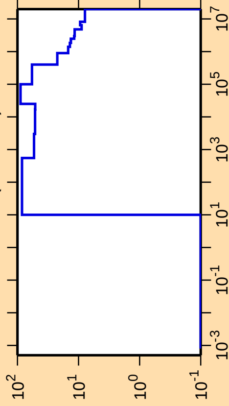
\Delta\sigma/\sigma vs. E for ^{141}\text{Ba}(n,\text{nonel.})
