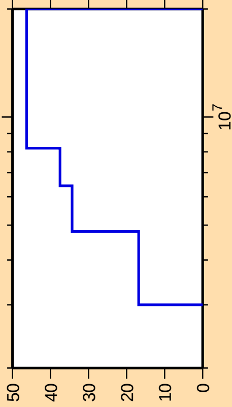
\Delta\sigma/\sigma vs. E for ^{141}\text{Ba}(n,n\text{cont.})
