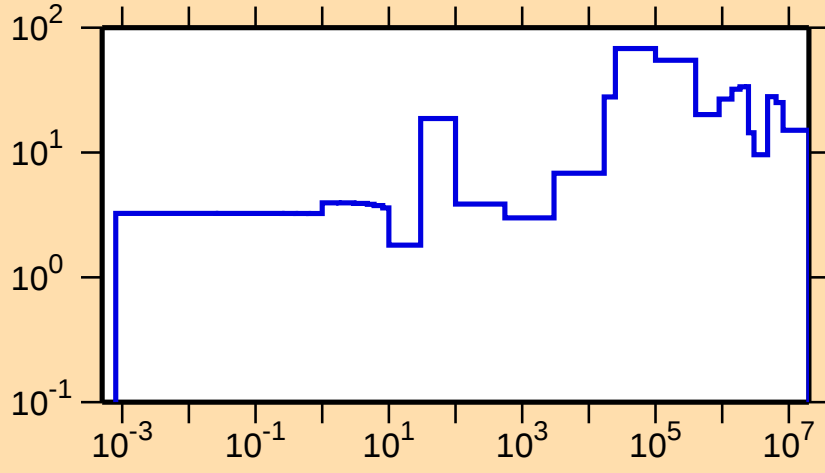
\Delta\sigma/\sigma vs. E for ^{141}\text{Ba}(n,\text{el.})
