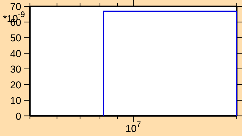
\sigma vs. E for ^{141}\text{Ba}(n,\text{nd})
