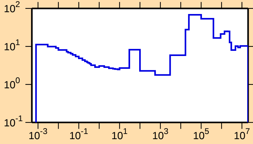
\Delta\sigma/\sigma vs. E for ^{141}\text{Ba}(n,\text{tot.})
