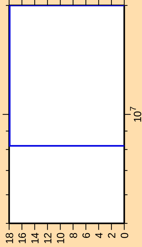
\Delta\sigma/\sigma vs. E for ^{141}\text{Ba}(n,3n)
