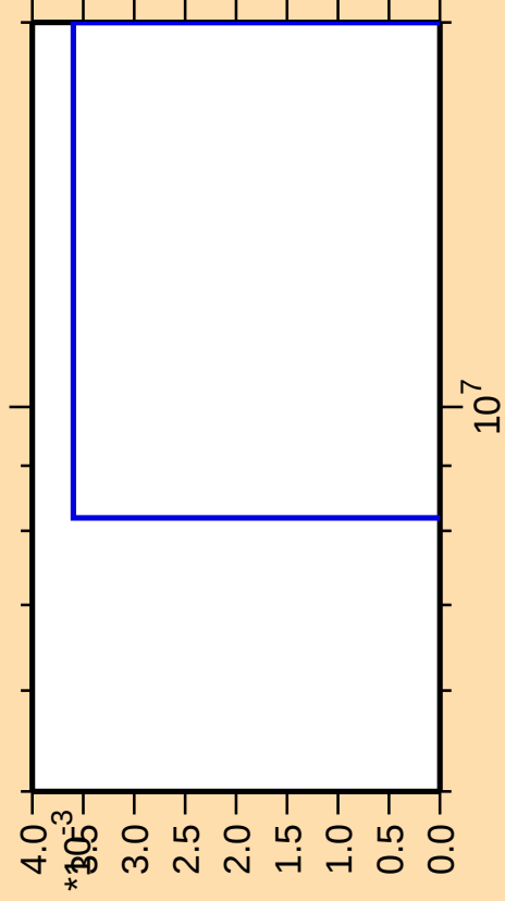
\Delta\sigma/\sigma vs. E for ^{141}\text{Ba}(n,\text{He}3)
