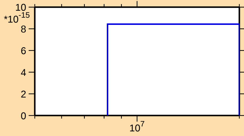
\sigma vs. E for ^{141}\text{Ba}(n,3n\alpha)
