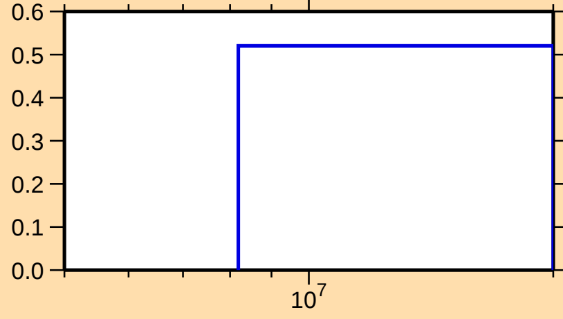
\sigma vs. E for ^{141}\text{Ba}(n,3n)
