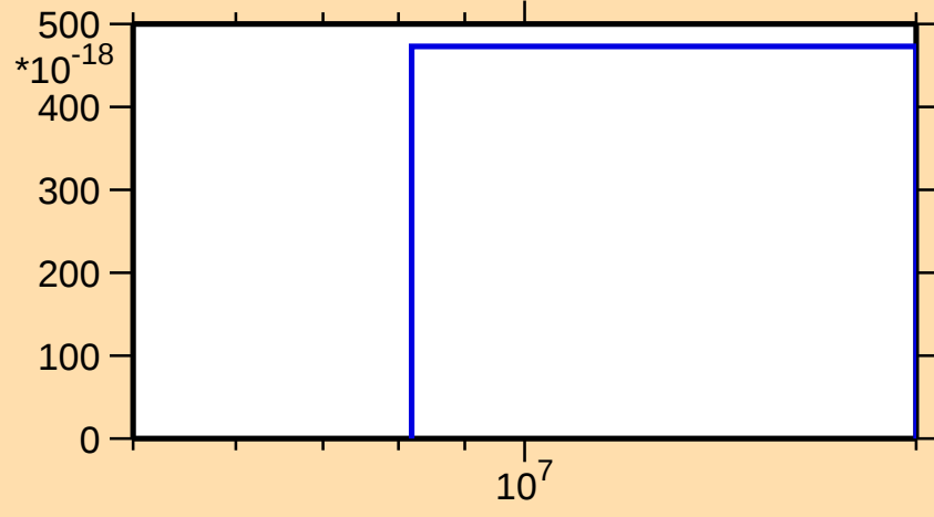
\sigma vs. E for ^{141}\text{Ba}(n,\text{He}3)
