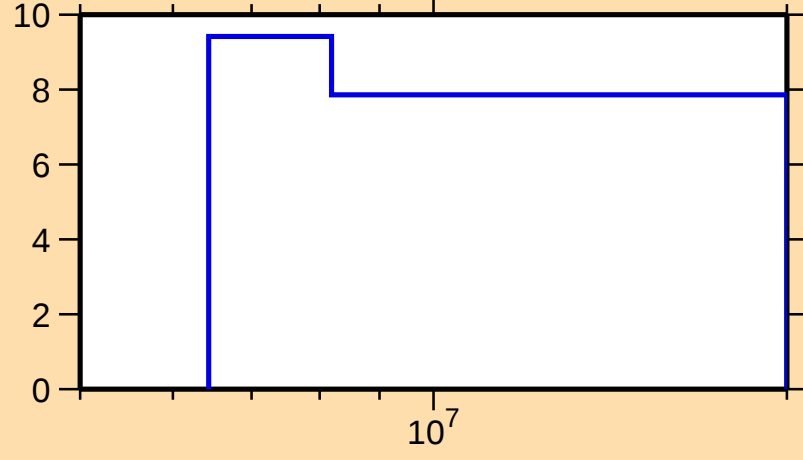
\Delta\sigma/\sigma vs. E for ^{141}\text{Ba}(n,\text{nonel.})
