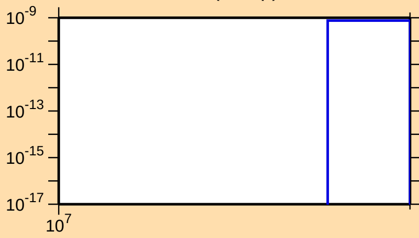
\sigma vs. E for ^{142}\text{Ba}(n,2np)
