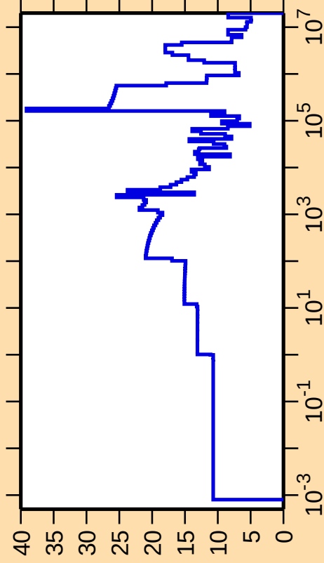
\Delta\sigma/\sigma vs. E for ^{142}\text{Ba}(n,\text{el.})
