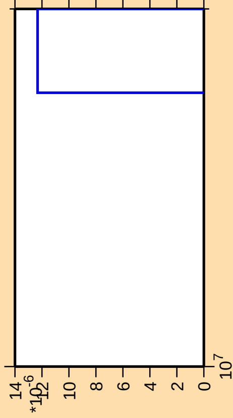
\Delta\sigma/\sigma vs. E for ^{142}\text{Ba}(\text{mt } 11)
