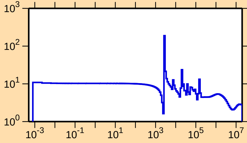
\sigma vs. E for ^{142}\text{Ba}(n,\text{el.})
