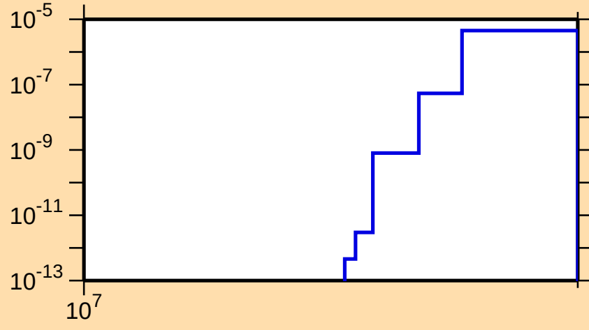
\sigma vs. E for ^{142}\text{Ba}(n,nt)
