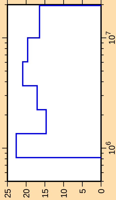
\Delta\sigma/\sigma vs. E for ^{142}\text{Ba}(n,n_3)
