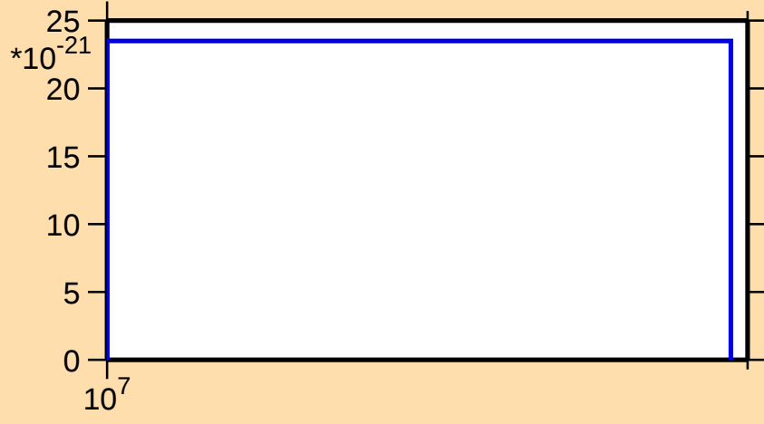
\sigma vs. E for ^{142}\text{Ba} (mt 11)
