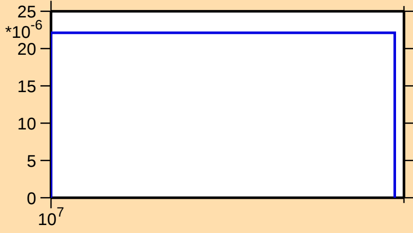
\sigma vs. E for ^{142}\text{Ba}(n,d)
