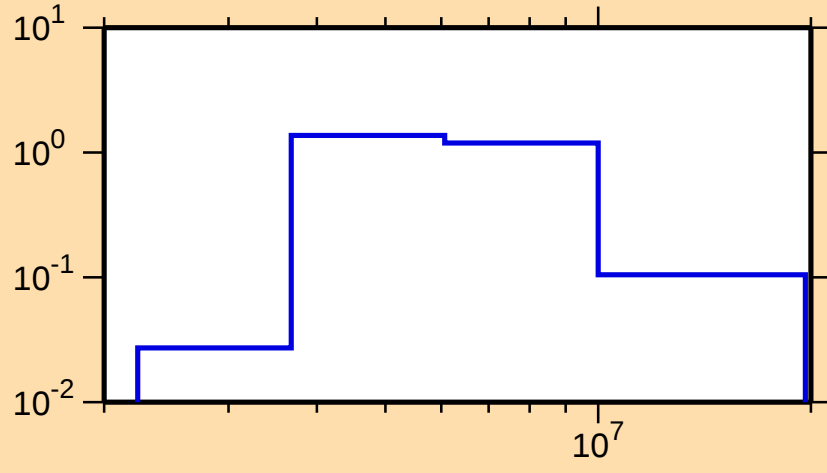
\sigma vs. E for ^{142}\text{Ba}(n,n\text{cont.})
