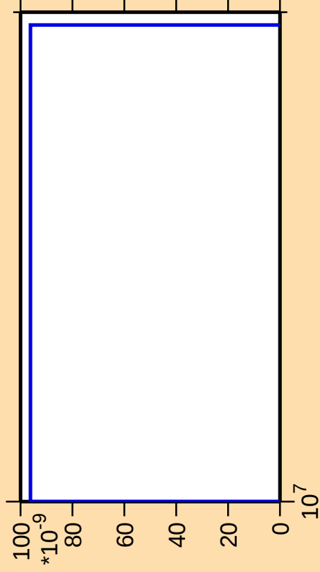
\Delta\sigma/\sigma vs. E for ^{142}\text{Ba} (mt 11)
