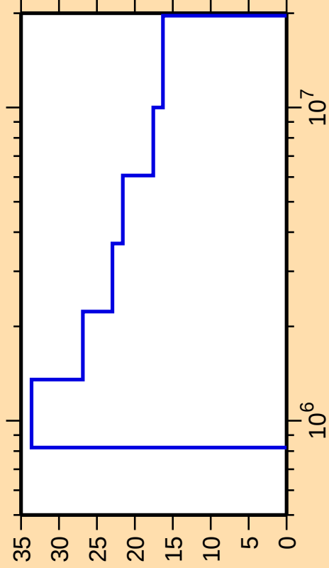
\Delta\sigma/\sigma vs. E for ^{142}\text{Ba}(n,n_2)
