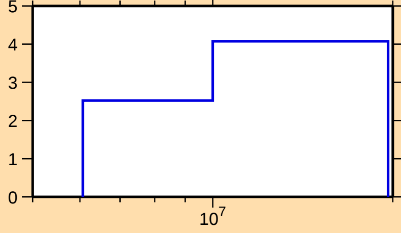
\Delta\sigma/\sigma vs. E for ^{142}\text{Ba}(n,\text{tot.})
