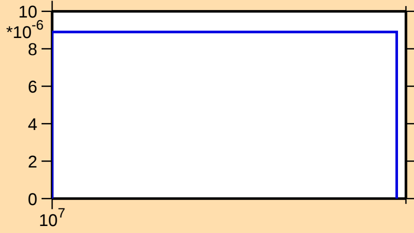
\sigma vs. E for ^{142}\text{Ba}(n,np)
