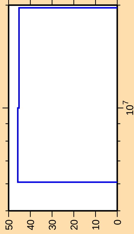
\Delta\sigma/\sigma vs. E for ^{142}\text{Ba}(n,p)
