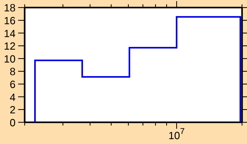
\Delta\sigma/\sigma vs. E for ^{142}\text{Ba}(n,\text{inel.})
