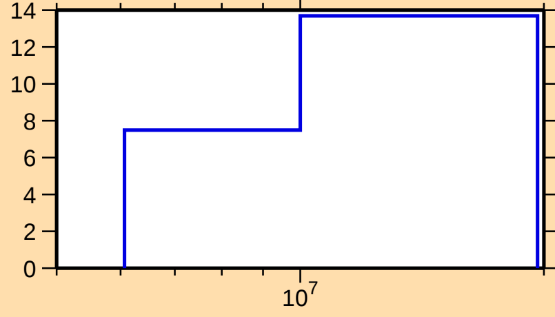
\Delta\sigma/\sigma vs. E for ^{142}\text{Ba}(n,2n)
