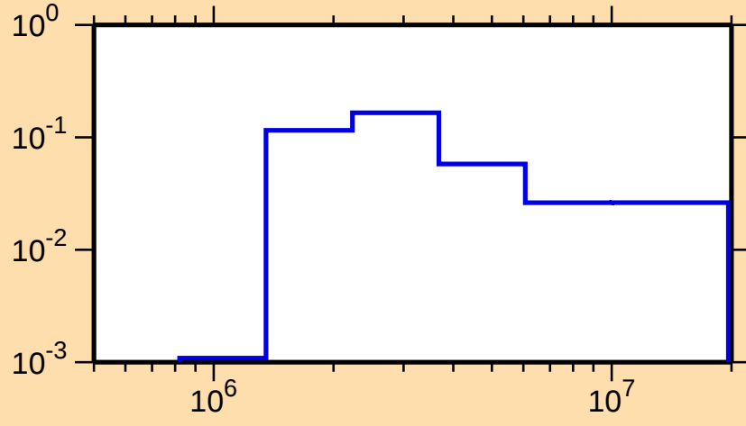
\sigma vs. E for ^{142}\text{Ba}(n,n_3)
