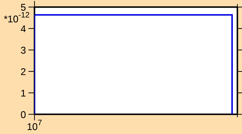
\sigma vs. E for ^{142}\text{Ba}(n,2np)
