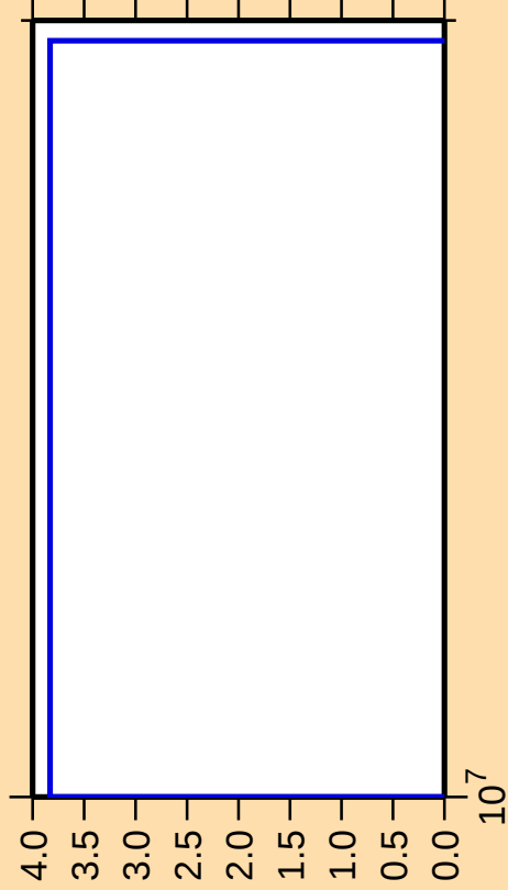
\Delta\sigma/\sigma vs. E for ^{142}\text{Ba}(n,2np)
