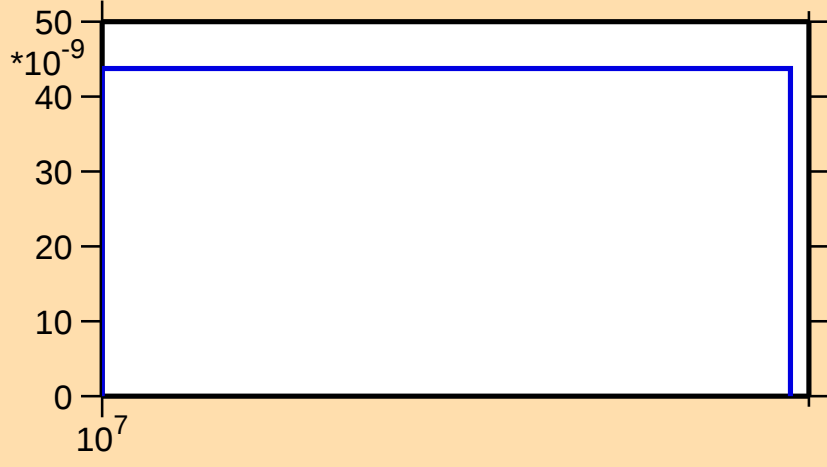
\sigma vs. E for ^{142}\text{Ba}(n,\text{nt})
