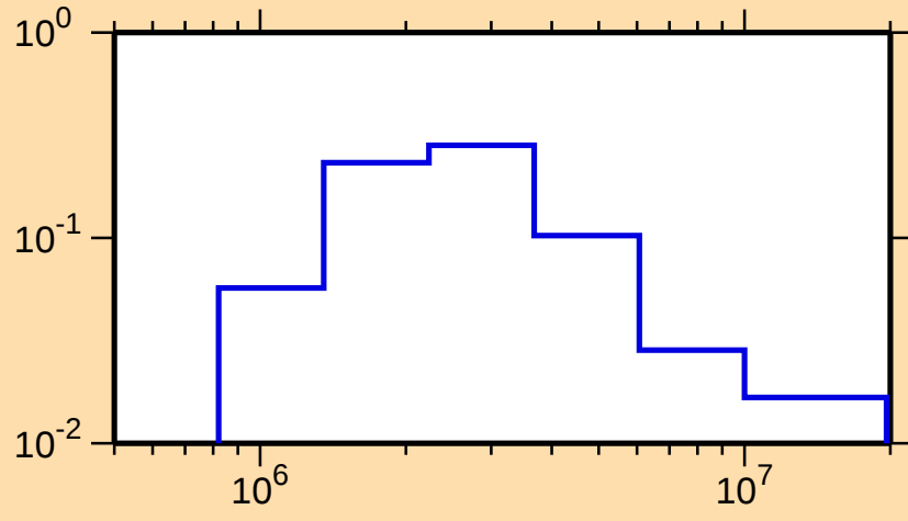
\sigma vs. E for ^{142}\text{Ba}(n,n_2)
