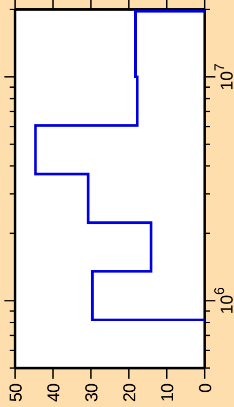
\Delta\sigma/\sigma vs. E for ^{142}\text{Ba}(n,n_4)
