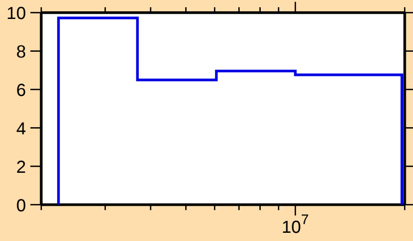
\Delta\sigma/\sigma vs. E for ^{142}\text{Ba}(n,n\text{onel.})
