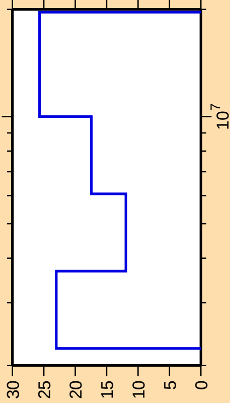
\Delta\sigma/\sigma vs. E for ^{142}\text{Ba}(n,\text{ncont.})
