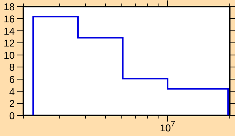
\Delta\sigma/\sigma vs. E for ^{142}\text{Ba}(n,\text{el.})
