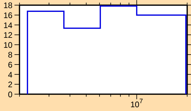
\Delta\sigma/\sigma vs. E for ^{142}\text{Ba}(n,n_1)
