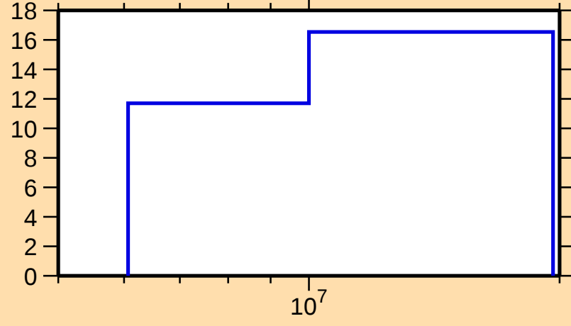
\Delta\sigma/\sigma vs. E for ^{142}\text{Ba}(n,\text{inel.})
