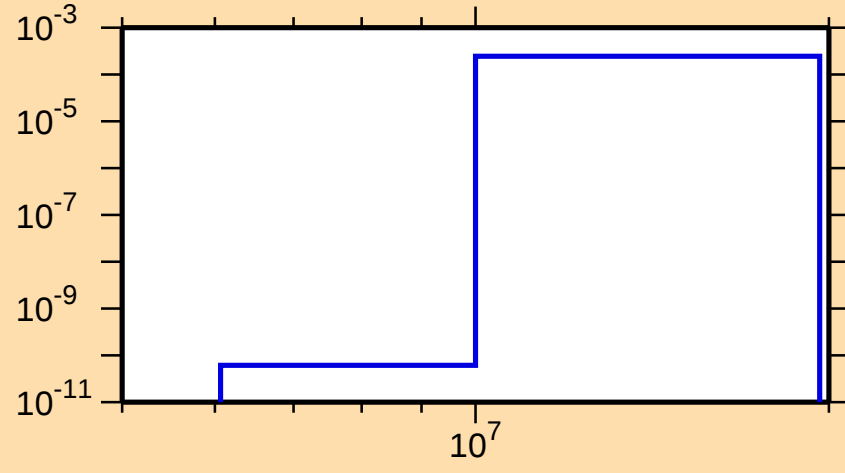
\sigma vs. E for ^{142}\text{Ba}(n,p)
