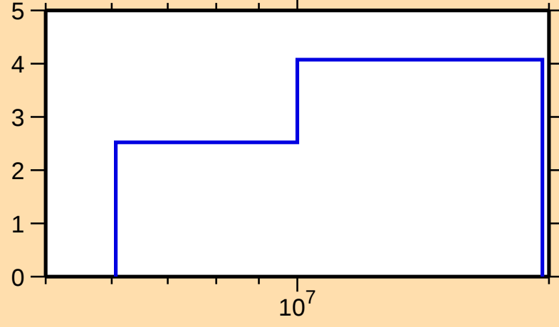
\Delta\sigma/\sigma vs. E for ^{142}\text{Ba}(n,\text{tot.})
