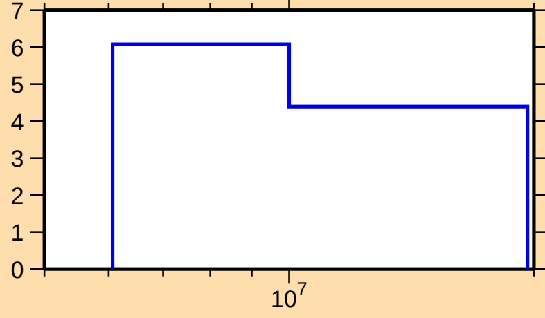
\Delta\sigma/\sigma vs. E for ^{142}\text{Ba}(n,\text{el.})
