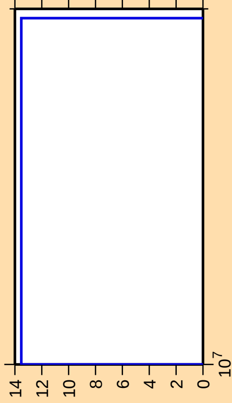
\Delta\sigma/\sigma vs. E for ^{142}\text{Ba}(n,3n)
