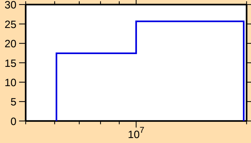
\Delta\sigma/\sigma vs. E for ^{142}\text{Ba}(n,n\text{cont.})
