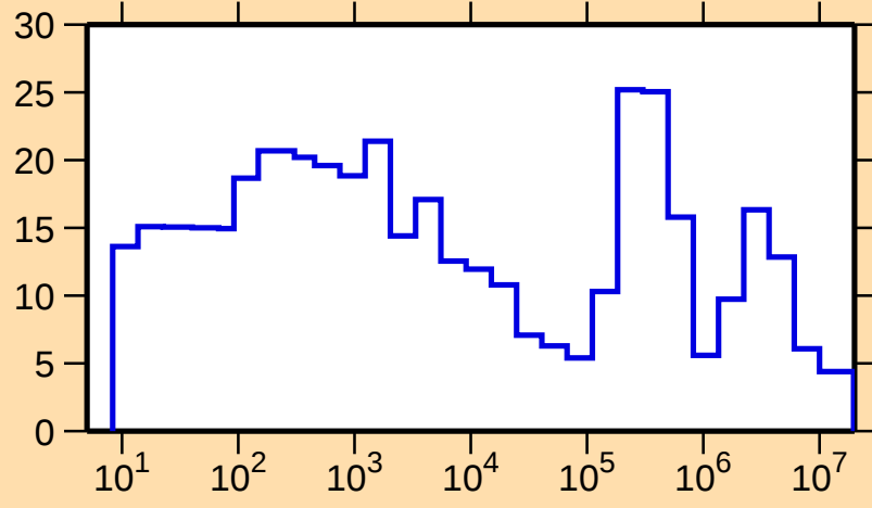
\Delta\sigma/\sigma vs. E for ^{142}\text{Ba}(n,\text{el.})
