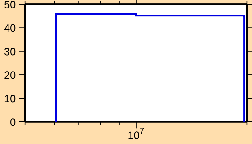
\Delta\sigma/\sigma vs. E for ^{142}\text{Ba}(n,p)
