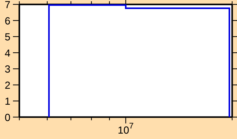
\Delta\sigma/\sigma vs. E for ^{142}\text{Ba}(n,\text{nonel.})
