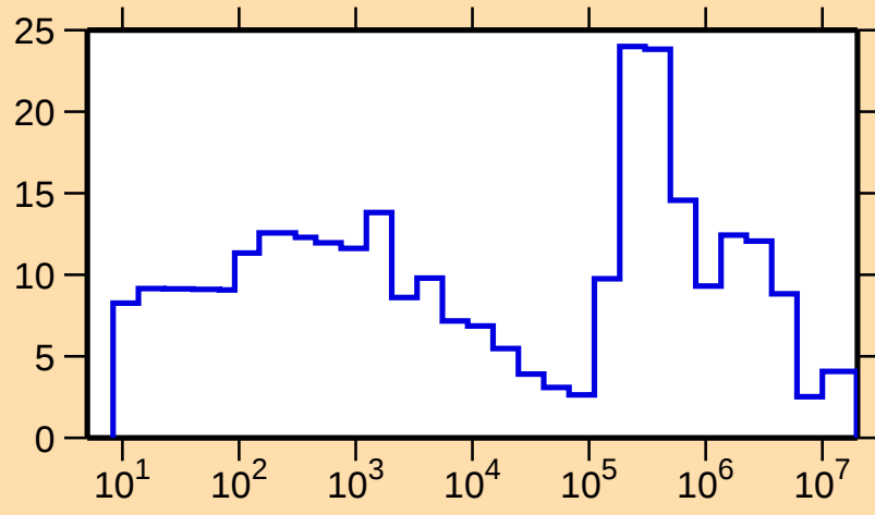
\Delta\sigma/\sigma vs. E for ^{142}\text{Ba}(n,\text{tot.})
