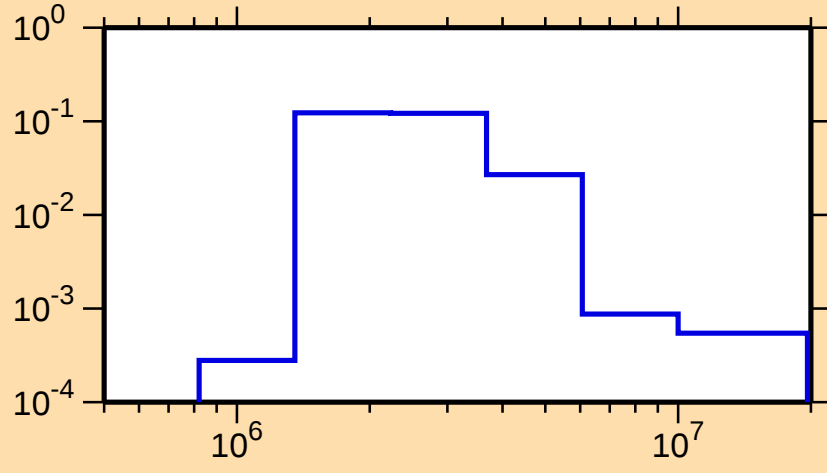
\sigma vs. E for ^{142}\text{Ba}(n,n_4)
