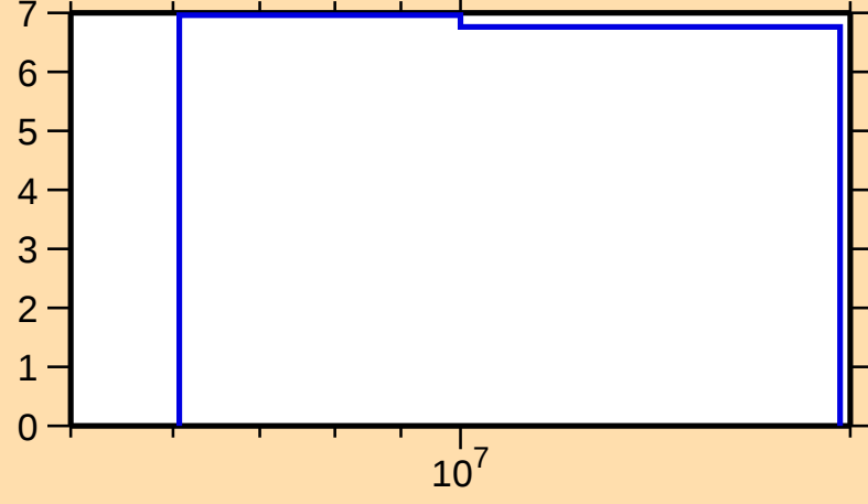
\Delta\sigma/\sigma vs. E for ^{142}\text{Ba}(n,\text{nonel.})
