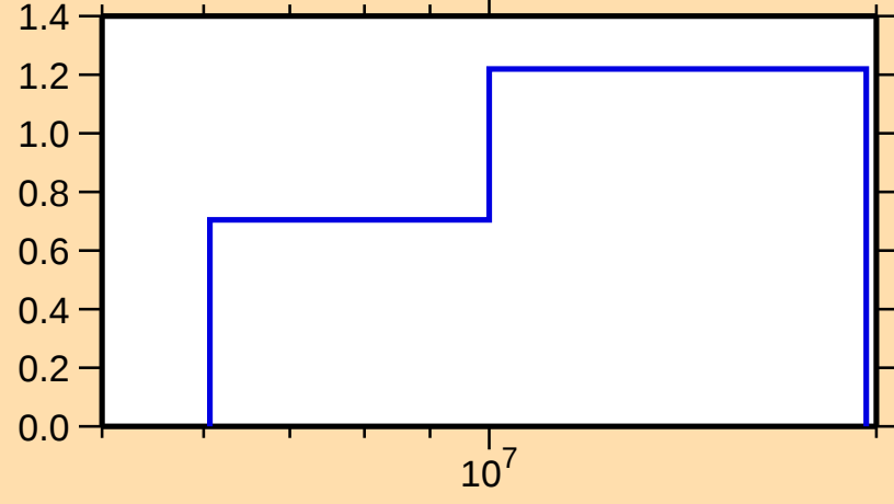
\sigma vs. E for ^{142}\text{Ba}(n,2n)
