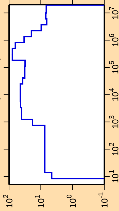
\Delta\sigma/\sigma vs. E for ^{142}\text{Ba}(n,\text{nonel.})
