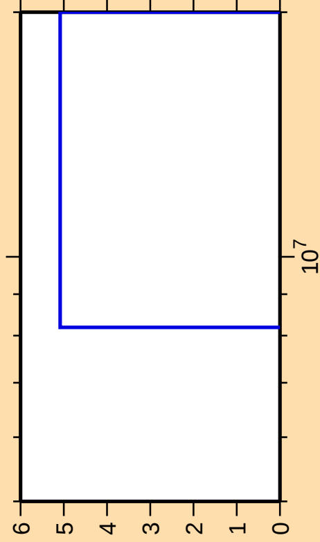
\Delta\sigma/\sigma vs. E for ^{142}\text{Ba}(n,2np)
