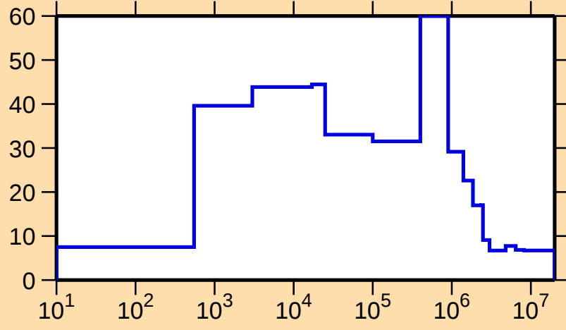
\Delta\sigma/\sigma vs. E for ^{142}\text{Ba}(n,\text{nonel.})
