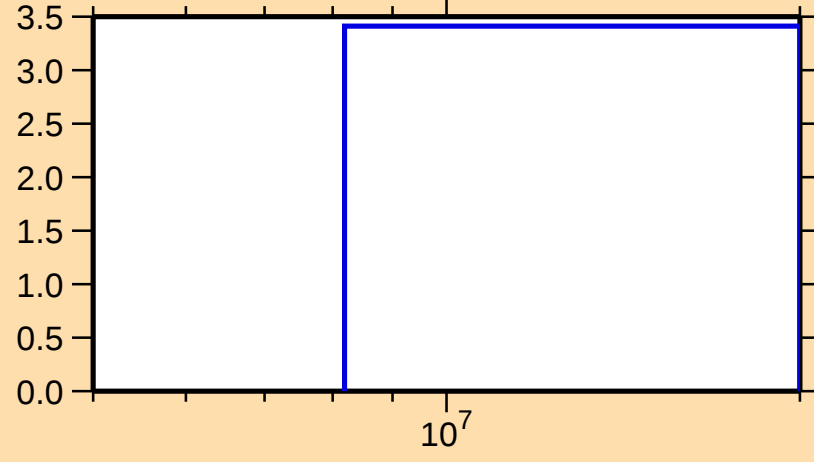
\Delta\sigma/\sigma vs. E for ^{142}\text{Ba}(n,\text{tot.})
