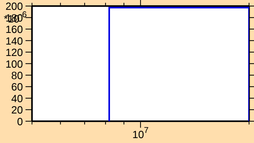
\sigma vs. E for ^{142}\text{Ba}(n,p)
