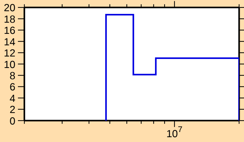
\Delta\sigma/\sigma vs. E for ^{142}\text{Ba}(n,2n)
