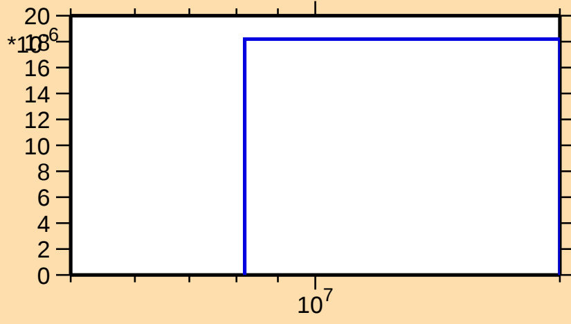
\sigma vs. E for ^{142}\text{Ba}(n,t)
