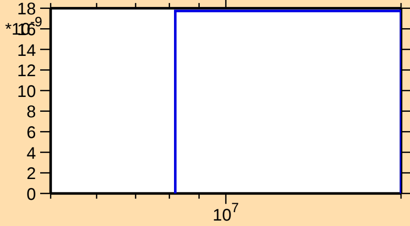
\sigma vs. E for ^{142}\text{Ba}(n,2n\alpha)
