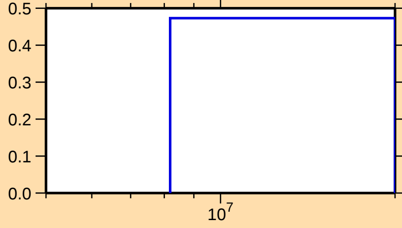
\sigma vs. E for ^{142}\text{Ba}(n,3n)
