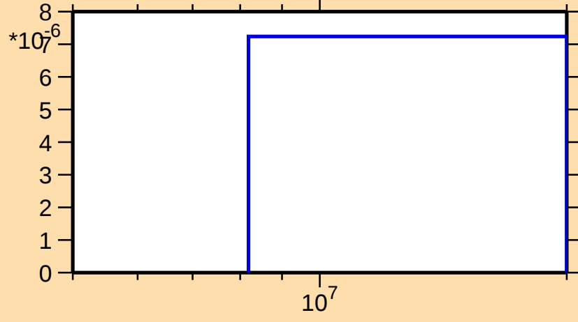
\sigma vs. E for ^{142}\text{Ba}(n,np)
