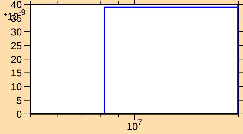
\sigma vs. E for ^{142}\text{Ba}(n,nt)
