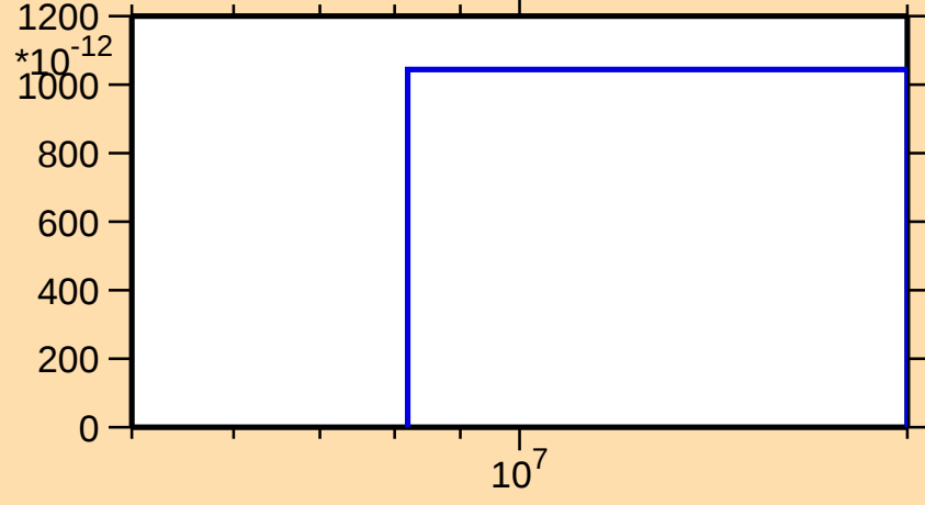
\sigma vs. E for ^{142}\text{Ba}(n,\text{nd})
