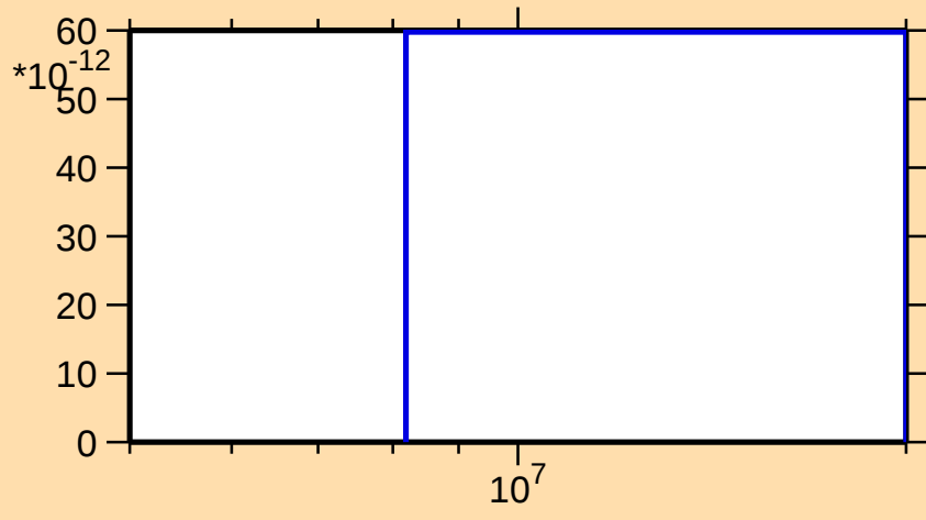
\sigma vs. E for ^{142}\text{Ba}(n,3n\alpha)
