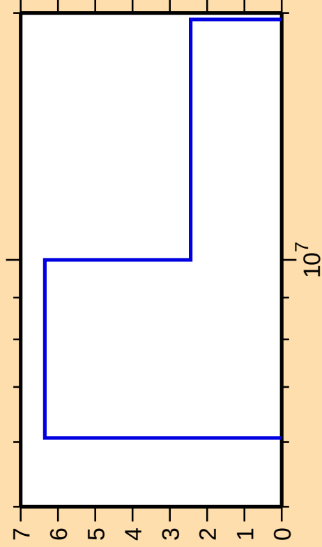
\Delta\sigma/\sigma vs. E for ^{269}
