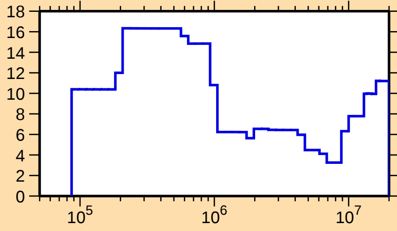
\Delta\sigma/\sigma vs. E for ^{271}\text{I}
