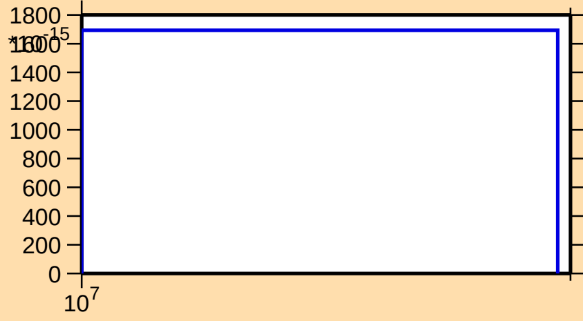
\sigma vs. E for ^{191}\text{Bi}(\text{mt } 34)
