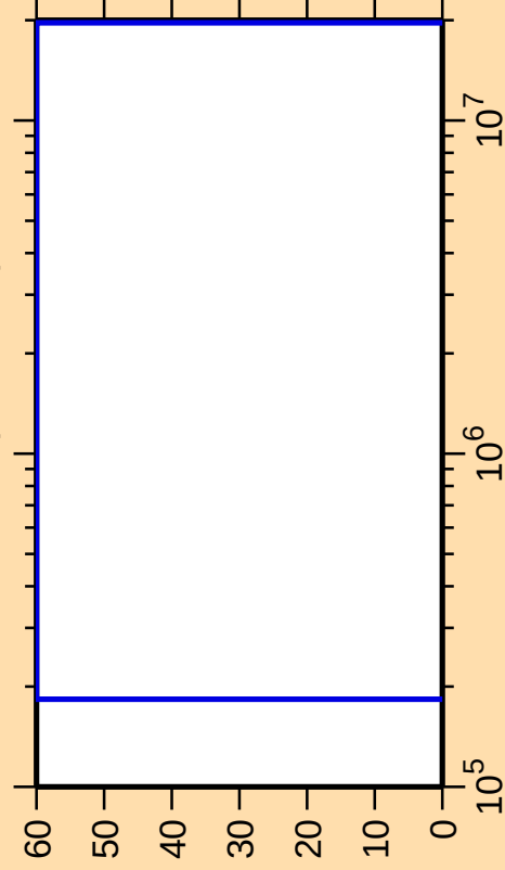
\Delta\sigma/\sigma vs. E for ^{191}\text{Bi}(n,n\text{cont.})
