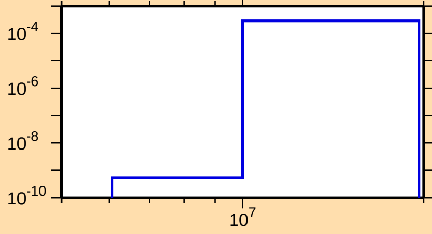
\sigma vs. E for ^{191}\text{Bi}(n,t)
