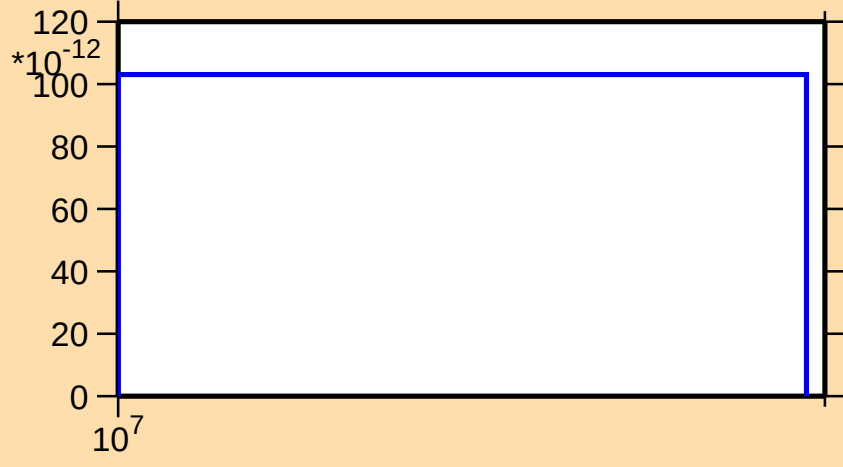
\sigma vs. E for ^{191}\text{Bi}(n,\text{nt})
