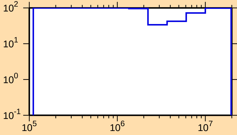
\Delta\sigma/\sigma vs. E for ^{191}\text{Bi}(n,n_1)
