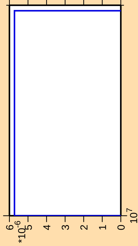
\Delta\sigma/\sigma vs. E for ^{191}\text{Bi} (mt 42)
