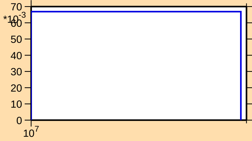
\sigma vs. E for ^{191}\text{Bi}(n,2n)
