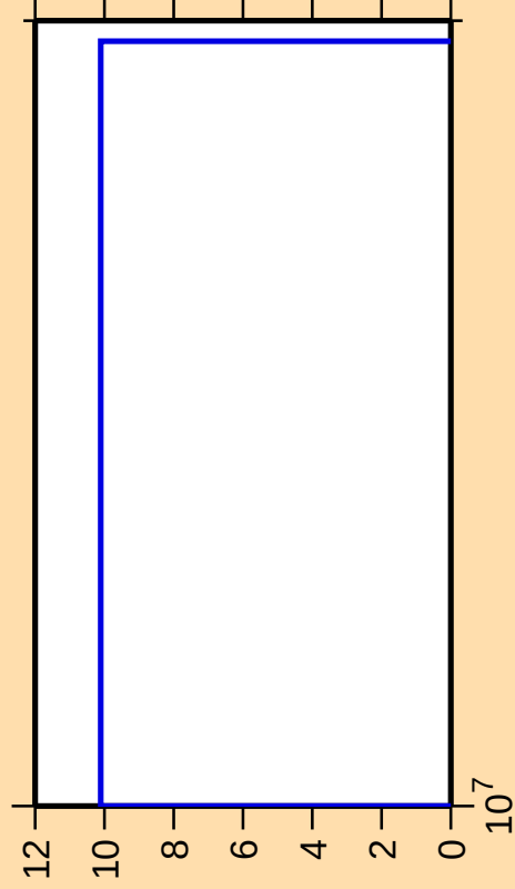
\Delta\sigma/\sigma vs. E for ^{191}\text{Bi}(\text{mt } 34)
