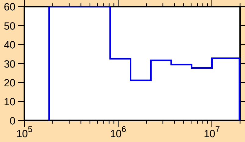
\Delta\sigma/\sigma vs. E for ^{191}\text{Bi}(n,n\text{onel.})
