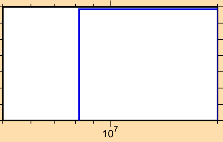
\sigma vs. E for ^{194}\text{Bi}(n,\text{pd})
