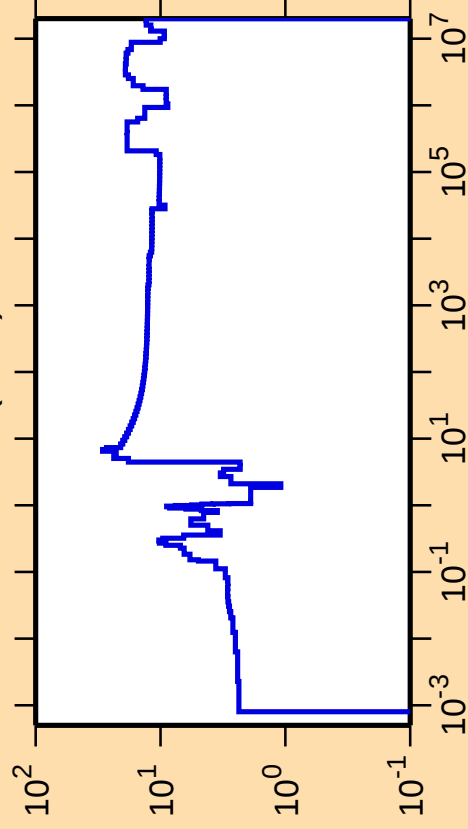
\Delta\sigma/\sigma vs. E for ^{194}\text{Bi}(n,\text{el.})
