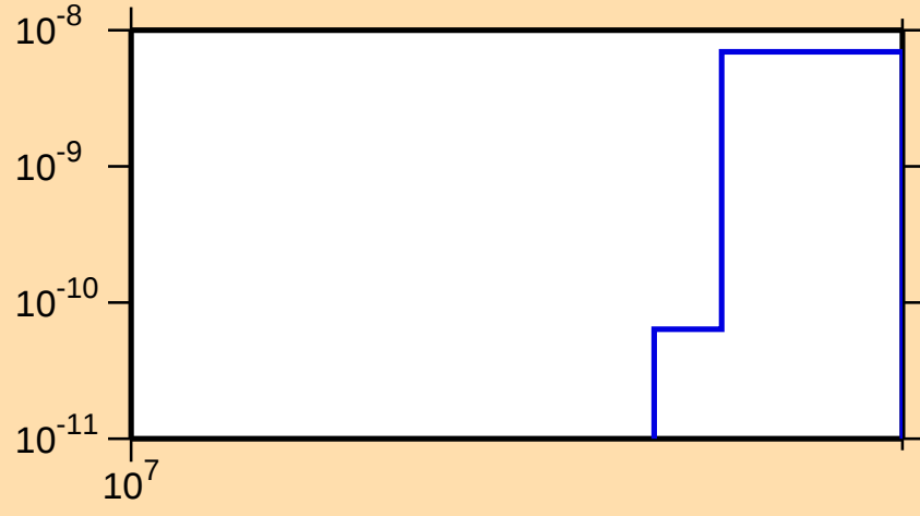
\sigma vs. E for ^{194}\text{Bi}(n,\text{nt})
