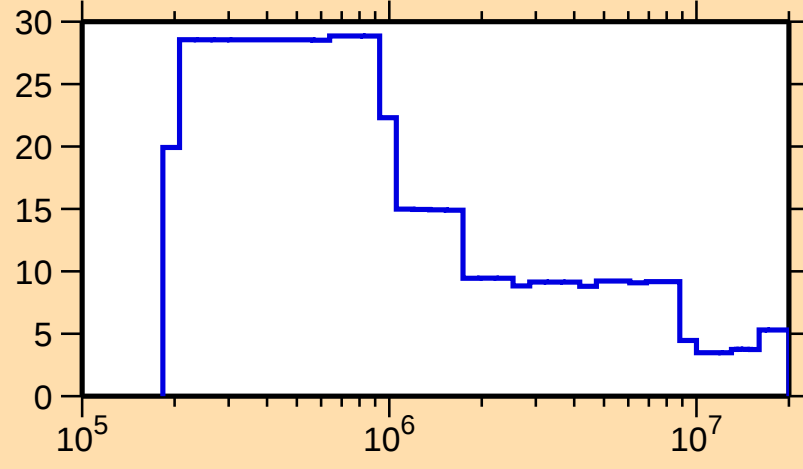
\Delta\sigma/\sigma vs. E for ^{194}\text{Bi}(n,\text{tot.})
