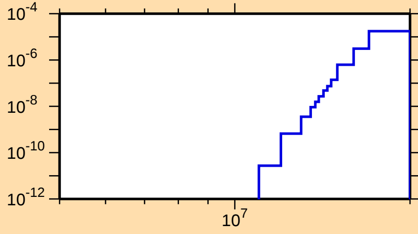
\sigma vs. E for ^{194}\text{Bi}(n,\text{nd})
