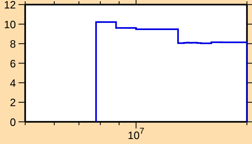
\Delta\sigma/\sigma vs. E for ^{194}\text{Bi}(n,\text{nonel.})
