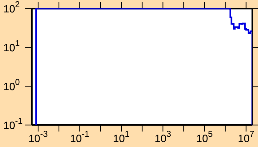
\Delta\sigma/\sigma vs. E for ^{194}\text{Bi}(n,p)
