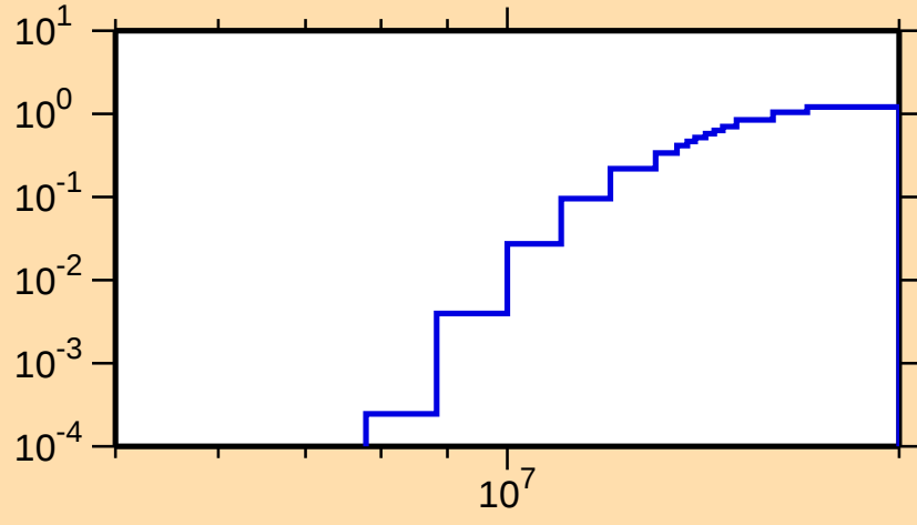
\sigma vs. E for ^{194}\text{Bi}(n,2n)
