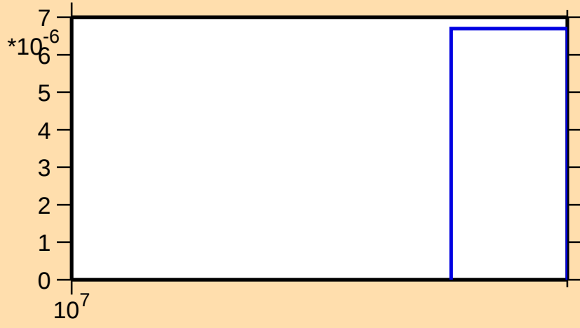
\sigma vs. E for ^{194}\text{Bi}(n,3n)
