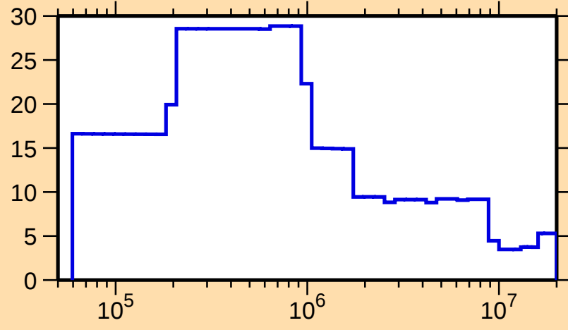
\Delta\sigma/\sigma vs. E for ^{194}\text{Bi}(n,\text{tot.})
