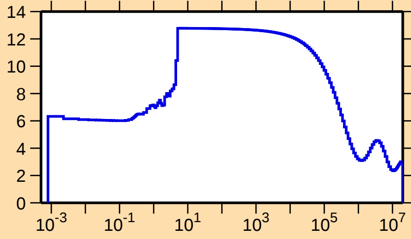
\sigma vs. E for ^{194}\text{Bi}(n,\text{el.})
