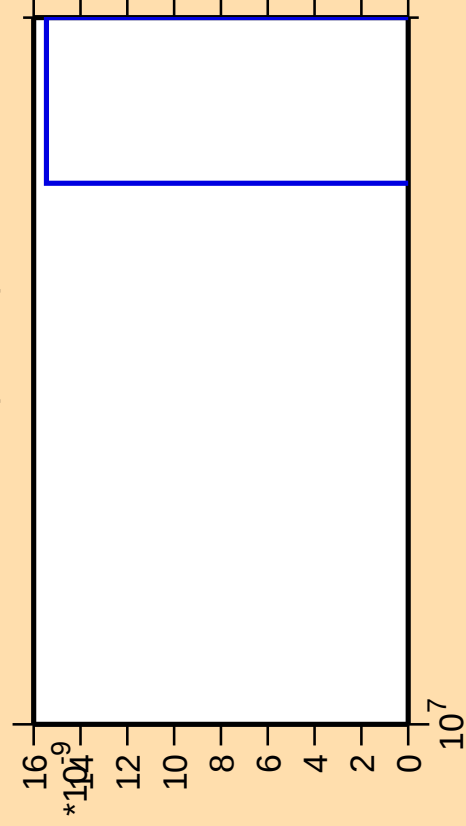
\Delta\sigma/\sigma vs. E for ^{194}\text{Bi}(\text{mt } 42)
