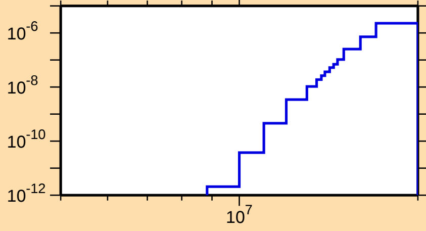
\sigma vs. E for ^{194}\text{Bi}(\text{mt 45})
