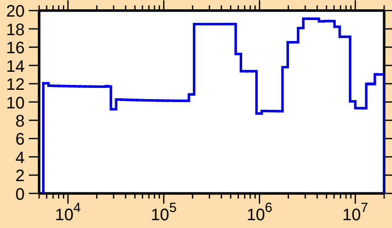
\Delta\sigma/\sigma vs. E for ^{194}\text{Bi}(n,\text{el.})
