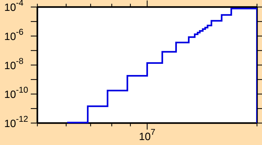
\sigma vs. E for ^{194}\text{Bi}(n,\text{He3})
