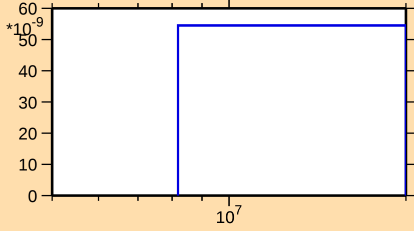
\sigma vs. E for ^{194}\text{Bi}(n,3n)
