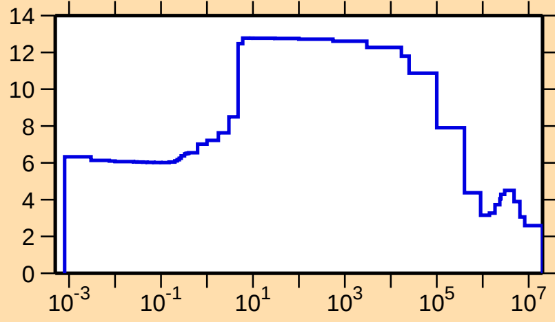
\sigma vs. E for ^{194}\text{Bi}(n,\text{el.})
