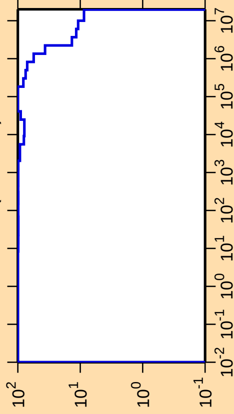
\Delta\sigma/\sigma vs. E for ^{194}\text{Bi}(n,\text{nonel.})
