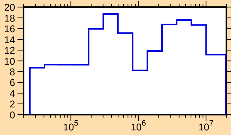
\Delta\sigma/\sigma vs. E for ^{194}\text{Bi}(n,\text{el.})
