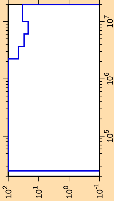
\Delta\sigma/\sigma vs. E for ^{194}\text{Bi}(n,n_{\text{cont.}})
