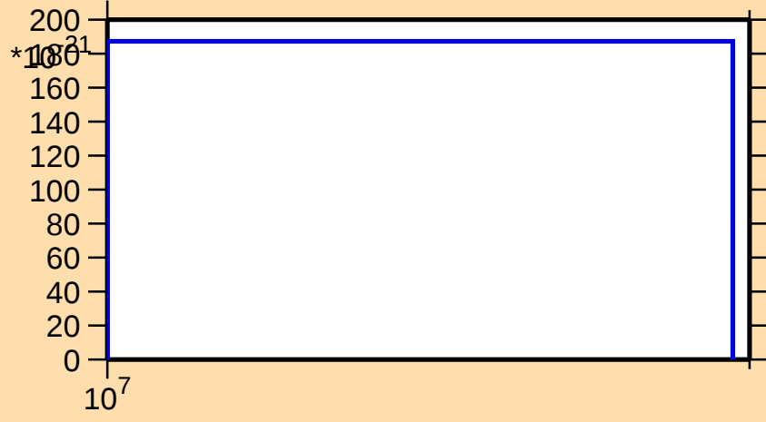
\sigma vs. E for ^{195}\text{Bi} (mt 42)
