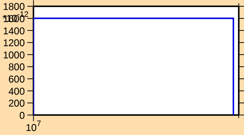
\sigma vs. E for ^{195}\text{Bi}(n,\text{nt})
