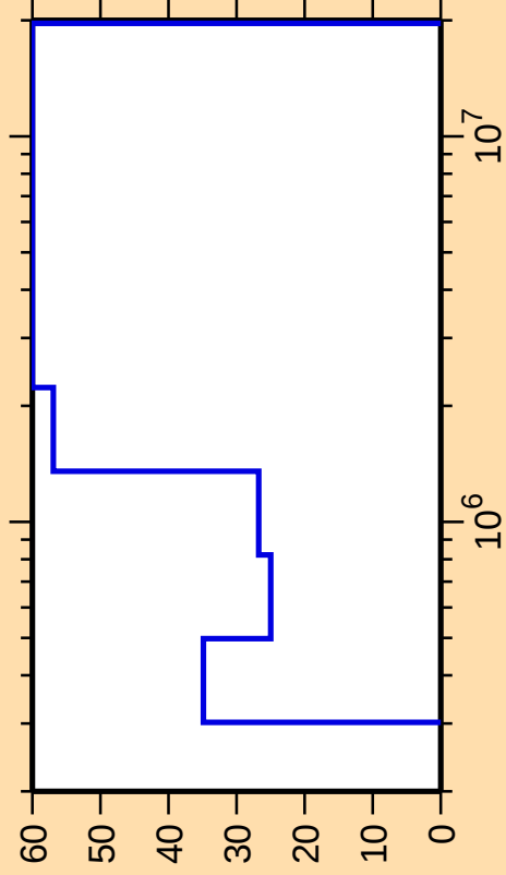
\Delta\sigma/\sigma vs. E for ^{195}\text{Bi}(n,\gamma)
