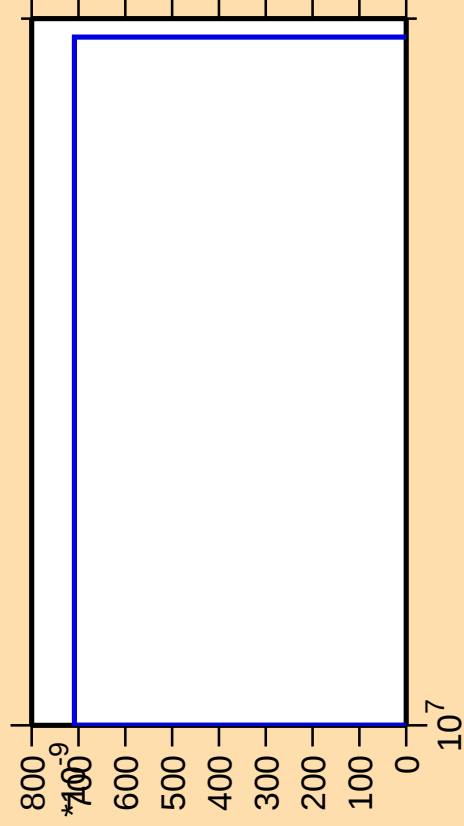
\Delta\sigma/\sigma vs. E for ^{195}\text{Bi} (mt 42)
