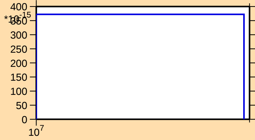
\sigma vs. E for ^{195}\text{Bi}(\text{mt } 34)
