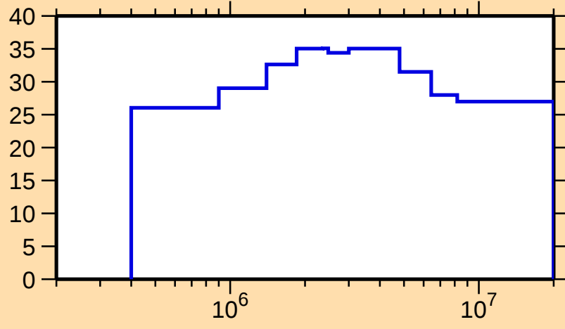
\Delta\sigma/\sigma vs. E for ^{195}\text{Bi}(n,n\text{onel.})
