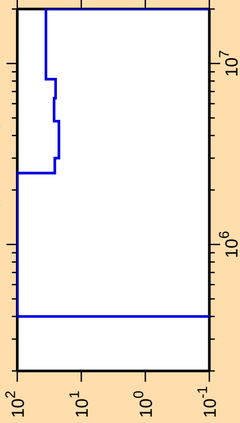
\Delta\sigma/\sigma vs. E for ^{195}\text{Bi}(n,n\text{cont.})
