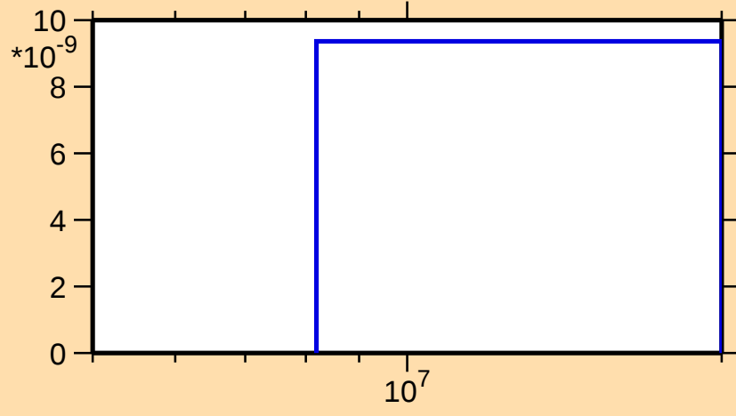
\sigma vs. E for ^{195}\text{Bi}(n,\text{pd})
