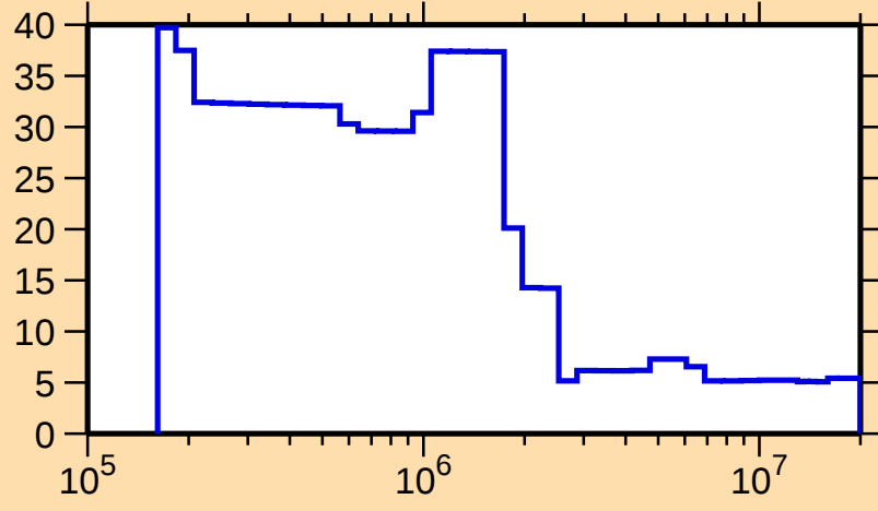
\Delta\sigma/\sigma vs. E for ^{198}\text{Bi}(n,\text{nonel.})
