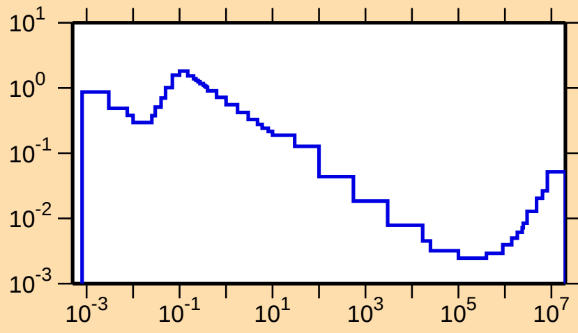
\sigma vs. E for ^{198}\text{Bi}(n,p)
