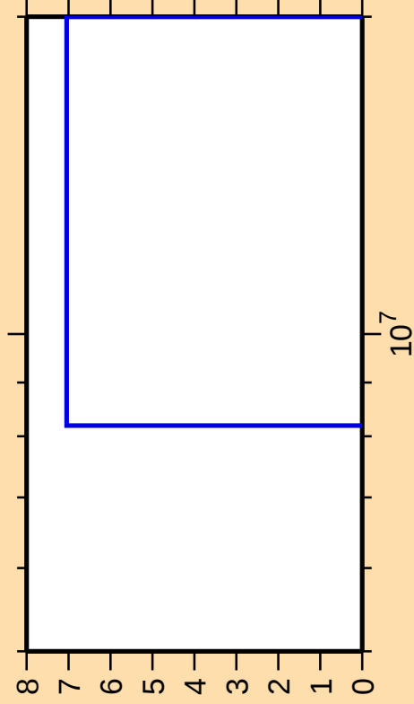
\Delta\sigma/\sigma vs. E for ^{198}\text{Bi}(n,\text{pt})
