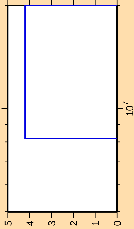
\Delta\sigma/\sigma vs. E for ^{198}\text{Bi}(\text{mt } 34)
