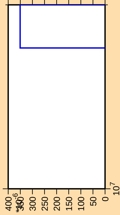
\Delta\sigma/\sigma vs. E for ^{198}\text{Bi}(\text{mt } 42)
