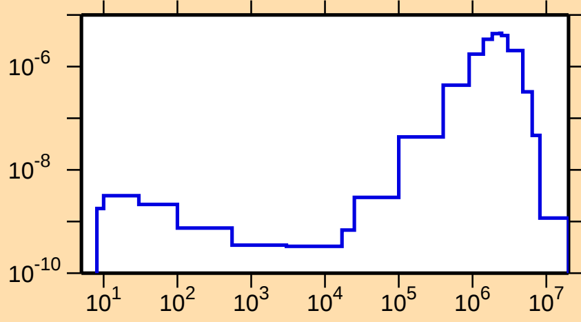
\sigma vs. E for ^{198}\text{Bi}(n,n_3)
