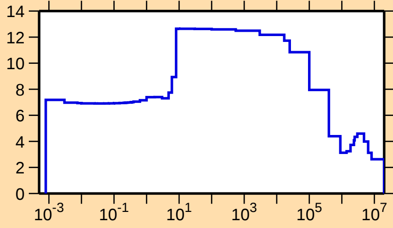
\sigma vs. E for ^{198}\text{Bi}(n,\text{el.})
