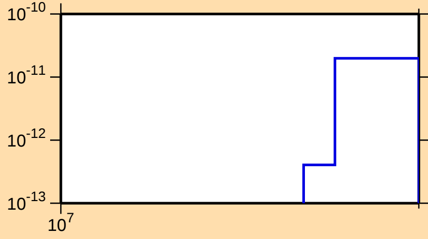
\sigma vs. E for ^{200}\text{Bi}(\text{mt } 34)
