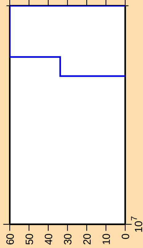
\Delta\sigma/\sigma vs. E for ^{200}\text{Bi}(\text{mt } 45)
