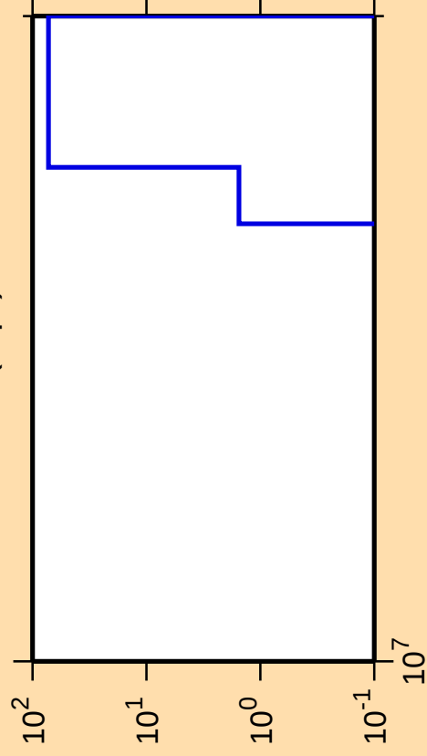
\Delta\sigma/\sigma vs. E for ^{200}\text{Bi}(n,\text{pt})
