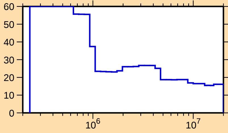
\Delta\sigma/\sigma vs. E for ^{200}\text{Bi}(n,n\text{onel.})
