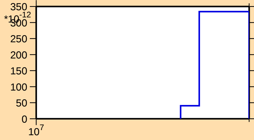
\sigma vs. E for ^{200}\text{Bi}(\text{mt } 45)
