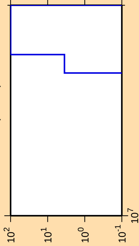
\Delta\sigma/\sigma vs. E for ^{200}\text{Bi}(\text{mt } 34)
