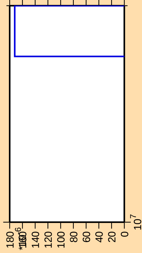
\Delta\sigma/\sigma vs. E for ^{200}\text{Bi}(\text{mt } 42)
