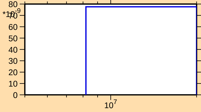
\sigma vs. E for ^{207}\text{Bi}(n,\text{nd})
