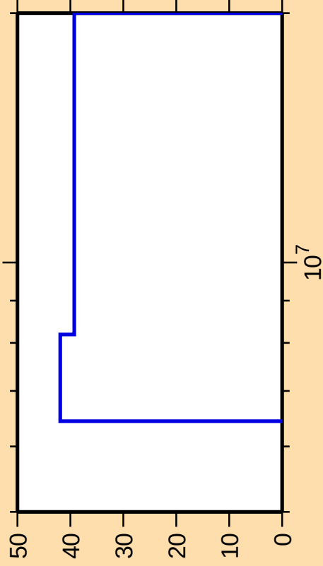
\Delta\sigma/\sigma vs. E for ^{207}\text{Bi}(n,n_1)
