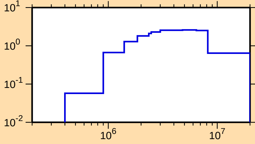
\sigma vs. E for ^{207}\text{Bi}(n,\text{inel.})
