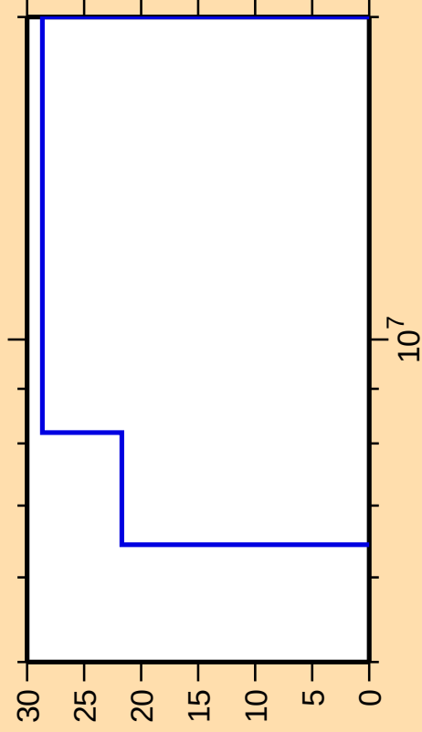
\Delta\sigma/\sigma vs. E for ^{207}\text{Bi}(n,n\text{cont.})
