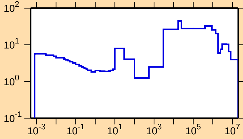
\Delta\sigma/\sigma vs. E for ^{207}\text{Bi}(n,\text{tot.})
