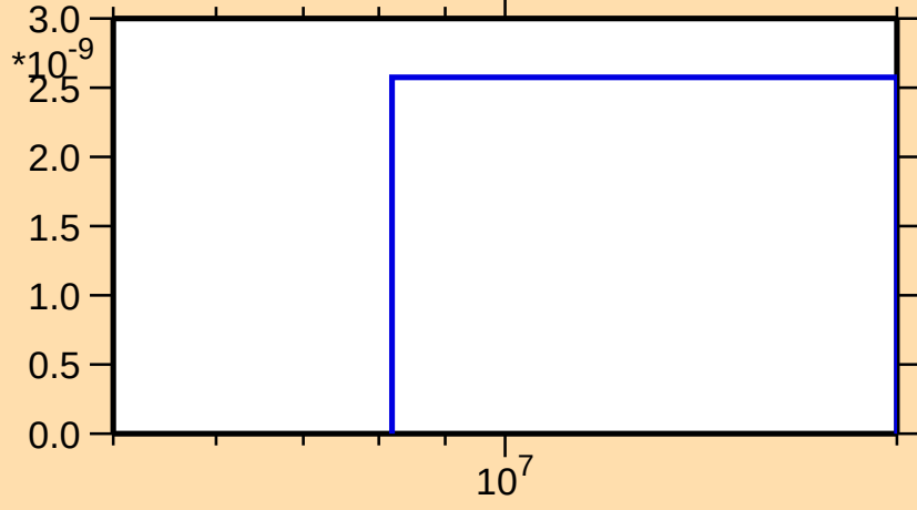
\sigma vs. E for ^{207}\text{Bi}(n,2n\alpha)
