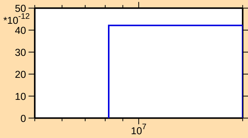
\sigma vs. E for ^{207}\text{Bi}(n,\text{He3})
