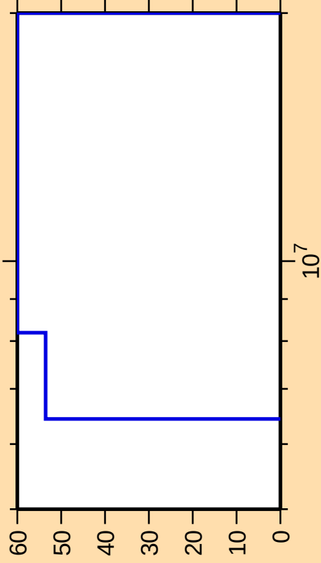
\Delta\sigma/\sigma vs. E for ^{207}\text{Bi}(n,\gamma)
