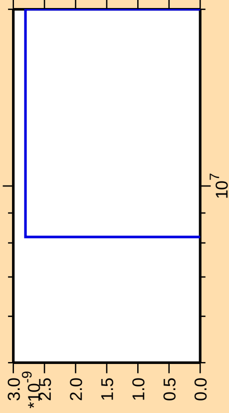
\Delta\sigma/\sigma vs. E for ^{207}\text{Bi}(\text{mt } 42)
