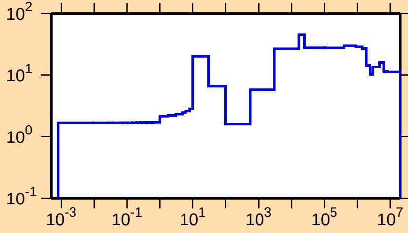
\Delta\sigma/\sigma vs. E for ^{207}\text{Bi}(n,\text{el.})
