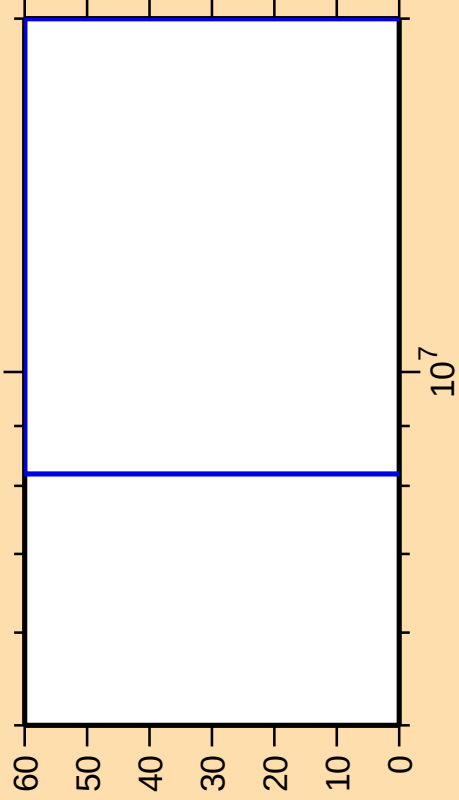
\Delta\sigma/\sigma vs. E for ^{207}\text{Bi}(n,2np)
