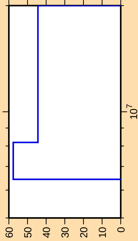
\Delta\sigma/\sigma vs. E for ^{207}\text{Bi}(n,p)
