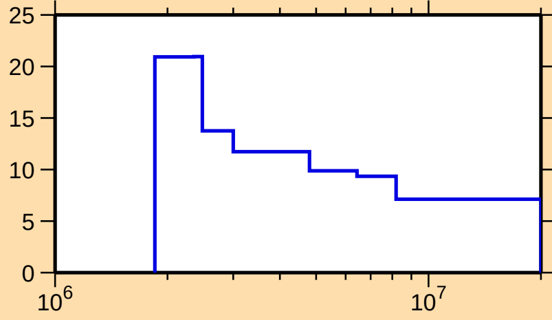
\Delta\sigma/\sigma vs. E for ^{207}\text{Bi}(n,n\text{onel.})
