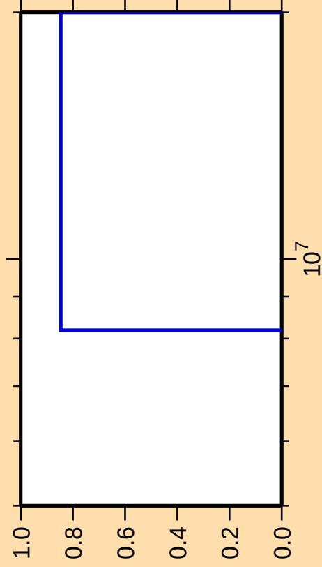
\Delta\sigma/\sigma vs. E for ^{207}\text{Bi}(n,p\alpha)
