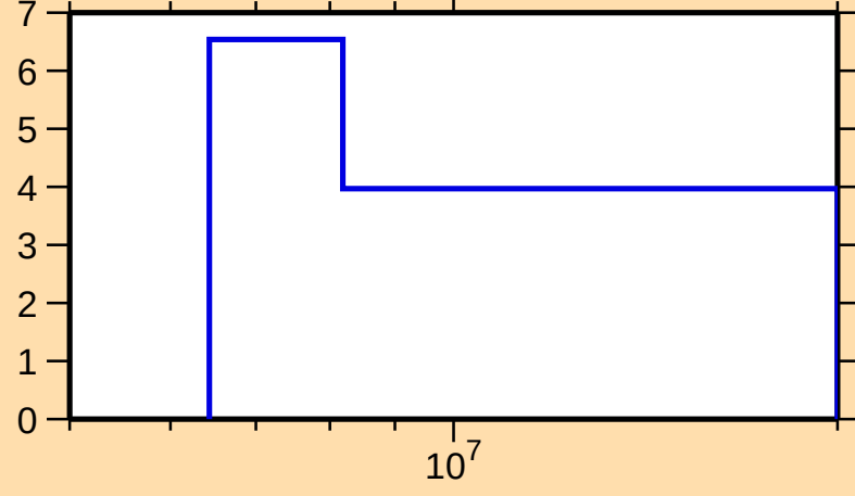
\Delta\sigma/\sigma vs. E for ^{207}\text{Bi}(n,\text{tot.})
