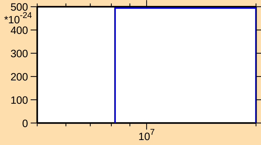
\sigma vs. E for ^{207}\text{Bi}(\text{mt } 42)
