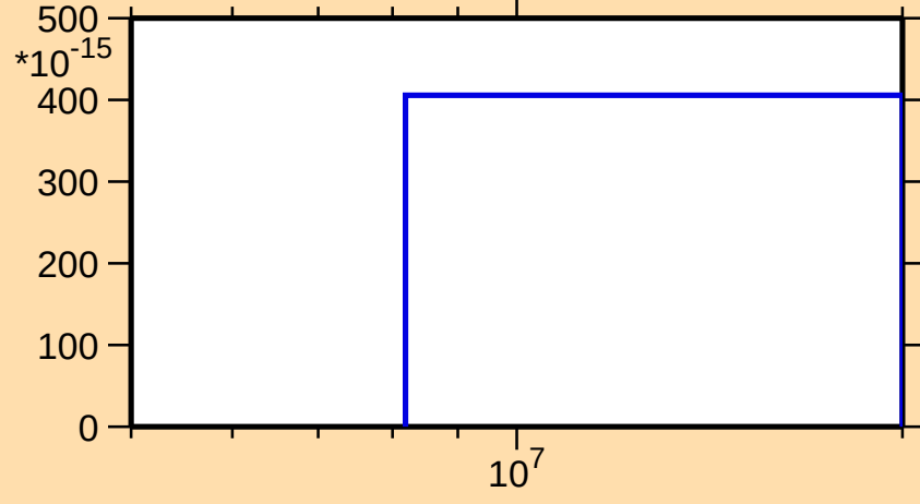
\sigma vs. E for ^{207}\text{Bi}(n,p\alpha)
