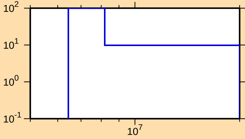
\Delta\sigma/\sigma vs. E for ^{207}\text{Bi}(n,2n)
