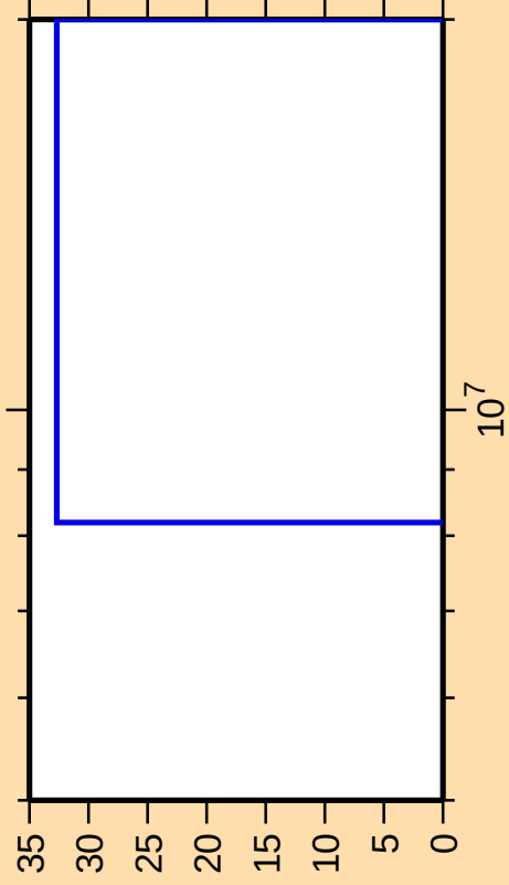
\Delta\sigma/\sigma vs. E for ^{207}\text{Bi}(n,3n)
