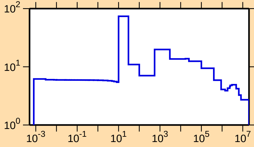
\sigma vs. E for ^{207}\text{Bi}(n,\text{el.})
