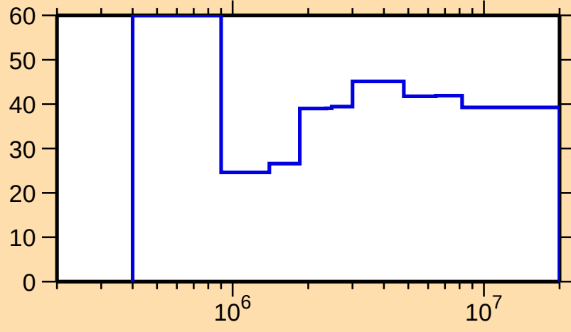
\Delta\sigma/\sigma vs. E for ^{207}\text{Bi}(n,n_1)
