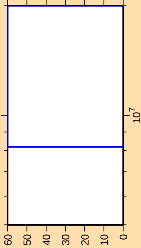
\Delta\sigma/\sigma vs. E for ^{207}\text{Bi}(n,2n\alpha)
