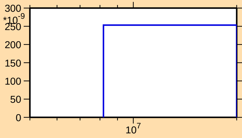
\sigma vs. E for ^{207}\text{Bi}(n,2np)
