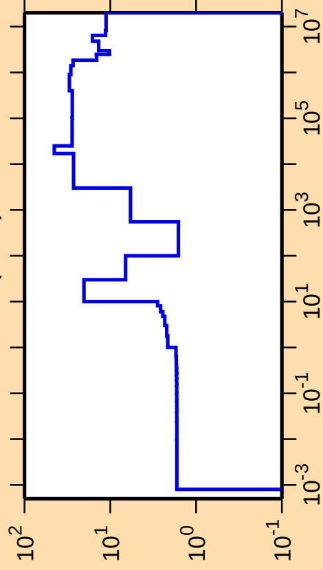
\Delta\sigma/\sigma vs. E for ^{207}\text{Bi}(n,\text{el.})
