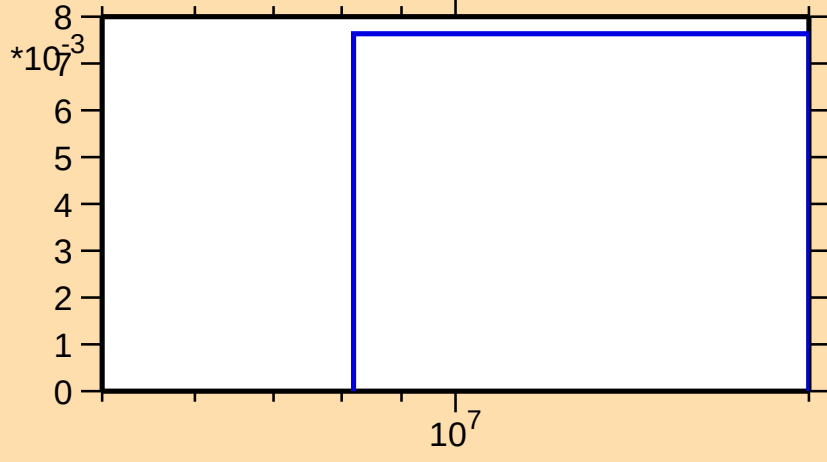
\sigma vs. E for ^{207}\text{Bi}(n,3n)
