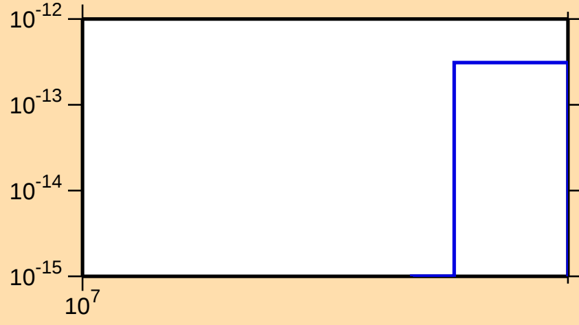
\sigma vs. E for ^{210}\text{Bi} (mt 34)
