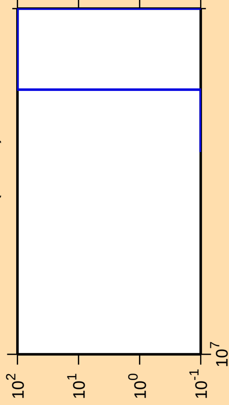
\Delta\sigma/\sigma vs. E for ^{210}\text{Bi}(\text{mt } 42)
