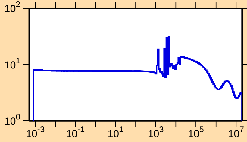
\sigma vs. E for ^{210}\text{Bi}(n,\text{el.})
