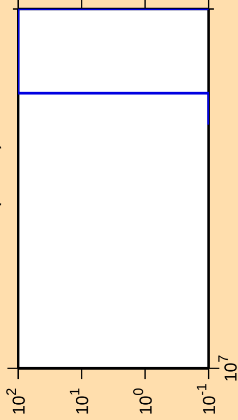
\Delta\sigma/\sigma vs. E for ^{210}\text{Bi}(\text{mt 11})
