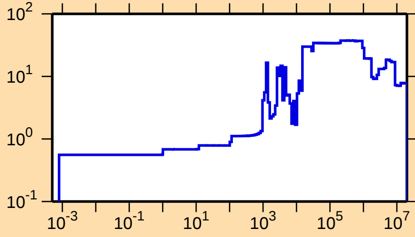
\Delta\sigma/\sigma vs. E for ^{210}\text{Bi}(n,\text{el.})
