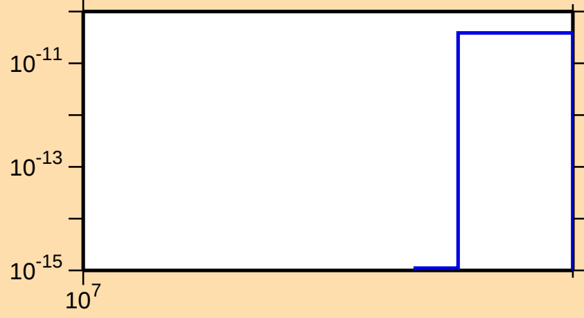
\sigma vs. E for ^{210}\text{Bi}(\text{mt 11})
