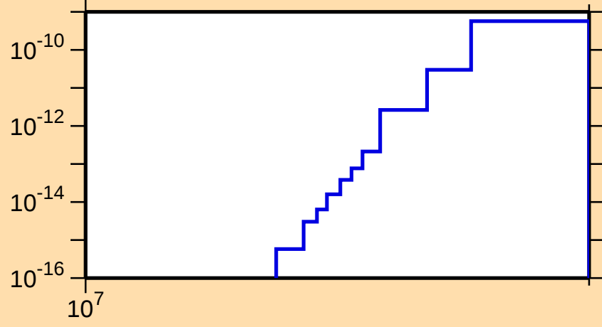
\sigma vs. E for ^{210}\text{Bi}(n,\text{He3})
