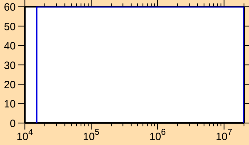
\Delta\sigma/\sigma vs. E for ^{210}\text{Bi}(n,n_1)
