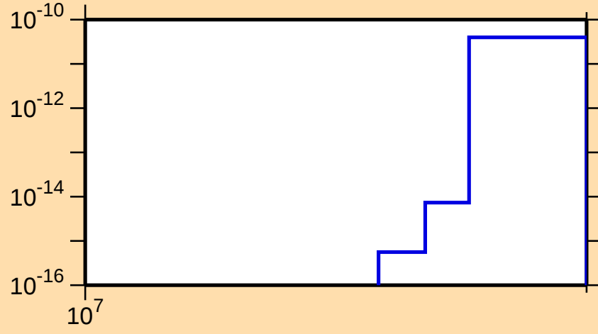
\sigma vs. E for ^{210}\text{Bi}(\text{mt } 42)
