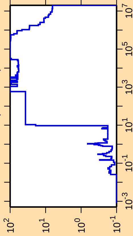
\Delta\sigma/\sigma vs. E for ^{210}\text{Bi}(n,\text{nonel.})
