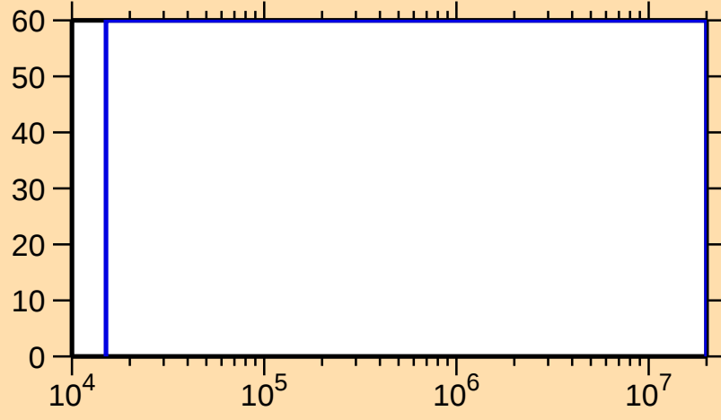
\Delta\sigma/\sigma vs. E for ^{210}\text{Bi}(n,n_1)
