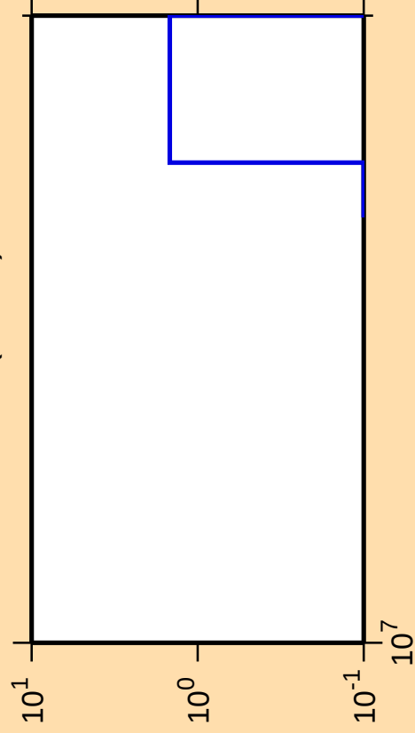
\Delta\sigma/\sigma vs. E for ^{210}\text{Bi} (mt 34)
