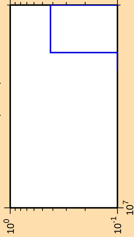
\Delta\sigma/\sigma vs. E for ^{212}\text{Bi} (mt 34)
