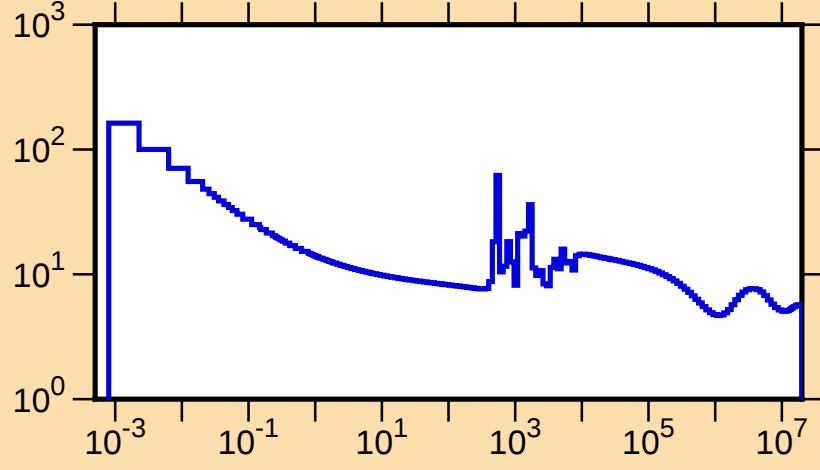
\sigma vs. E for ^{212}\text{Bi}(n,\text{tot.})
