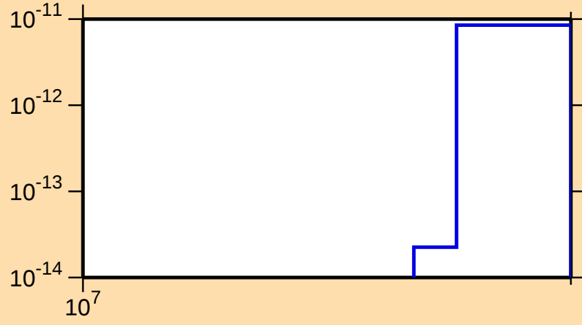
\sigma vs. E for ^{212}\text{Bi}(\text{mt 45})
