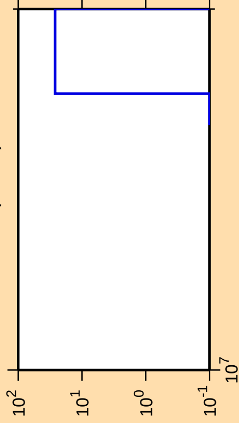
\Delta\sigma/\sigma vs. E for ^{212}\text{Bi}(\text{mt 45})
