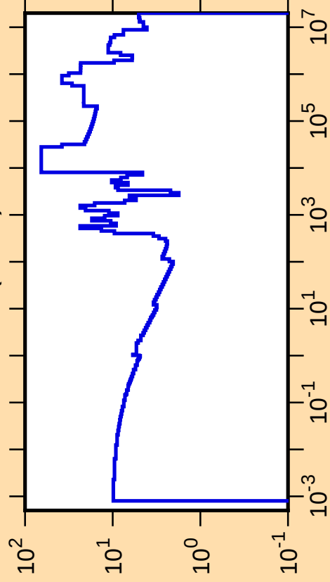
\Delta\sigma/\sigma vs. E for ^{212}\text{Bi}(n,\text{tot.})
