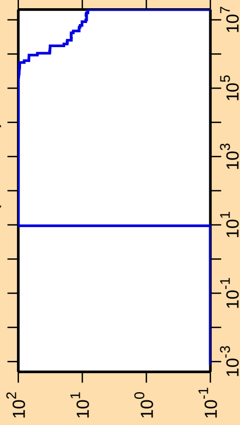
\Delta\sigma/\sigma vs. E for ^{212}\text{Bi}(n,\text{nonel.})
