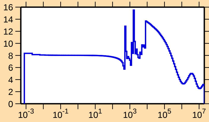
\sigma vs. E for ^{212}\text{Bi}(n,\text{el.})
