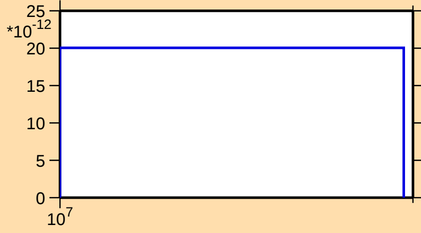
\sigma vs. E for ^{212}\text{Bi}(\text{mt } 42)
