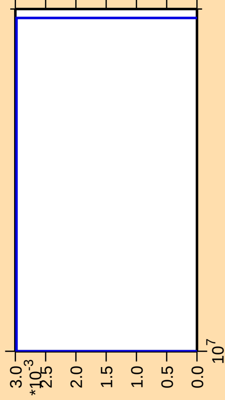
\Delta\sigma/\sigma vs. E for ^{212}\text{Bi}(\text{mt } 34)
