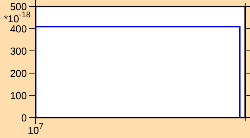
\sigma vs. E for ^{212}\text{Bi}(\text{mt } 34)
