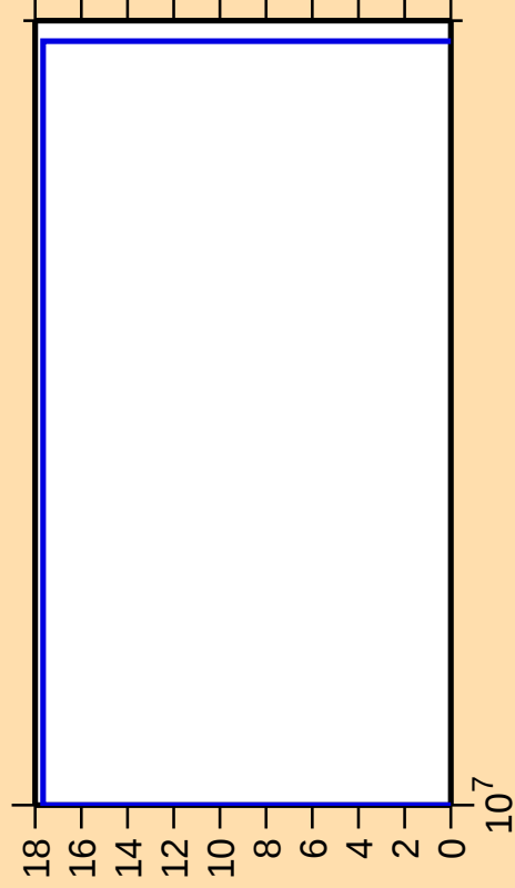
\Delta\sigma/\sigma vs. E for ^{212}\text{Bi}(\text{mt } 42)
