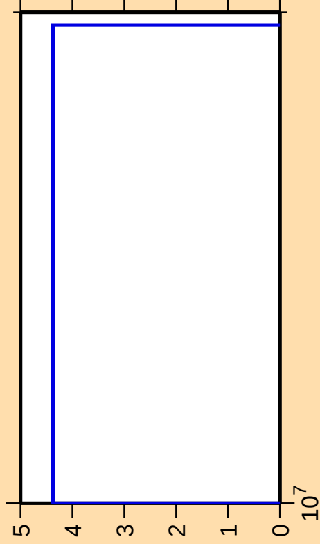
\Delta\sigma/\sigma vs. E for ^{212}\text{Bi}(\text{mt117})
