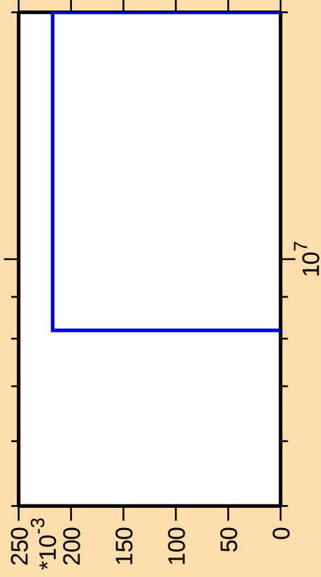
\Delta\sigma/\sigma vs. E for ^{212}\text{Bi}(\text{mt } 45)
