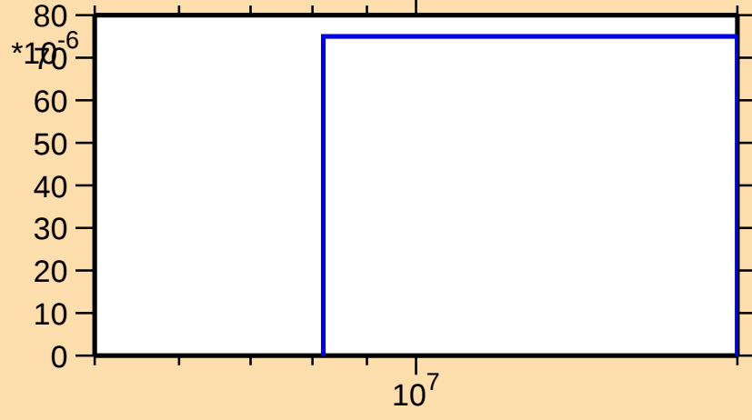
\sigma vs. E for ^{212}\text{Bi}(n,\text{nt})
