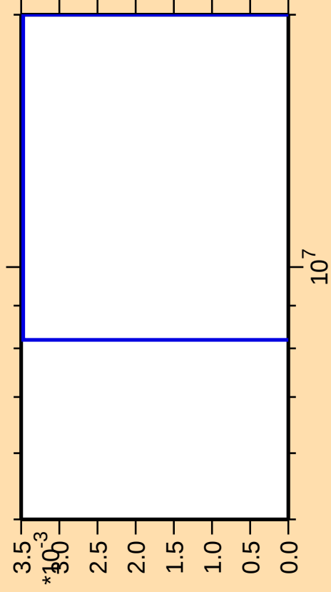
\Delta\sigma/\sigma vs. E for ^{212}\text{Bi}(\text{mt } 34)
