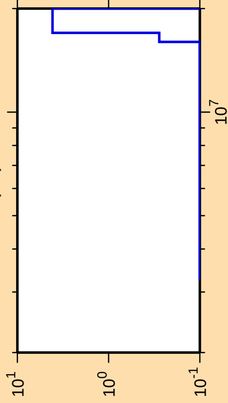
\Delta\sigma/\sigma vs. E for ^{222}\text{Bi}(n,f)
