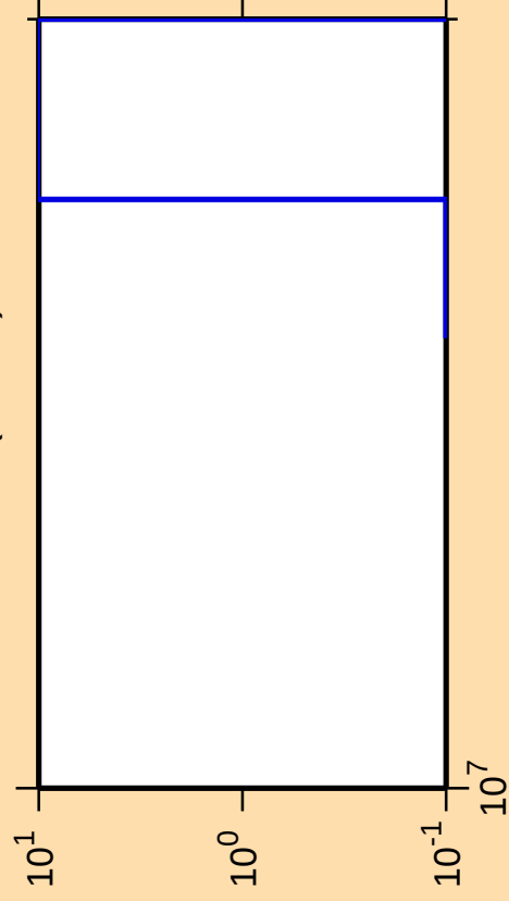
\Delta\sigma/\sigma vs. E for ^{222}\text{Bi}(\text{mt } 42)
