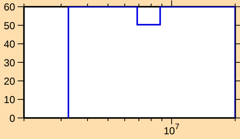
\Delta\sigma/\sigma vs. E for ^{222}\text{Bi}(n,2n)
