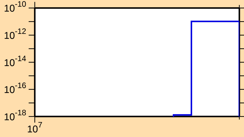
\sigma vs. E for ^{222}\text{Bi}(\text{mt } 42)
