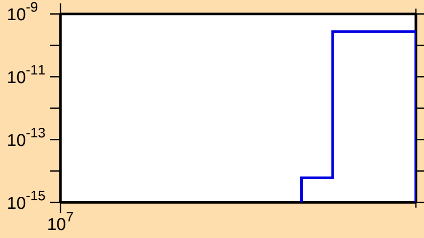
\sigma vs. E for ^{222}\text{Bi}(\text{mt 11})
