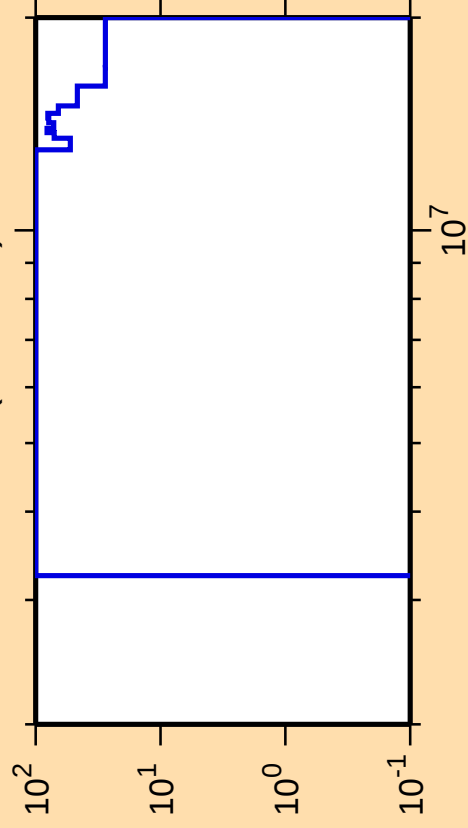
\Delta\sigma/\sigma vs. E for ^{222}\text{Bi}(n,n\text{cont.})
