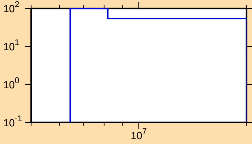
\Delta\sigma/\sigma vs. E for ^{222}\text{Bi}(n,p)
