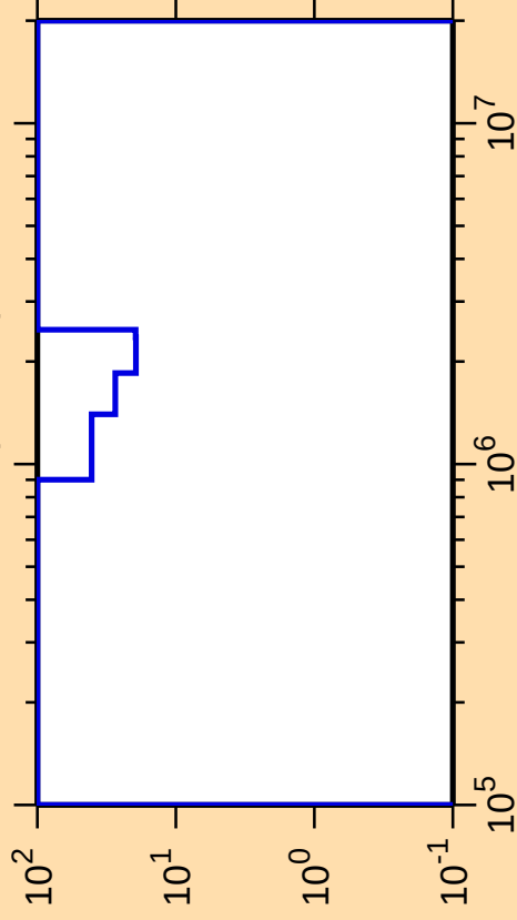
\Delta\sigma/\sigma vs. E for ^{222}\text{Bi}(n,\text{inel.})
