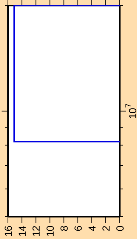
\Delta\sigma/\sigma vs. E for ^{222}\text{Bi}(\text{mt } 11)
