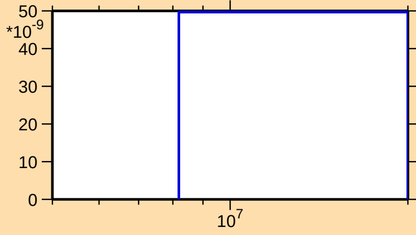
\sigma vs. E for ^{222}\text{Bi}(n,2n\alpha)
