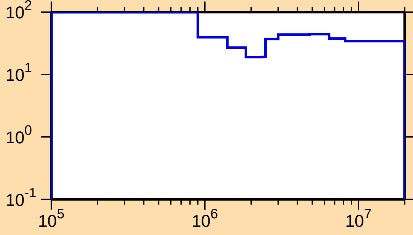
\Delta\sigma/\sigma vs. E for ^{222}\text{Bi}(n,\text{nonel.})
