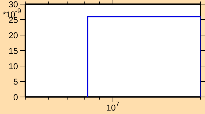
\sigma vs. E for ^{222}\text{Bi}(n,2np)
