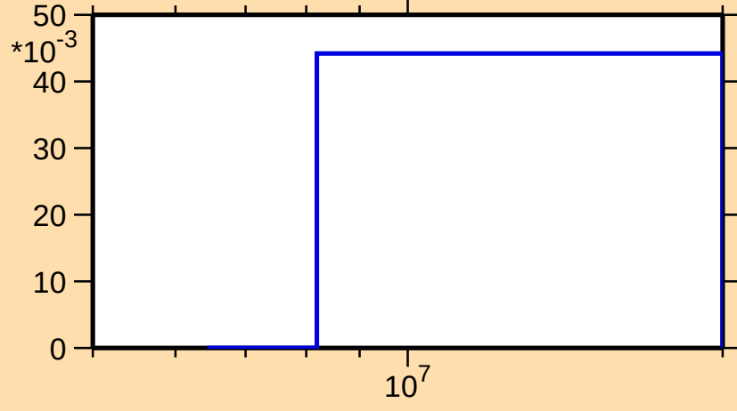
\Delta\sigma/\sigma vs. E for ^{222}\text{Bi}(n,f)
