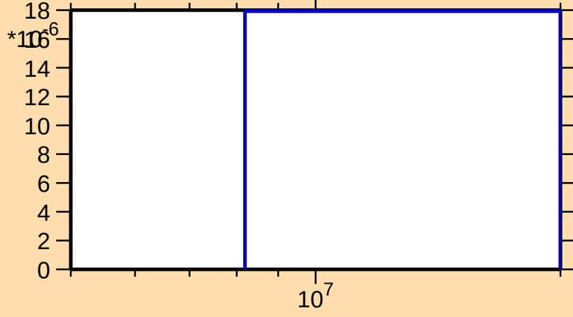
\sigma vs. E for ^{222}\text{Bi}(n,d)
