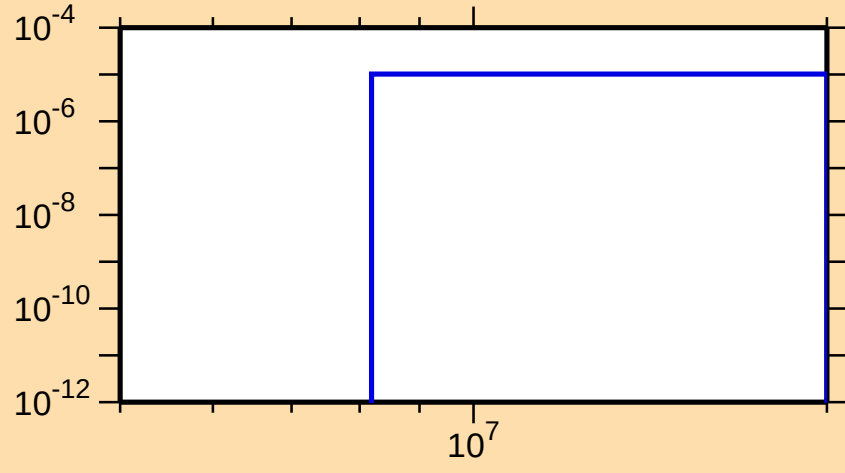
\sigma vs. E for ^{222}\text{Bi}(n,np)
