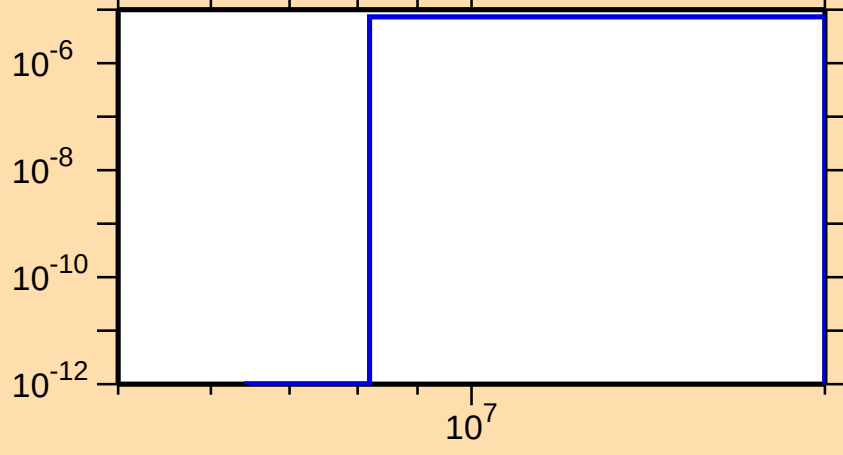
\sigma vs. E for ^{222}\text{Bi}(n,n\alpha)
