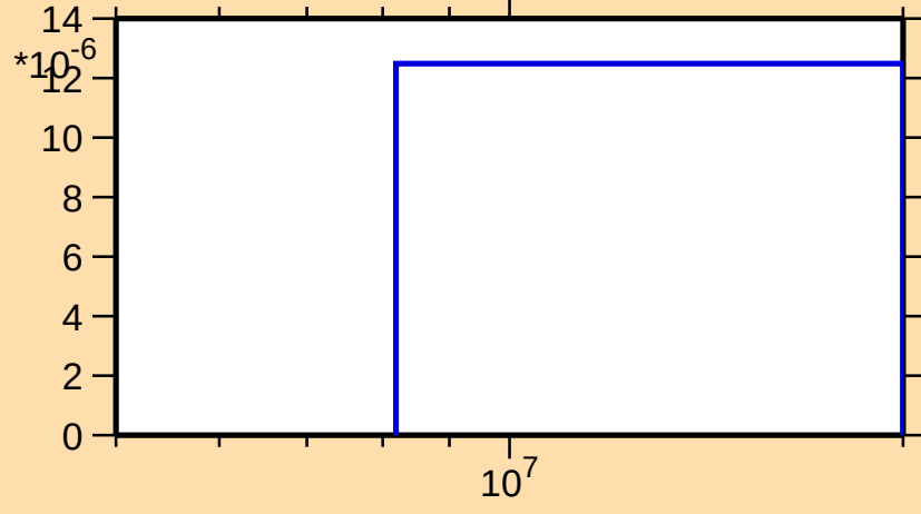
\sigma vs. E for ^{222}\text{Bi}(n,\text{nt})
