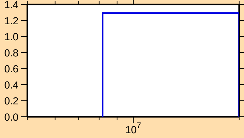
\sigma vs. E for ^{222}\text{Bi}(n,3n)
