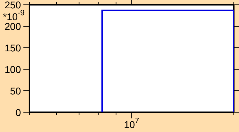
\sigma vs. E for ^{222}\text{Bi}(n,\text{nd})
