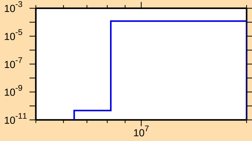
\sigma vs. E for ^{222}\text{Bi}(n,t)
