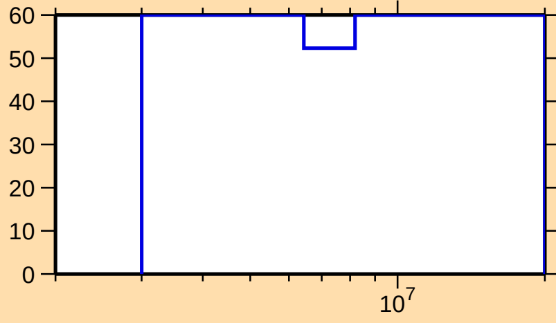
\Delta\sigma/\sigma vs. E for ^{222}\text{Bi}(n,2n)
