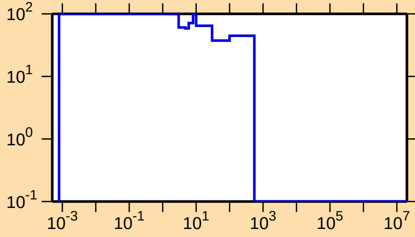
\Delta\sigma/\sigma vs. E for ^{222}\text{Bi}(n,f)
