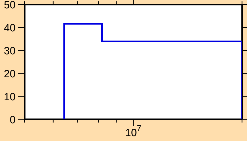
\Delta\sigma/\sigma vs. E for ^{222}\text{Bi}(n,\text{tot.})
