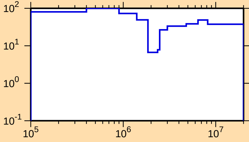
\Delta\sigma/\sigma vs. E for ^{222}\text{Bi}(n,\text{el.})
