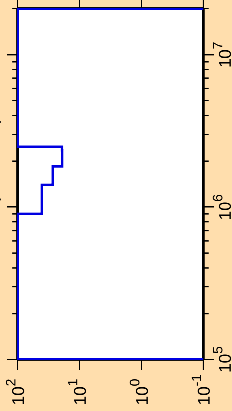
\Delta\sigma/\sigma vs. E for ^{222}\text{Bi}(n,\text{ncont.})
