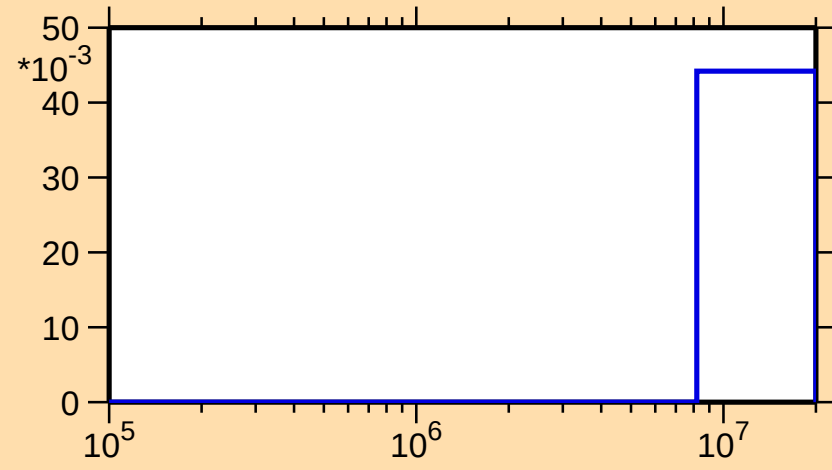
\Delta\sigma/\sigma vs. E for ^{222}\text{Bi}(n,\text{f})
