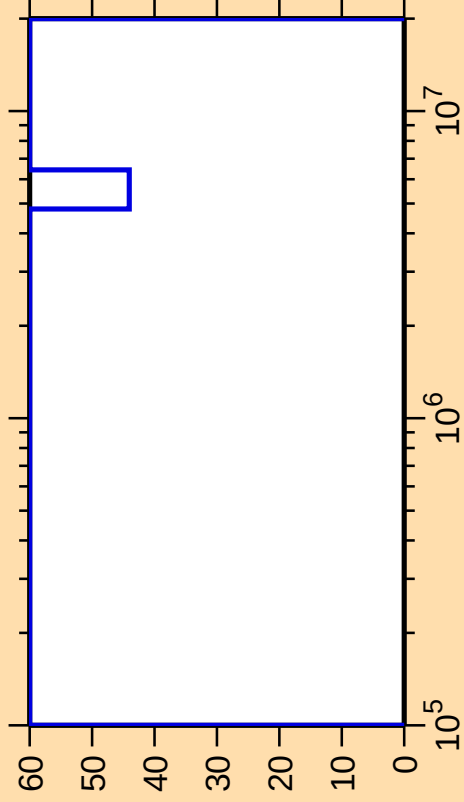
\Delta\sigma/\sigma vs. E for ^{222}\text{Bi}(n,\gamma)
