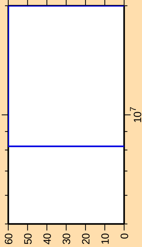
\Delta\sigma/\sigma vs. E for ^{222}\text{Bi}(n,\text{nt})
