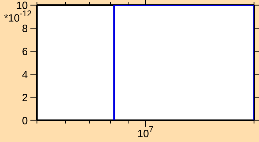
\sigma vs. E for ^{222}\text{Bi}(n,3n\alpha)
