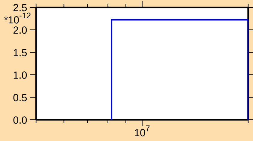
\sigma vs. E for ^{222}\text{Bi}(\text{mt } 11)
