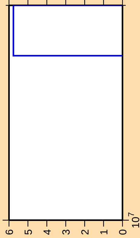
\Delta\sigma/\sigma vs. E for ^{240}\text{Bk}(n,3n\alpha)
