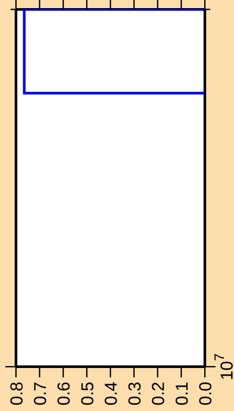
\Delta\sigma/\sigma vs. E for ^{240}\text{Bk}(\text{mt } 34)
