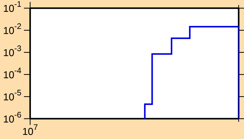
\sigma vs. E for ^{240}\text{Bk}(n,3n)
