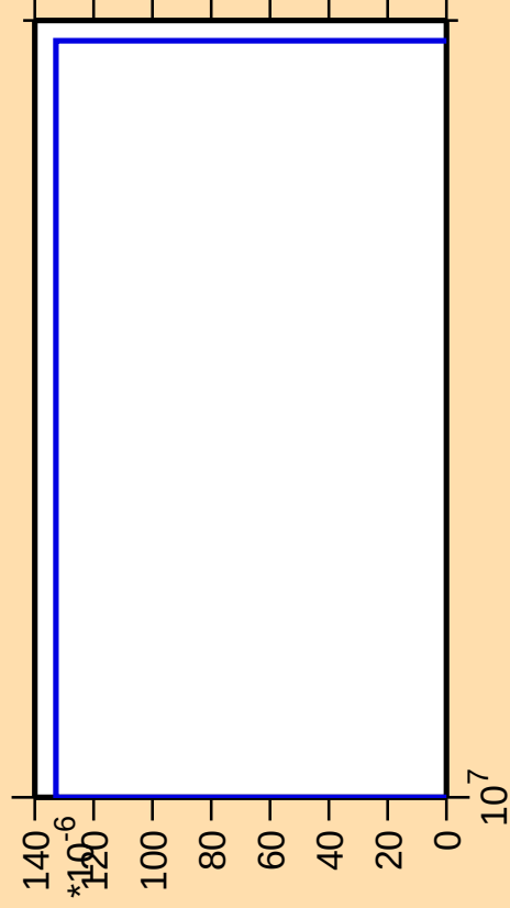
\Delta\sigma/\sigma vs. E for ^{240}\text{Bk}(\text{mt 11})
