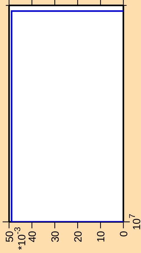
\Delta\sigma/\sigma vs. E for ^{240}\text{Bk}(n,3n\alpha)
