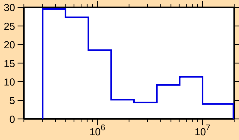
\Delta\sigma/\sigma vs. E for ^{240}\text{Bk}(n,\text{tot.})
