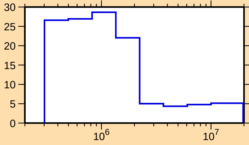
\Delta\sigma/\sigma vs. E for ^{240}\text{Bk}(n,\text{nonel.})
