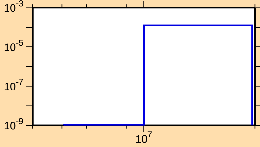
\sigma vs. E for ^{240}\text{Bk}(n,t)
