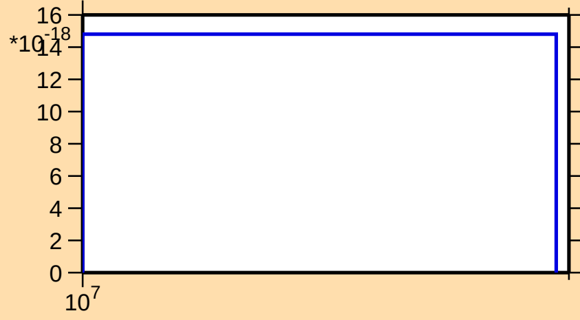
\sigma vs. E for ^{240}\text{Bk}(\text{mt 11})
