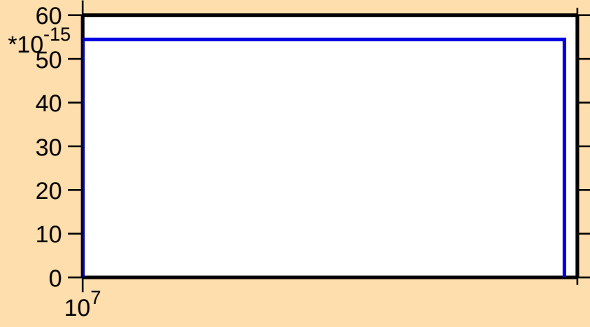
\sigma vs. E for ^{240}\text{Bk}(n,3n\alpha)
