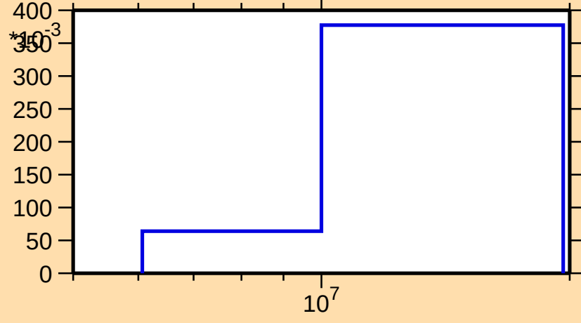
\sigma vs. E for ^{240}\text{Bk}(n,2n)
