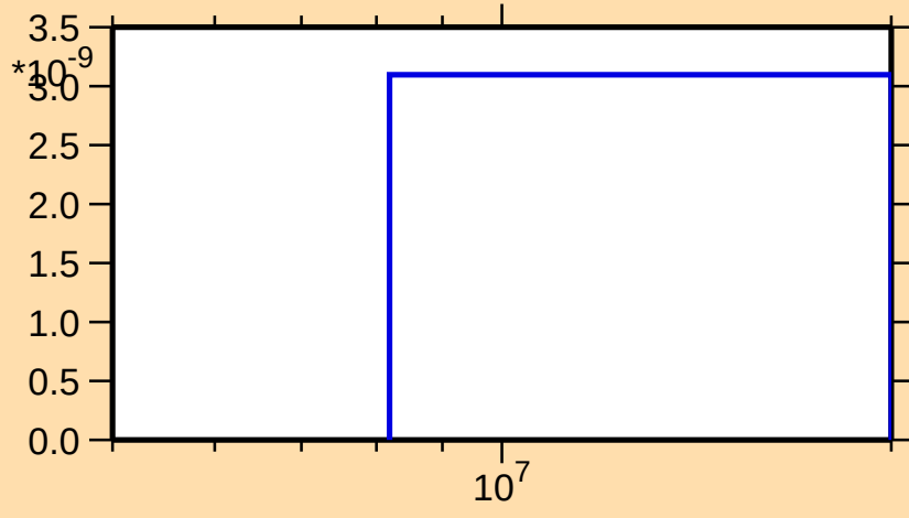
\sigma vs. E for ^{240}\text{Bk}(n,\text{He3})
