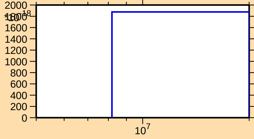
\sigma vs. E for ^{240}\text{Bk}(\text{mt } 34)
