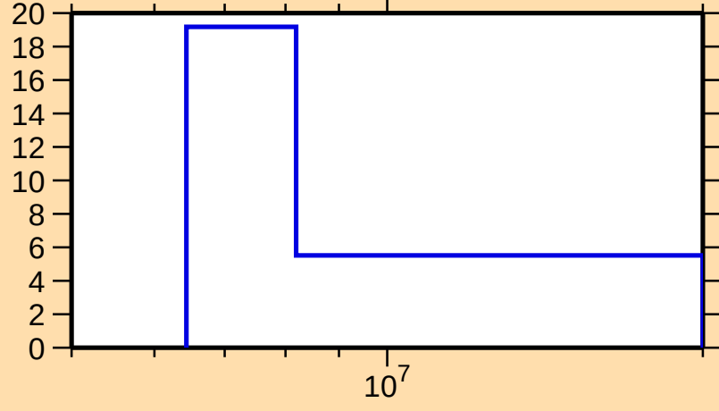
\Delta\sigma/\sigma vs. E for ^{240}\text{Bk}(n,\text{el.})
