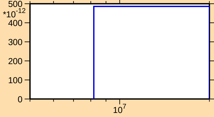
\sigma vs. E for ^{240}\text{Bk}(n,nt)
