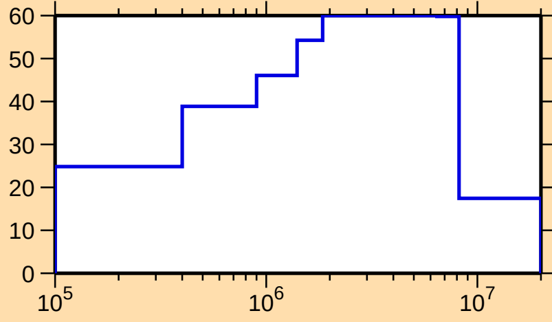
\Delta\sigma/\sigma vs. E for ^{240}\text{Bk}(n,f)
