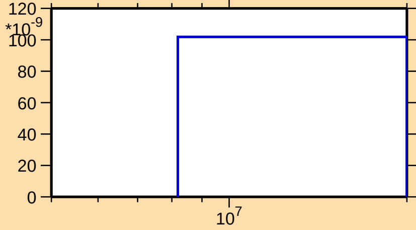
\sigma vs. E for ^{240}\text{Bk}(n,2np)
