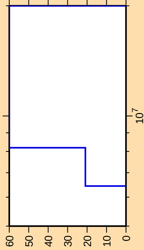
\Delta\sigma/\sigma vs. E for ^{240}\text{Bk}(n,t)
