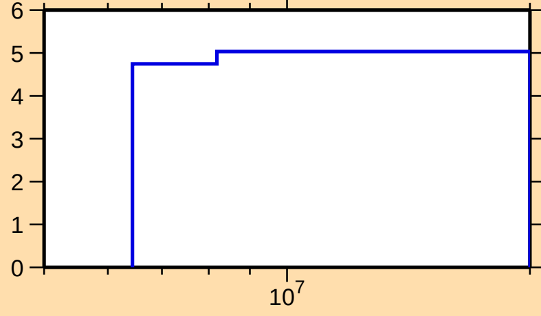
\Delta\sigma/\sigma vs. E for ^{240}\text{Bk}(n,\text{nonel.})
