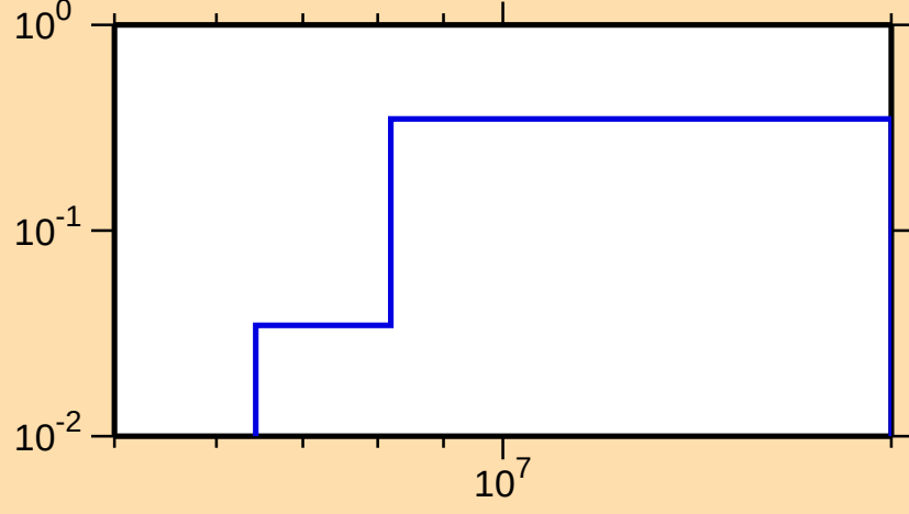
\sigma vs. E for ^{240}\text{Bk}(n,2n)
