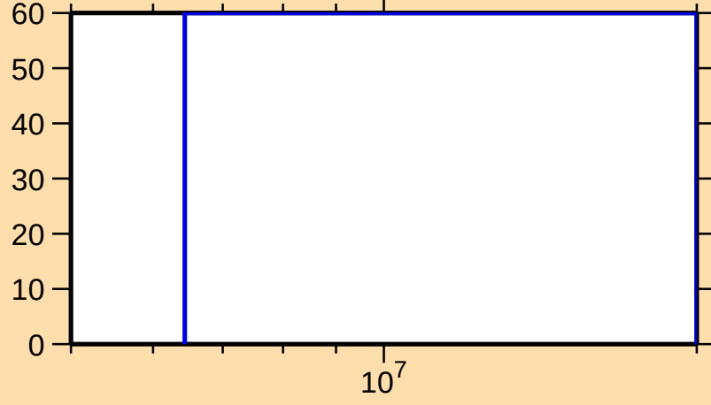
\Delta\sigma/\sigma vs. E for ^{240}\text{Bk}(n,\text{inel.})
