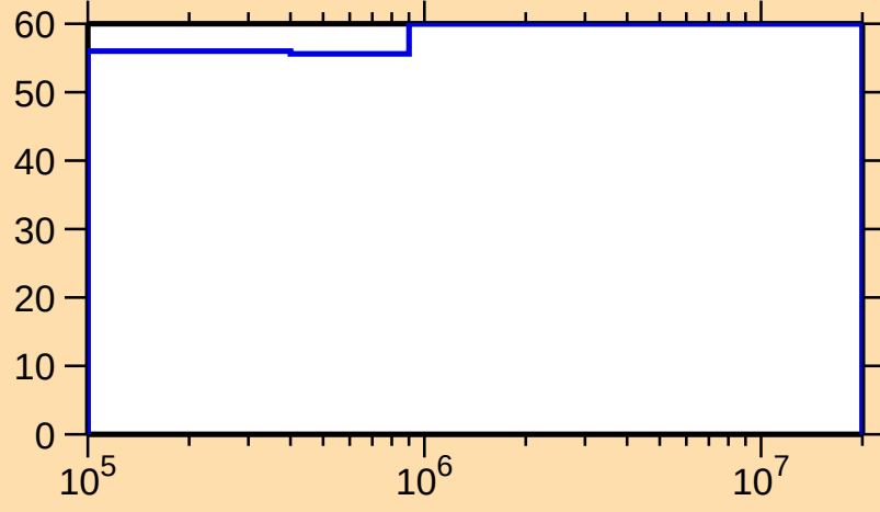
\Delta\sigma/\sigma vs. E for ^{240}\text{Bk}(n,n_1)
