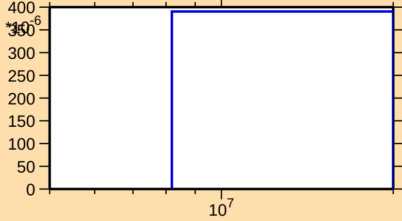
\sigma vs. E for ^{240}\text{Bk}(n,3n)
