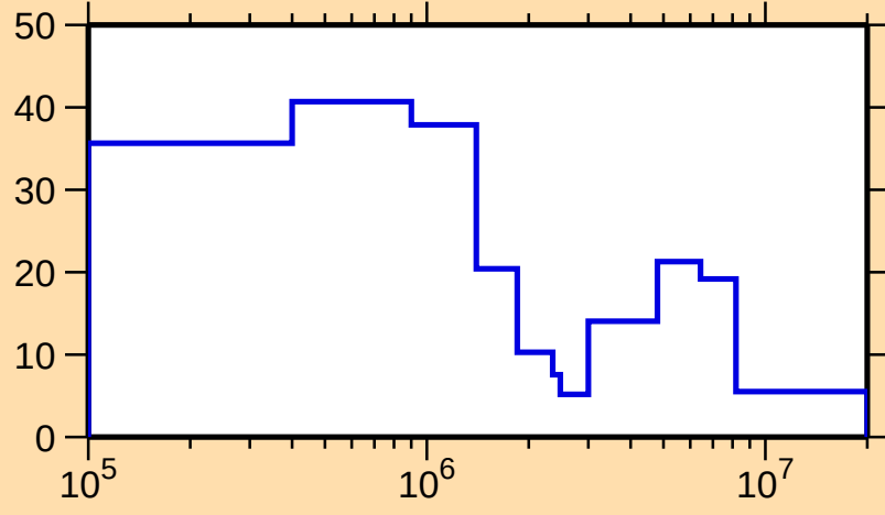
\Delta\sigma/\sigma vs. E for ^{240}\text{Bk}(n,\text{el.})
