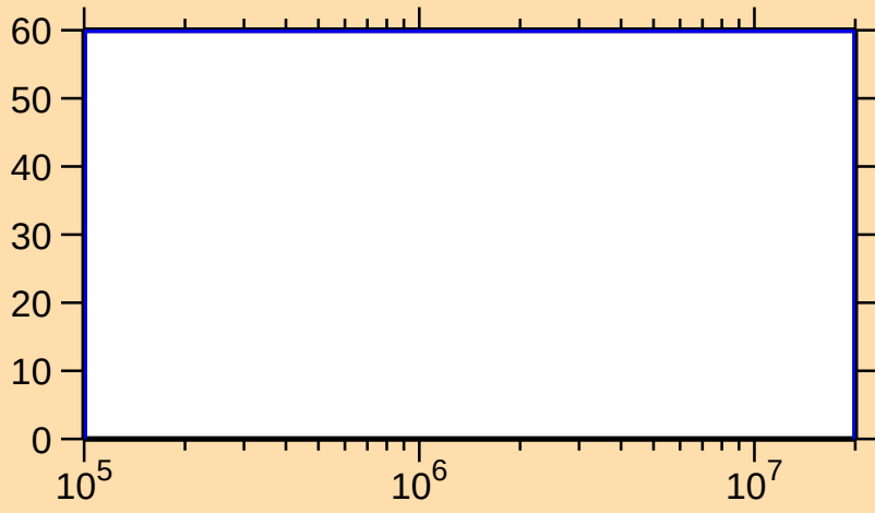
\Delta\sigma/\sigma vs. E for ^{240}\text{Bk}(n,\text{inel.})
