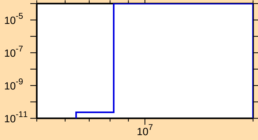
\sigma vs. E for ^{240}\text{Bk}(n,t)
