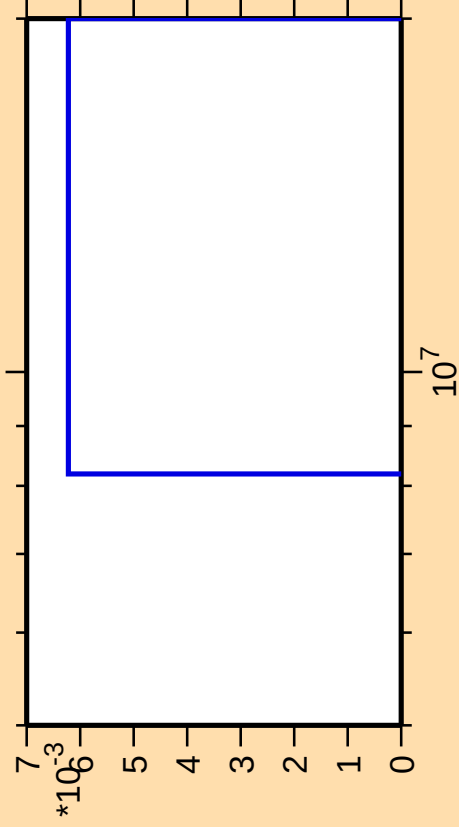
\Delta\sigma/\sigma vs. E for ^{240}\text{Bk}(\text{mt } 34)
