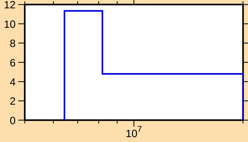
\Delta\sigma/\sigma vs. E for ^{240}\text{Bk}(n,\text{tot.})
