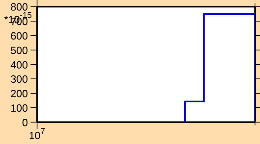
\sigma vs. E for ^{242}\text{Bk}(\text{mt } 45)
