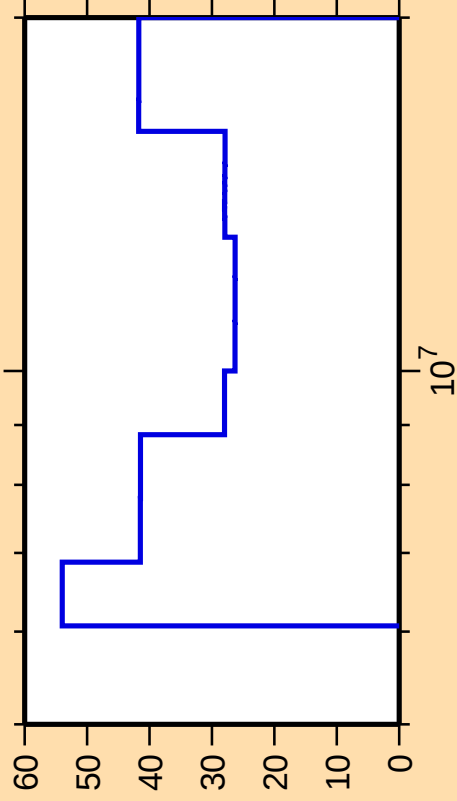
\Delta\sigma/\sigma vs. E for ^{242}\text{Bk}(n,p)
