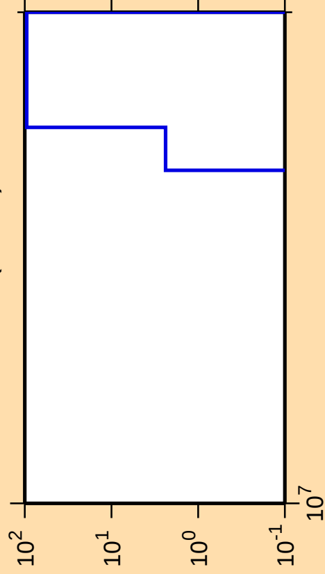
\Delta\sigma/\sigma vs. E for ^{242}\text{Bk}(n,3n\alpha)
