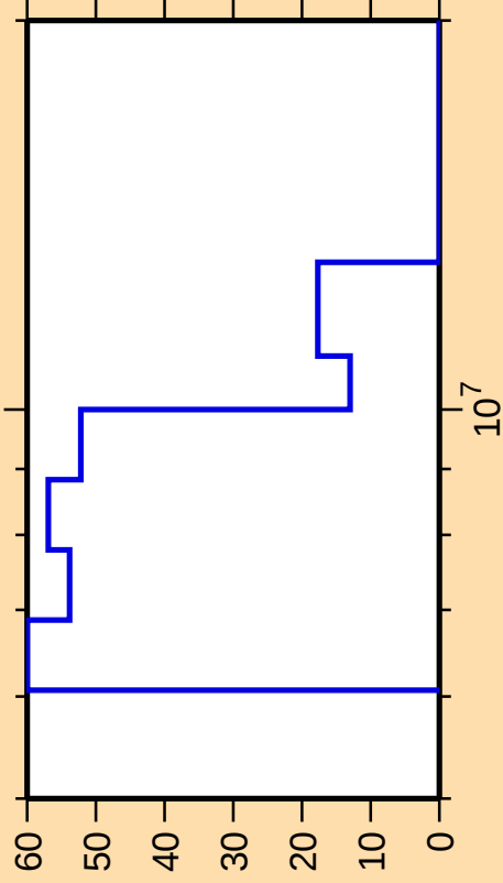
\Delta\sigma/\sigma vs. E for ^{242}\text{Bk}(n,n_1)
