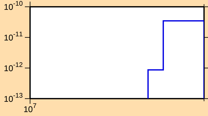
\sigma vs. E for ^{242}\text{Bk}(n,3n\alpha)
