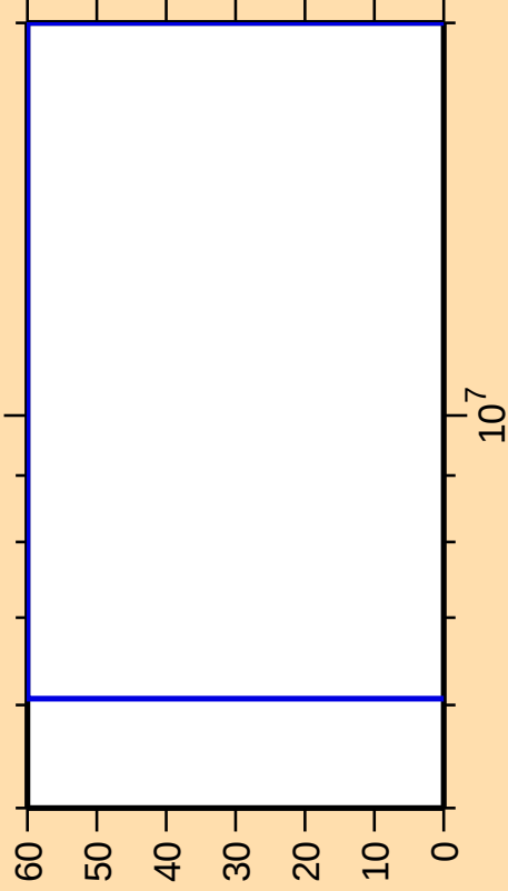
\Delta\sigma/\sigma vs. E for ^{242}\text{Bk}(n,\gamma)
