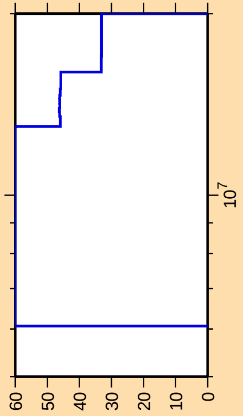
\Delta\sigma/\sigma vs. E for ^{242}\text{Bk}(n,f)
