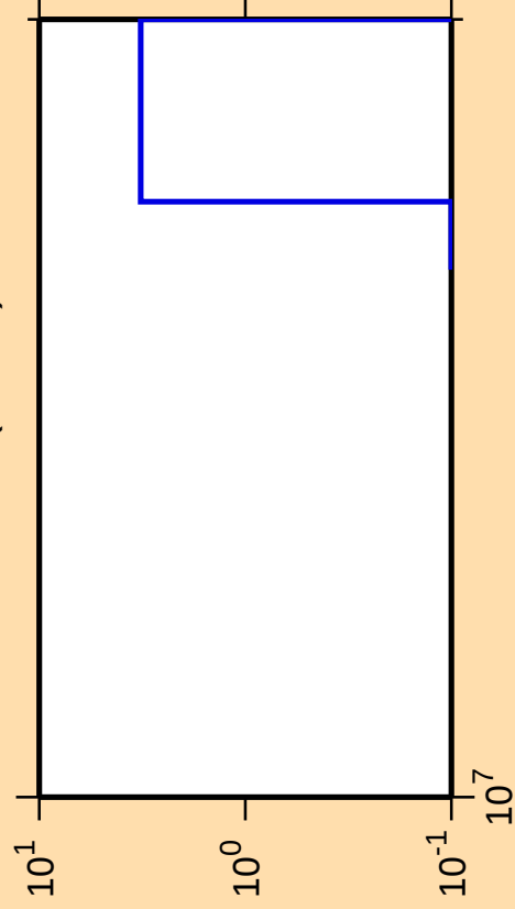
\Delta\sigma/\sigma vs. E for ^{242}\text{Bk}(\text{mt } 34)
