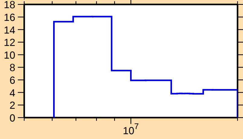
\Delta\sigma/\sigma vs. E for ^{242}\text{Bk}(n,\text{el.})
