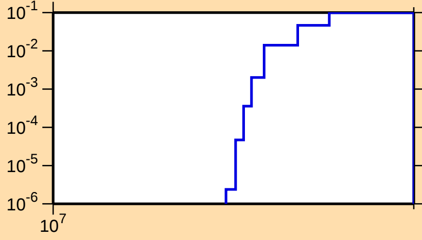
\sigma vs. E for ^{242}\text{Bk}(n,3n)
