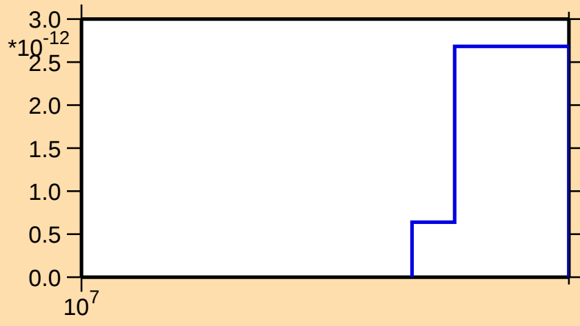
\sigma vs. E for ^{242}\text{Bk}(\text{mt117})
