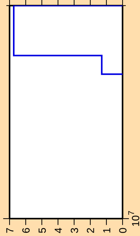
\Delta\sigma/\sigma vs. E for ^{242}\text{Bk}(\text{mt } 45)
