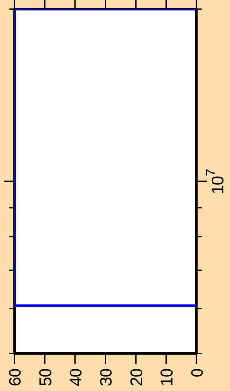
\Delta\sigma/\sigma vs. E for ^{242}\text{Bk}(n,\alpha)
