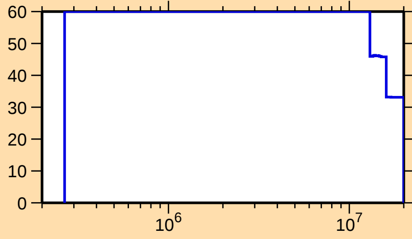
\Delta\sigma/\sigma vs. E for ^{242}\text{Bk}(n,f)
