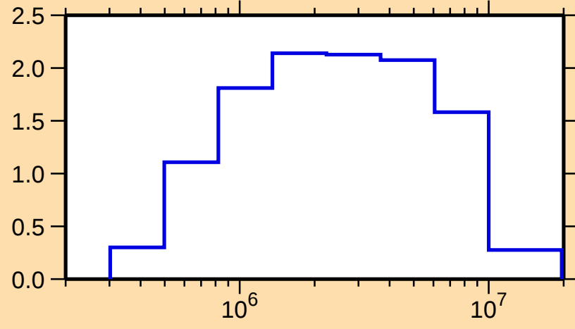
\sigma vs. E for ^{242}\text{Bk}(n,n\text{cont.})
