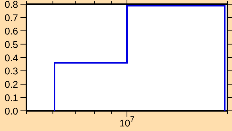
\sigma vs. E for ^{242}\text{Bk}(n,2n)
