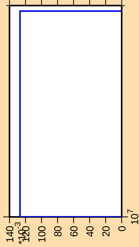
\Delta\sigma/\sigma vs. E for ^{242}\text{Bk}(\text{mt } 45)
