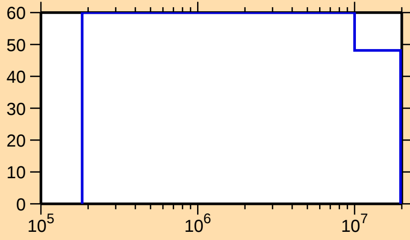
\Delta\sigma/\sigma vs. E for ^{242}\text{Bk}(n,f)
