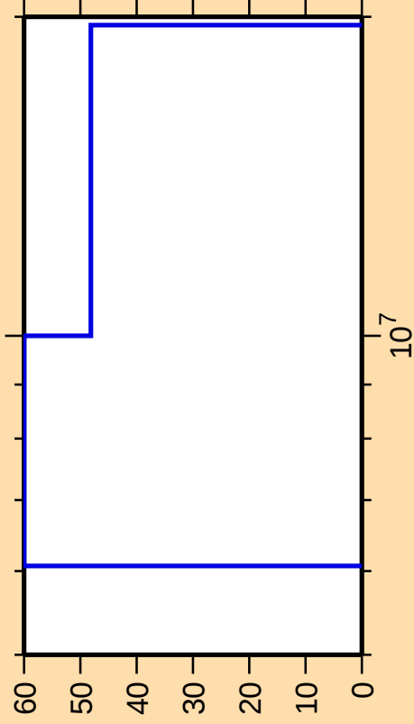
\Delta\sigma/\sigma vs. E for ^{242}\text{Bk}(n,f)
