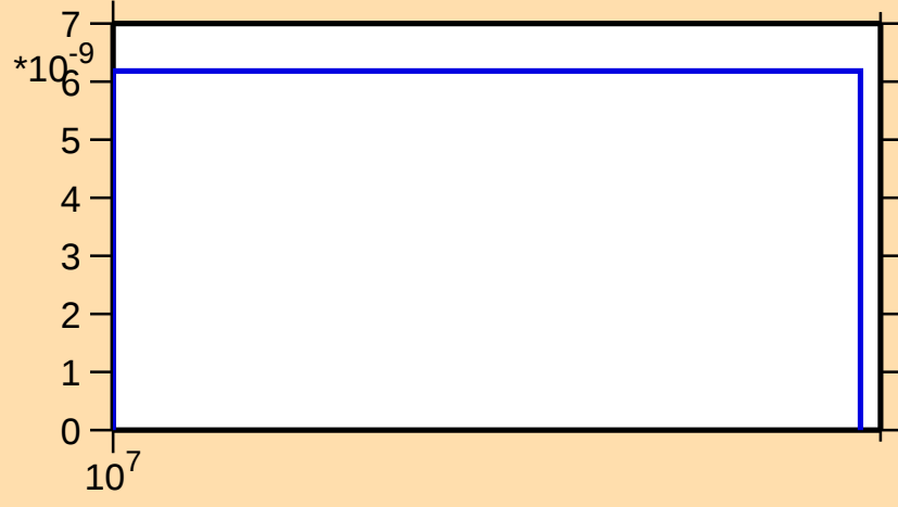
\sigma vs. E for ^{242}\text{Bk}(n,nt)
