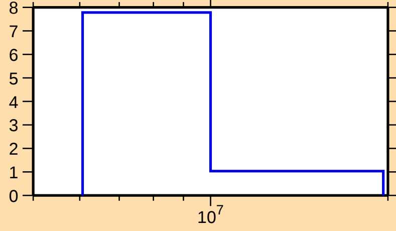
\Delta\sigma/\sigma vs. E for ^{242}\text{Bk}(n,\text{tot.})
