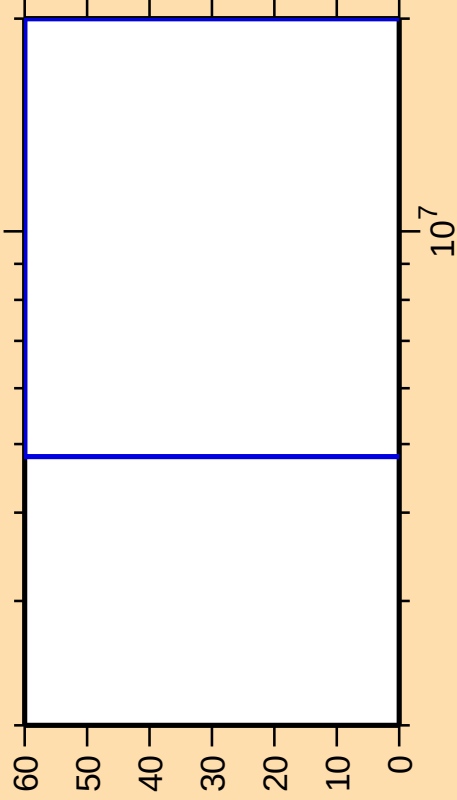
\Delta\sigma/\sigma vs. E for ^{242}\text{Bk}(n,n\text{cont.})
