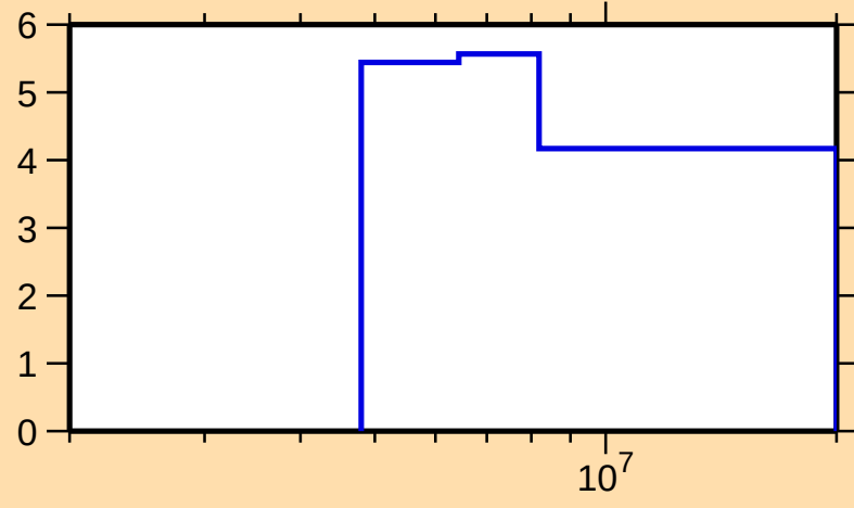
\Delta\sigma/\sigma vs. E for ^{242}\text{Bk}(n,\text{nonel.})
