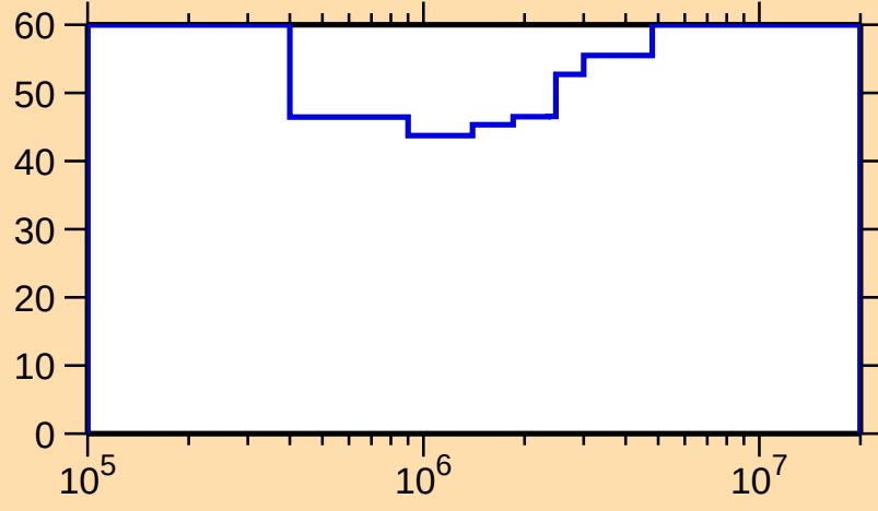
\Delta\sigma/\sigma vs. E for ^{242}\text{Bk}(n,n\text{cont.})
