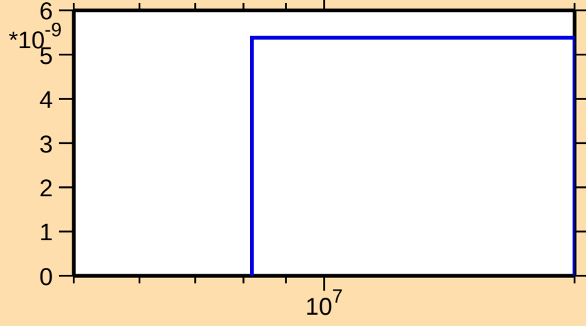
\sigma vs. E for ^{242}\text{Bk}(n,nt)
