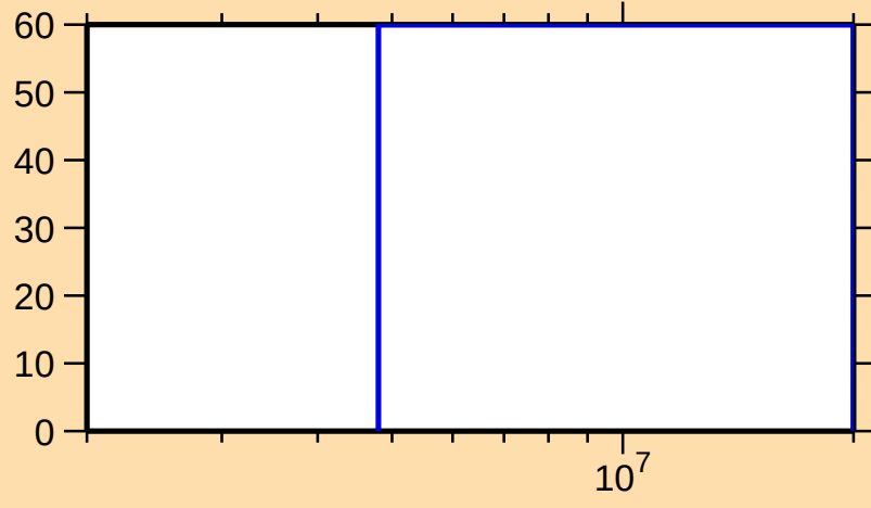
\Delta\sigma/\sigma vs. E for ^{242}\text{Bk}(n,2n)
