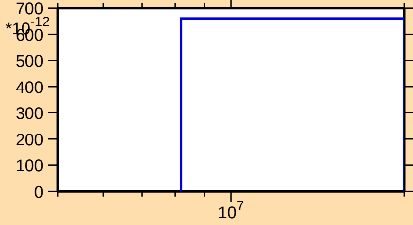
\sigma vs. E for ^{242}\text{Bk}(n,\text{He}3)
