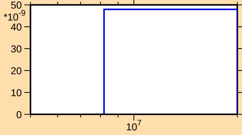
\sigma vs. E for ^{242}\text{Bk}(n,2np)
