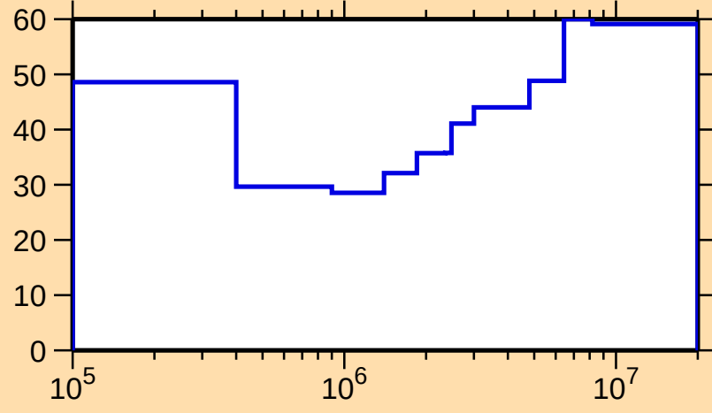
\Delta\sigma/\sigma vs. E for ^{242}\text{Bk}(n,\text{inel.})
