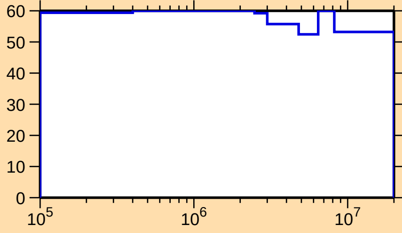
\Delta\sigma/\sigma vs. E for ^{242}\text{Bk}(n,n_1)
