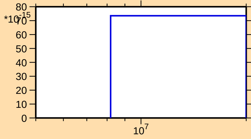
\sigma vs. E for ^{242}\text{Bk}(\text{mt117})
