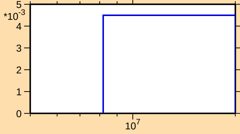
\sigma vs. E for ^{242}\text{Bk}(n,3n)
