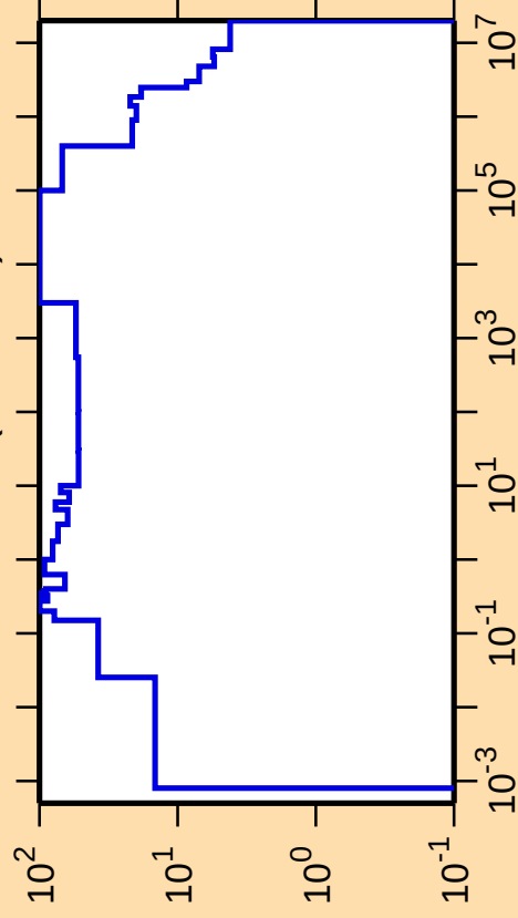
\Delta\sigma/\sigma vs. E for ^{242}\text{Bk}(n,\text{nonel.})
