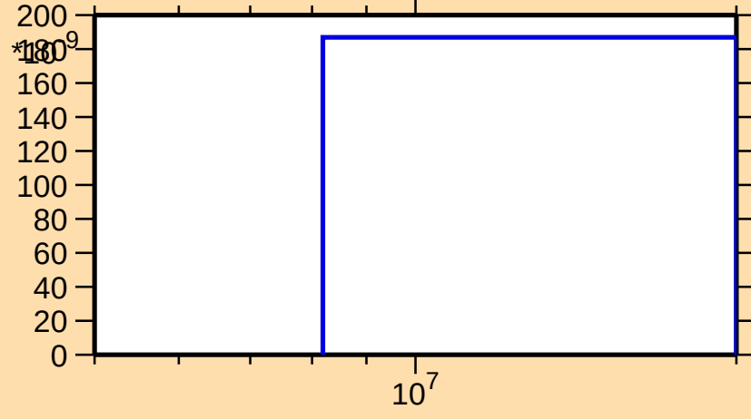
\sigma vs. E for ^{242}\text{Bk}(n,\text{nd})
