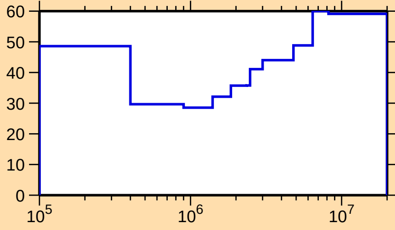
\Delta\sigma/\sigma vs. E for ^{242}\text{Bk}(n,\text{inel.})
