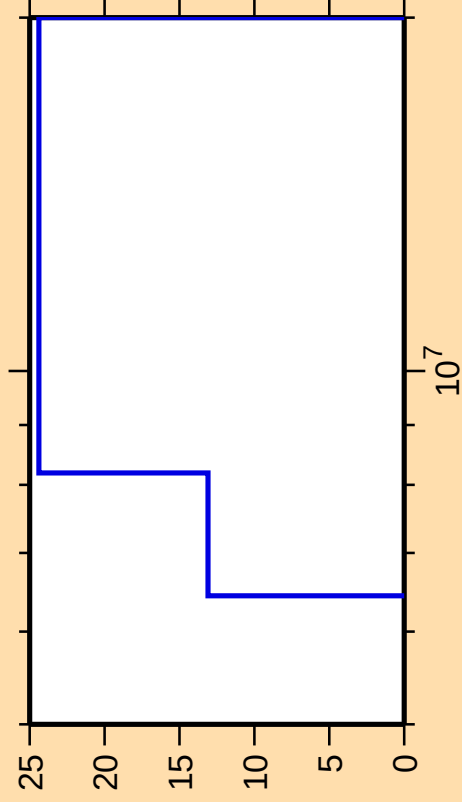
\Delta\sigma/\sigma vs. E for ^{242}\text{Bk}(n,t)
