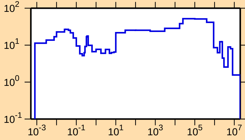
\Delta\sigma/\sigma vs. E for ^{242}\text{Bk}(n,\text{tot.})
