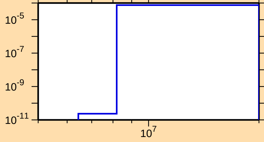
\sigma vs. E for ^{242}\text{Bk}(n,t)
