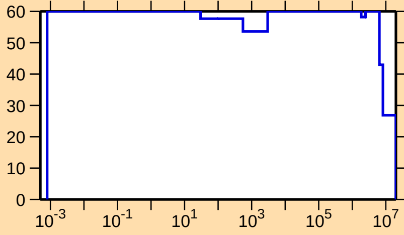
\Delta\sigma/\sigma vs. E for ^{242}\text{Bk}(n,p)
