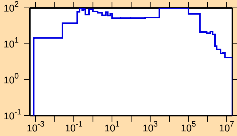
\Delta\sigma/\sigma vs. E for ^{242}\text{Bk}(n,\text{nonel.})
