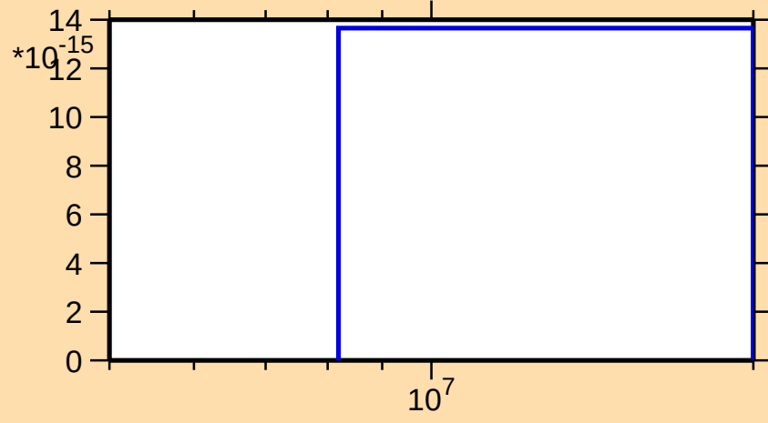
\sigma vs. E for ^{242}\text{Bk}(\text{mt } 34)
