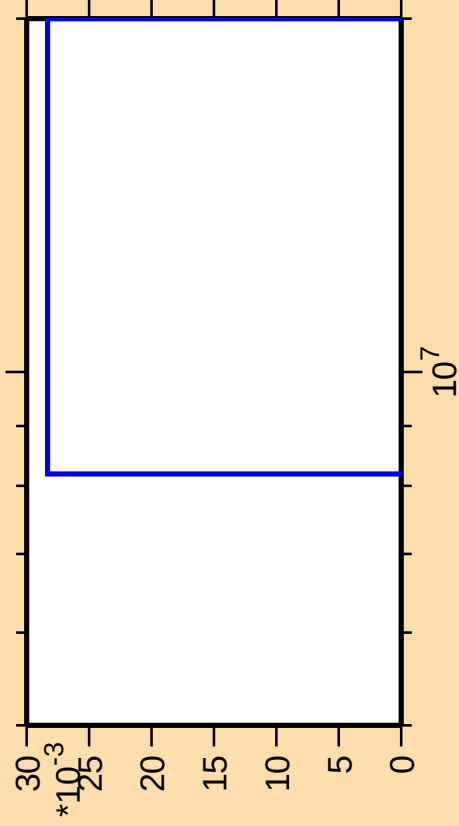
\Delta\sigma/\sigma vs. E for ^{242}\text{Bk}(\text{mt } 34)
