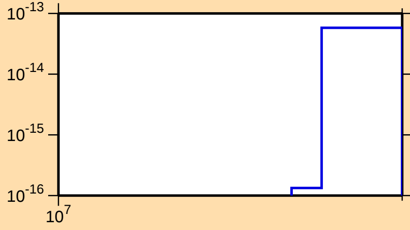
\sigma vs. E for ^{243}\text{Bk}(\text{mt } 34)
