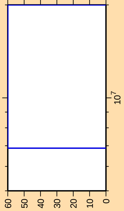
\Delta\sigma/\sigma vs. E for ^{243}\text{Bk}(n,\gamma)
