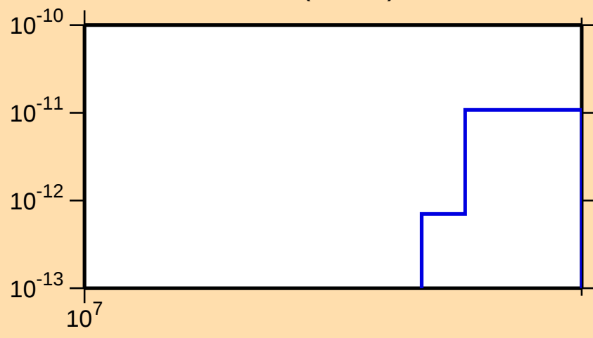
\sigma vs. E for ^{243}\text{Bk}(n,3n\alpha)
