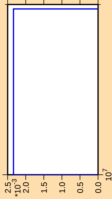
\Delta\sigma/\sigma vs. E for ^{243}\text{Bk}(\text{mt 11})
