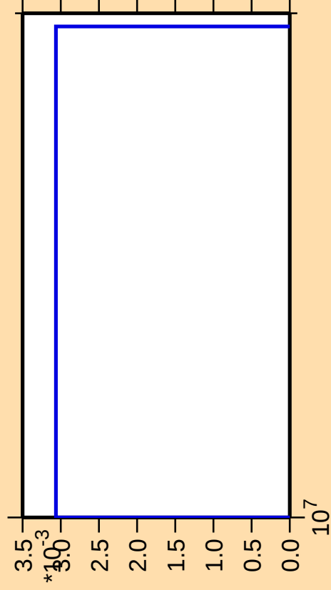
\Delta\sigma/\sigma vs. E for ^{243}\text{Bk}(\text{mt } 34)
