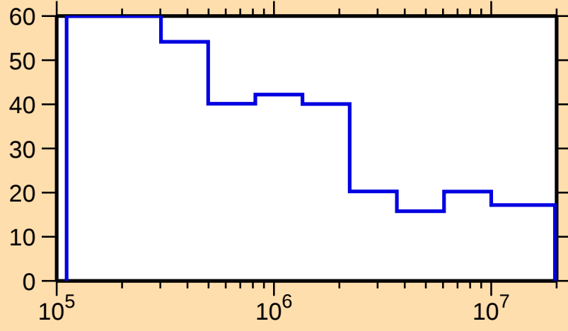
\Delta\sigma/\sigma vs. E for ^{243}\text{Bk}(n,\text{nonel.})
