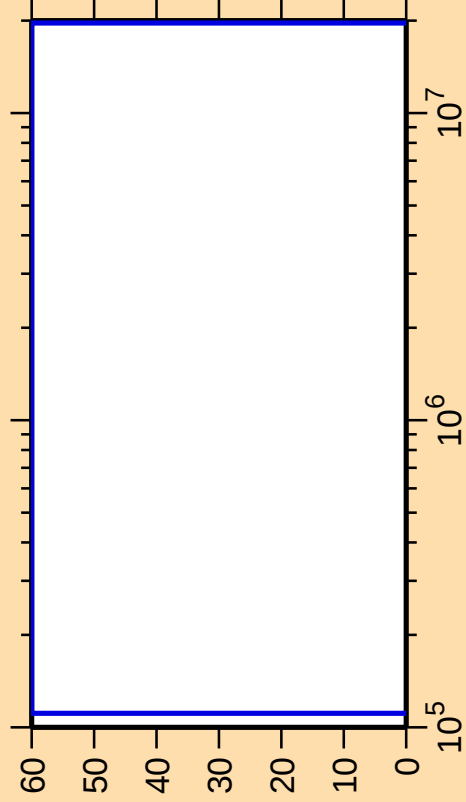
\Delta\sigma/\sigma vs. E for ^{243}\text{Bk}(n,\text{ncont.})
