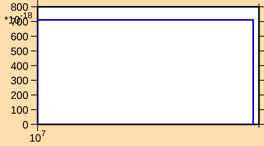
\sigma vs. E for ^{243}\text{Bk}(\text{mt 11})
