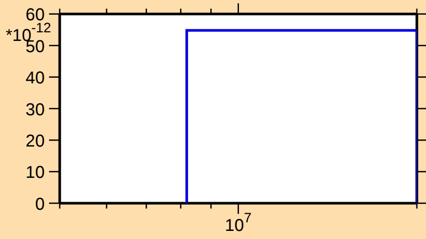
\sigma vs. E for ^{243}\text{Bk}(n,\text{He}3)
