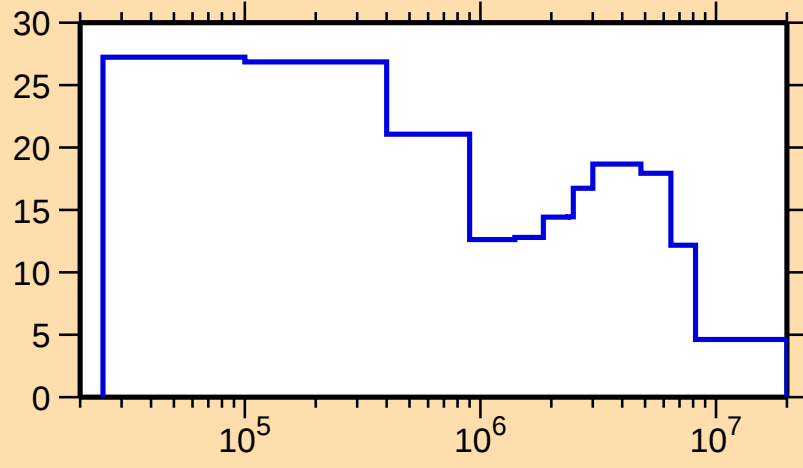
\Delta\sigma/\sigma vs. E for ^{243}\text{Bk}(n,\text{tot.})
