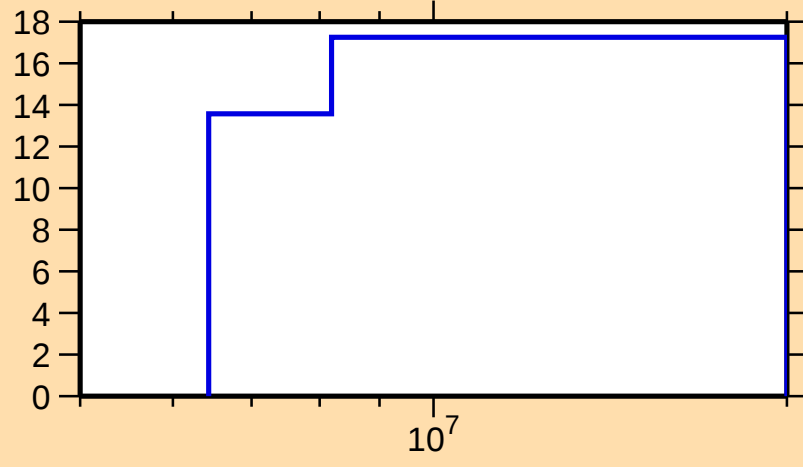
\Delta\sigma/\sigma vs. E for ^{243}\text{Bk}(n,\text{el.})
