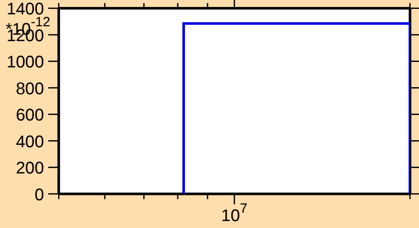
\sigma vs. E for ^{243}\text{Bk}(\text{mt } 45)
