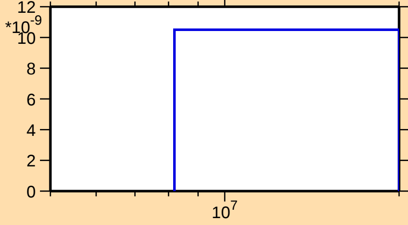
\sigma vs. E for ^{243}\text{Bk}(n,2np)
