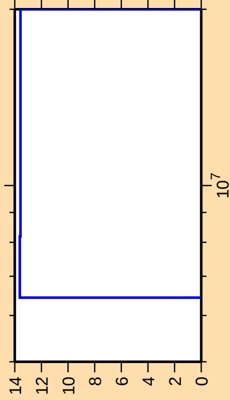
\Delta\sigma/\sigma vs. E for ^{243}\text{Bk}(n,f)
