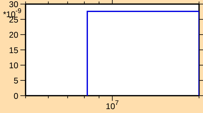
\sigma vs. E for ^{243}\text{Bk}(n,nt)
