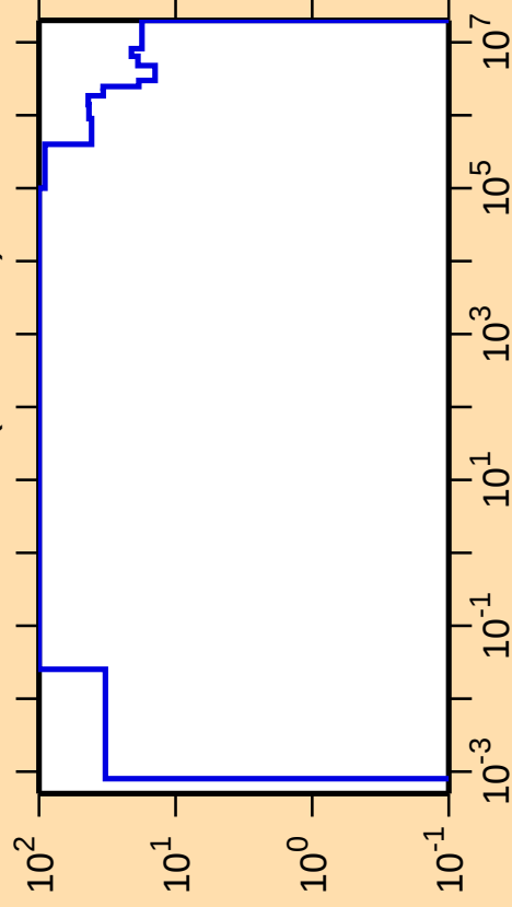
\Delta\sigma/\sigma vs. E for ^{243}\text{Bk}(n,\text{nonel.})
