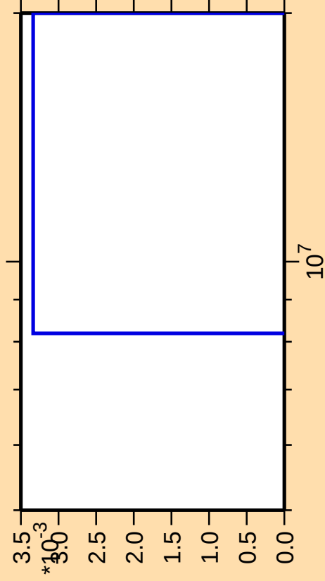
\Delta\sigma/\sigma vs. E for ^{243}\text{Bk}(\text{mt } 34)
