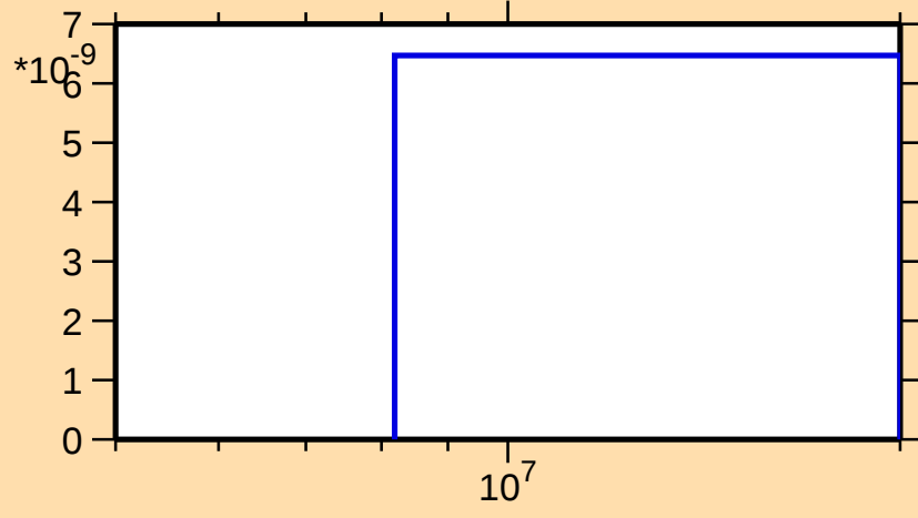
\sigma vs. E for ^{243}\text{Bk}(\text{mt117})
