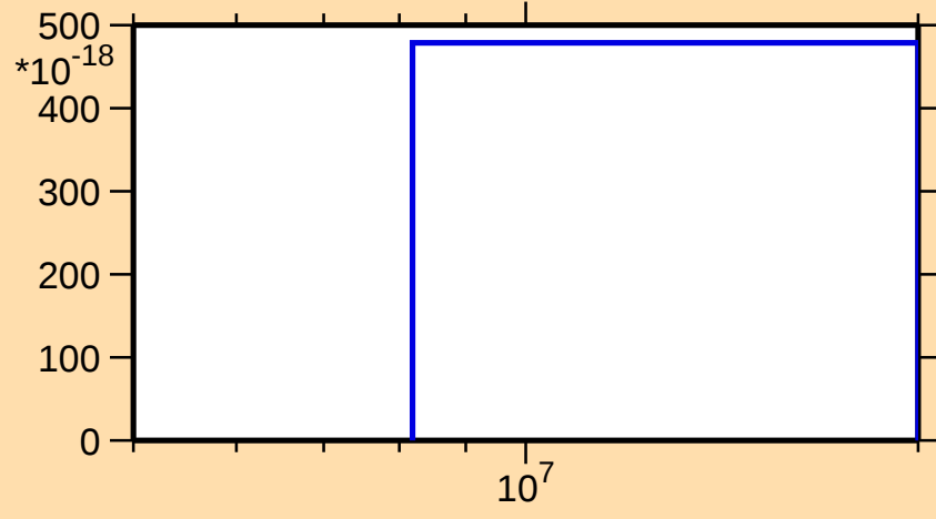
\sigma vs. E for ^{243}\text{Bk}(\text{mt } 34)
