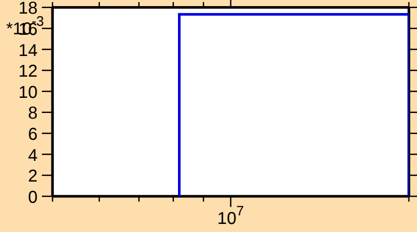
\sigma vs. E for ^{243}\text{Bk}(n,3n)
