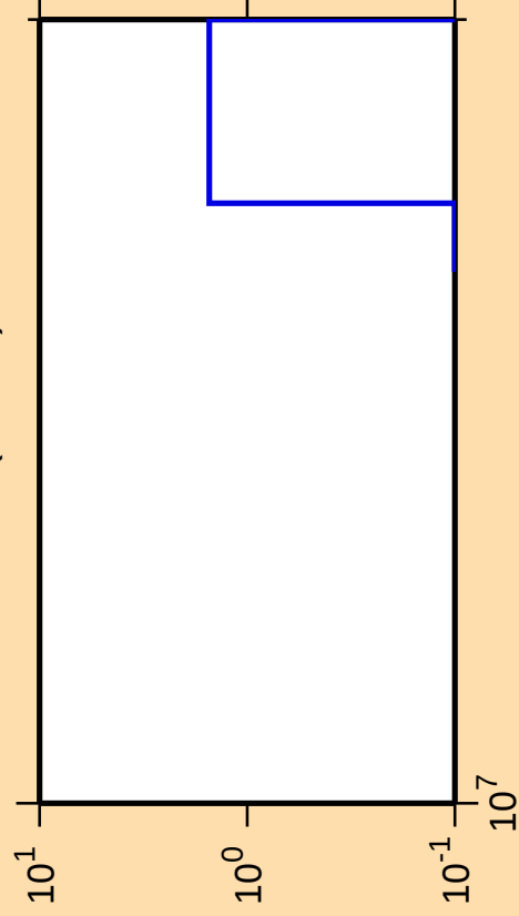
\Delta\sigma/\sigma vs. E for ^{70}\text{Br}(n,2n\alpha)
