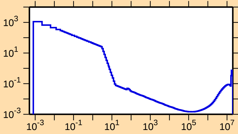
\sigma vs. E for ^{70}\text{Br}(n,p\alpha)
