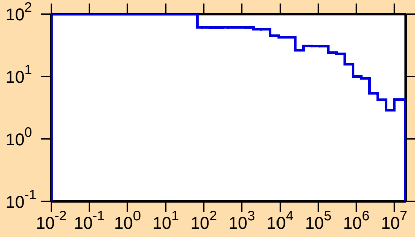
\Delta\sigma/\sigma vs. E for ^{70}\text{Br}(n,\text{nonel.})
