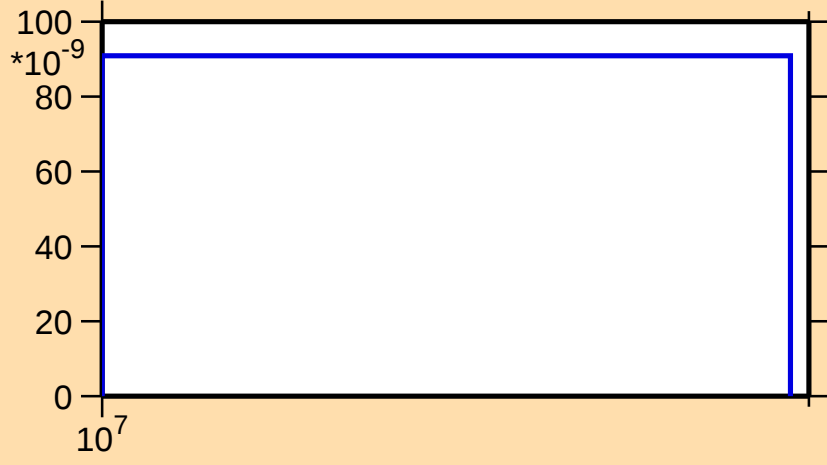
\sigma vs. E for ^{70}\text{Br}(\text{mt } 34)
