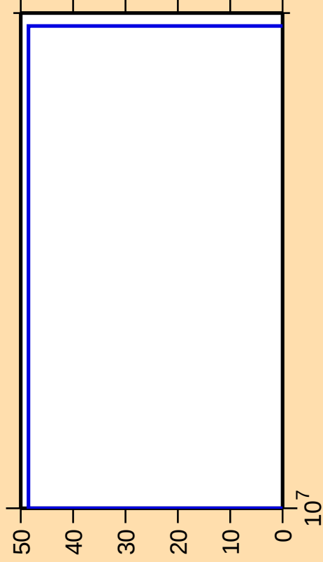
\Delta\sigma/\sigma vs. E for ^{70}\text{Br}(n,2np)
