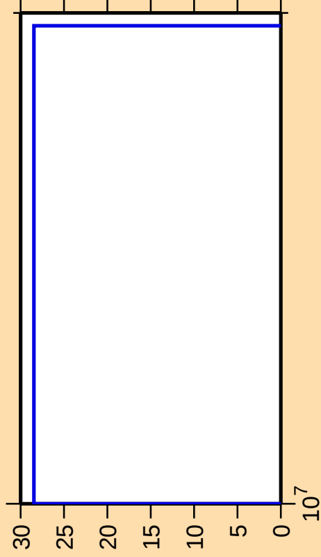
\Delta\sigma/\sigma vs. E for ^{70}\text{Br}(n,n_1)
