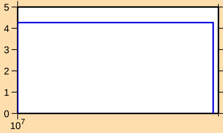
\Delta\sigma/\sigma vs. E for ^{70}\text{Br}(n,\text{nonel.})
