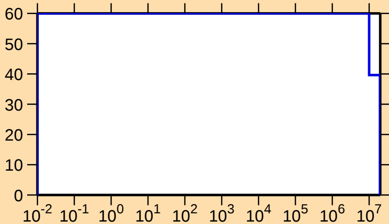
\Delta\sigma/\sigma vs. E for ^{70}\text{Br}(n,\gamma)
