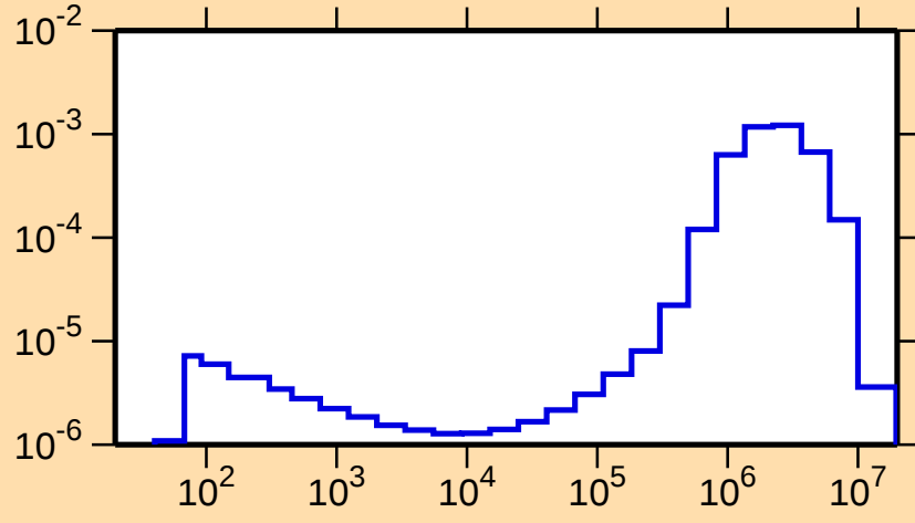
\sigma vs. E for ^{70}\text{Br}(n,\text{inel.})
