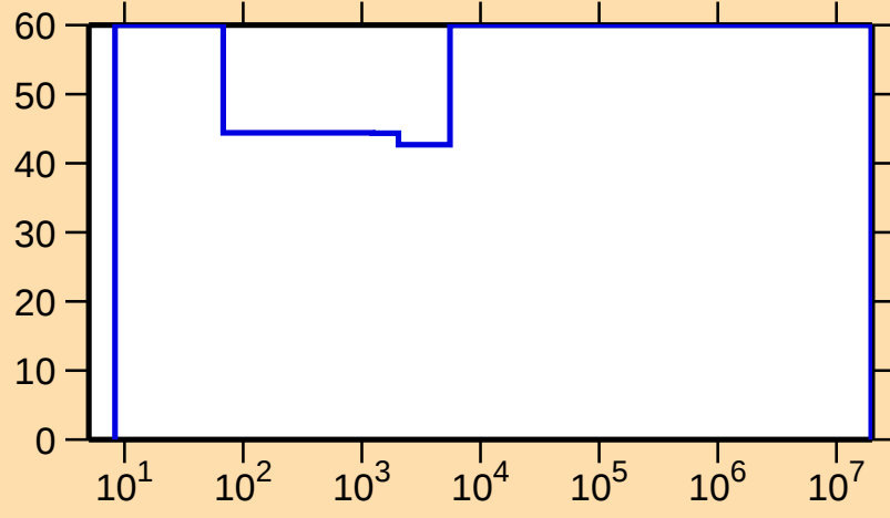
\Delta\sigma/\sigma vs. E for ^{70}\text{Br}(n,n\text{cont.})
