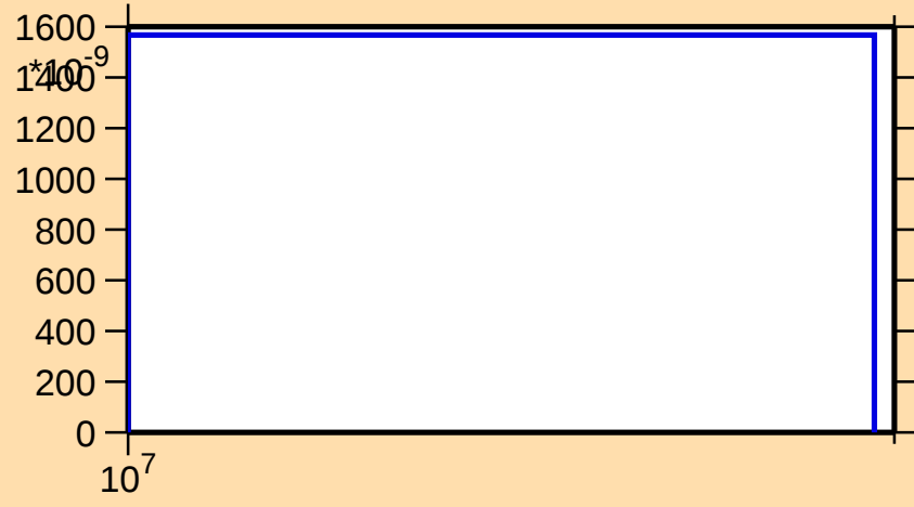
\sigma vs. E for ^{70}\text{Br}(n,2np)
