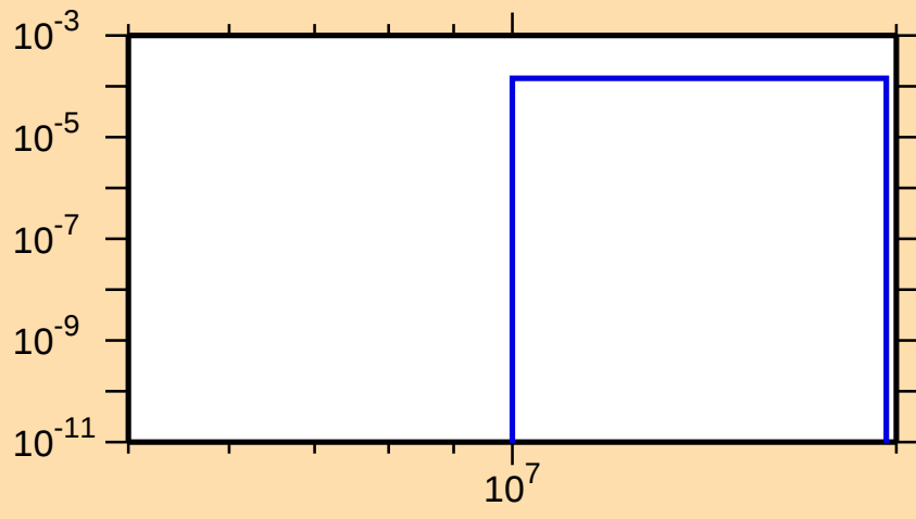
\sigma vs. E for ^{70}\text{Br}(n,\text{pt})
