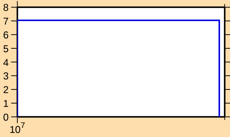
\Delta\sigma/\sigma vs. E for ^{70}\text{Br}(n,\text{tot.})
