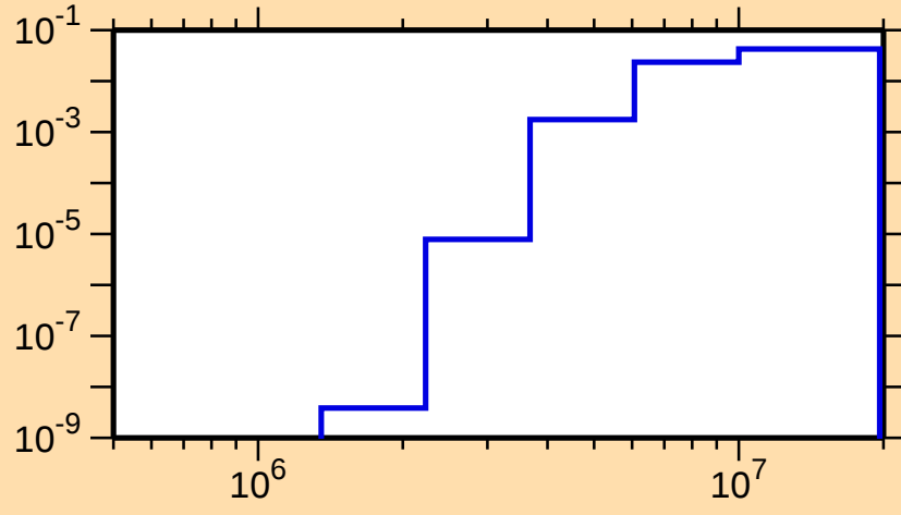
\sigma vs. E for ^{70}\text{Br}(n,np)
