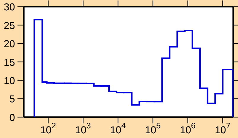
\Delta\sigma/\sigma vs. E for ^{70}\text{Br}(n,\text{el.})
