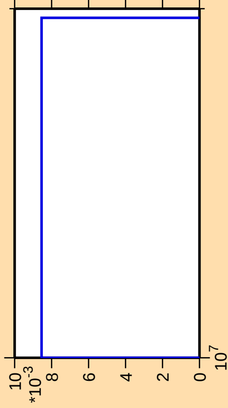
\Delta\sigma/\sigma vs. E for ^{70}\text{Br}(n,2n\alpha)
