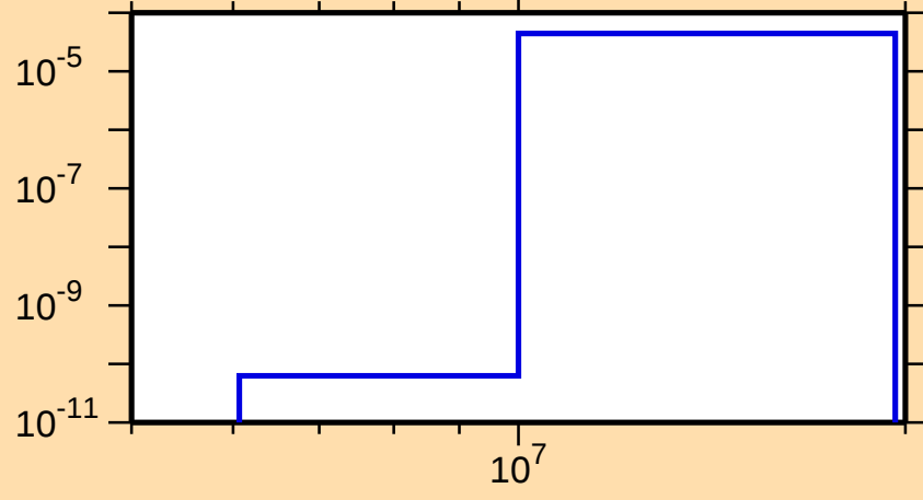
\sigma vs. E for ^{70}\text{Br}(\text{mt } 45)
