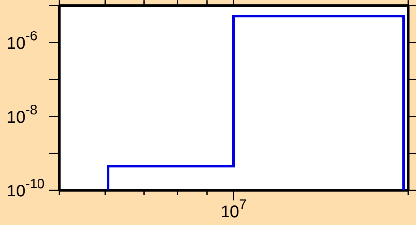
\sigma vs. E for ^{70}\text{Br}(\text{mt117})
