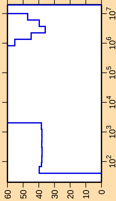
\Delta\sigma/\sigma vs. E for ^{70}\text{Br}(n,\text{inel.})
