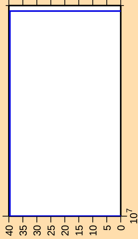
\Delta\sigma/\sigma vs. E for ^{70}\text{Br}(n,\gamma)
