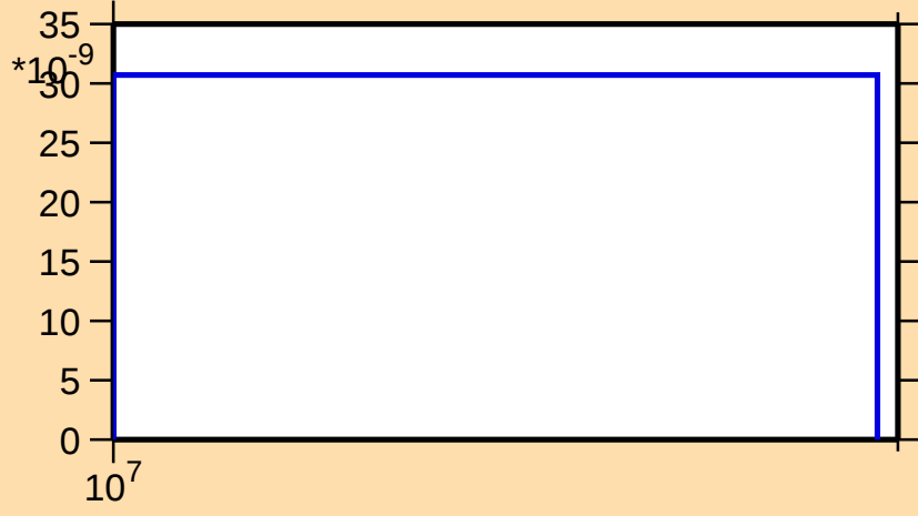
\sigma vs. E for ^{70}\text{Br}(n,2n)
