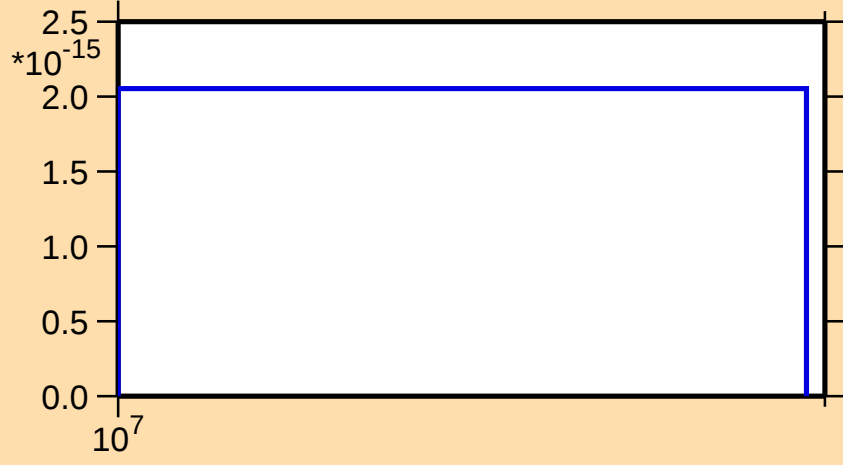
\sigma vs. E for ^{70}\text{Br}(n,2n\alpha)
