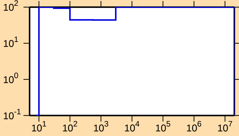
\Delta\sigma/\sigma vs. E for ^{70}\text{Br}(n,n\text{cont.})
