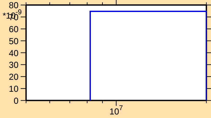
\sigma vs. E for ^{70}\text{Br}(\text{mt } 34)
