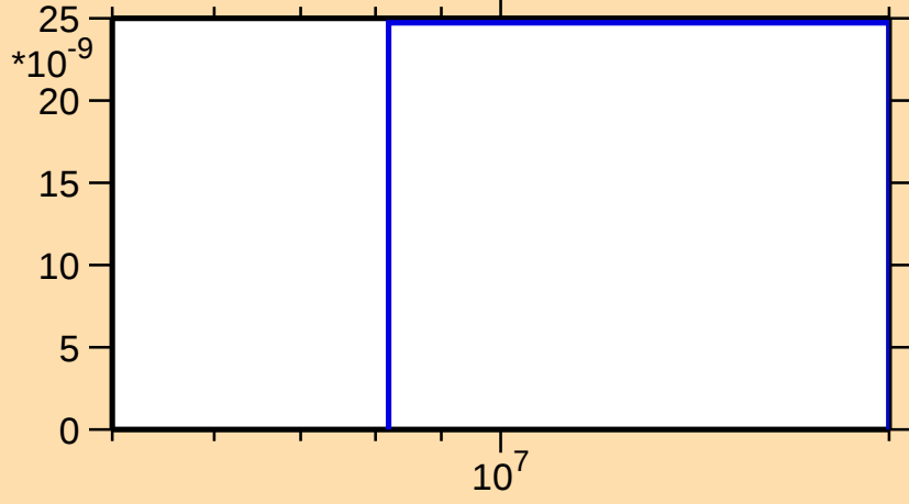
\sigma vs. E for ^{70}\text{Br}(n,2n)
