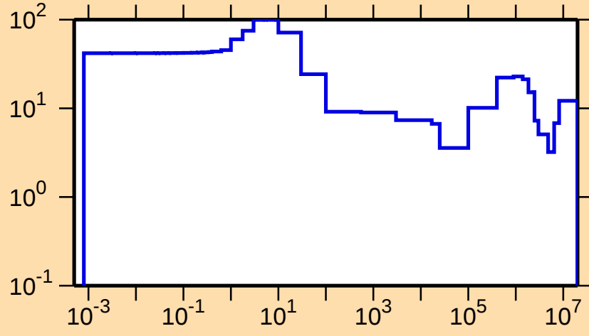
\Delta\sigma/\sigma vs. E for ^{70}\text{Br}(n,\text{el.})
