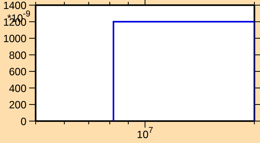
\sigma vs. E for ^{70}\text{Br}(n,\text{nd})
