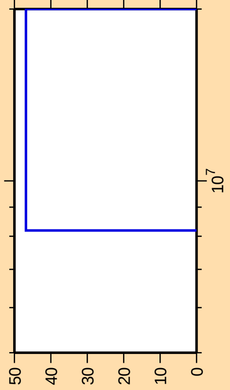
\Delta\sigma/\sigma vs. E for ^{70}\text{Br}(n,\gamma)
