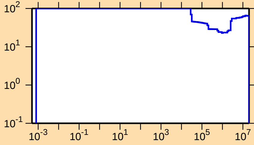
\Delta\sigma/\sigma vs. E for ^{71}\text{Br}(n,p)
