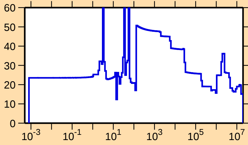
\Delta\sigma/\sigma vs. E for ^{71}\text{Br}(n,\text{el.})
