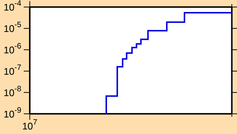
\sigma vs. E for ^{71}\text{Br}(n,2n)
