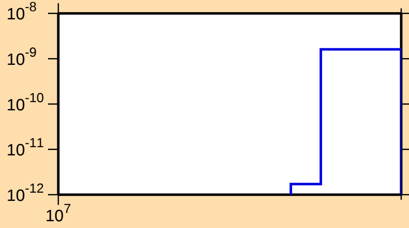
\sigma vs. E for ^{71}\text{Br} (mt 34)
