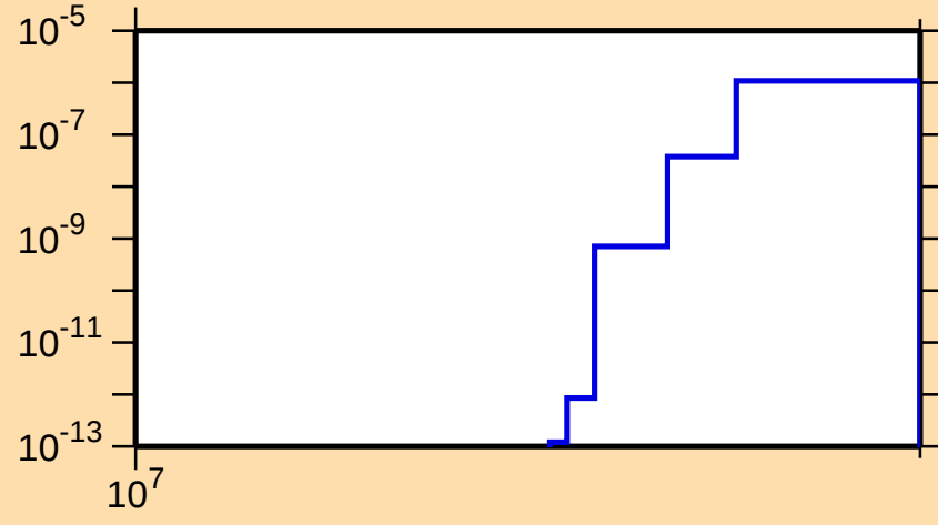
\sigma vs. E for ^{71}\text{Br}(n,\text{nd})
