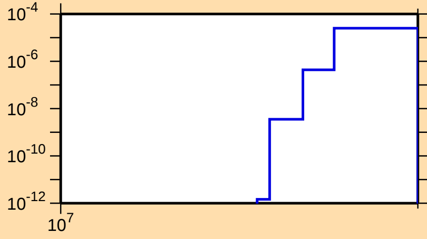
\sigma vs. E for ^{71}\text{Br}(n,\text{pt})
