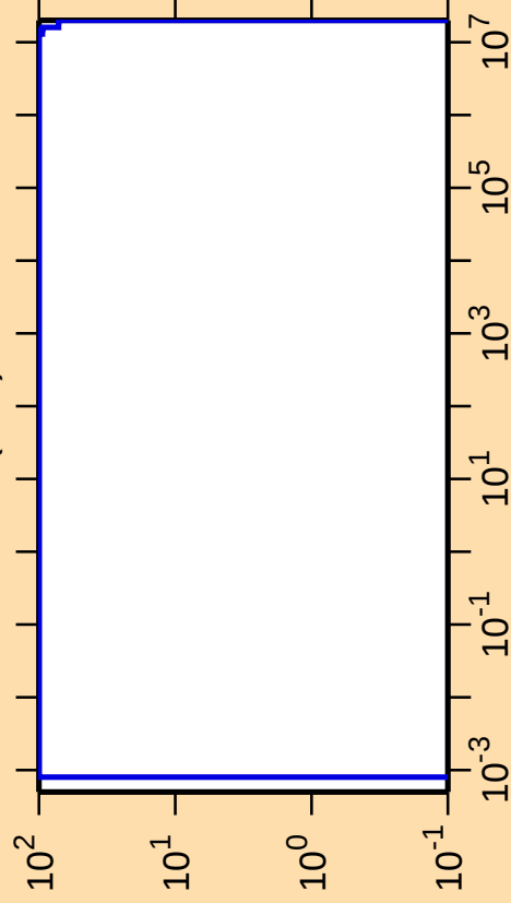
\Delta\sigma/\sigma vs. E for ^{71}\text{Br}(n,\alpha)
