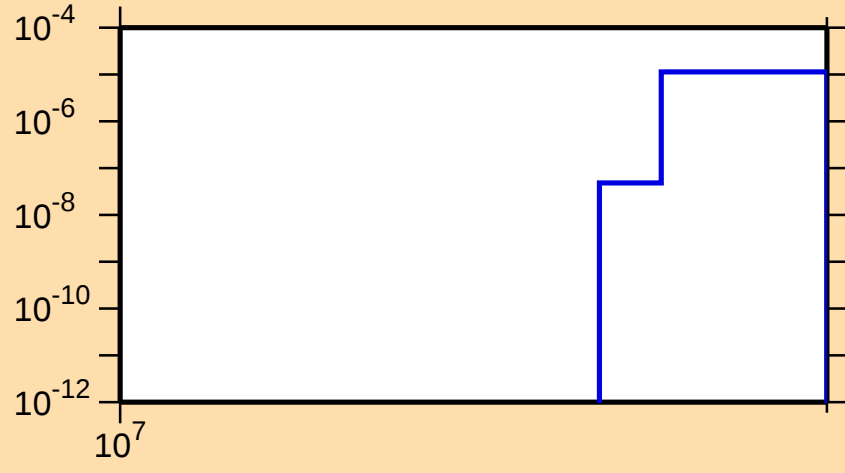
\sigma vs. E for ^{71}\text{Br}(n,2np)
