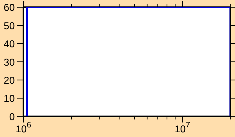
\Delta\sigma/\sigma vs. E for ^{71}\text{Br}(n,n\text{cont.})
