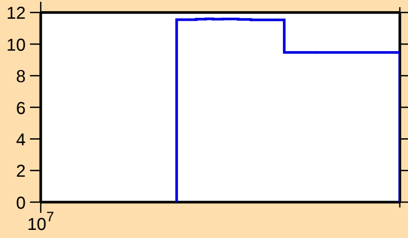
\Delta\sigma/\sigma vs. E for ^{71}\text{Br}(n,\text{tot.})
