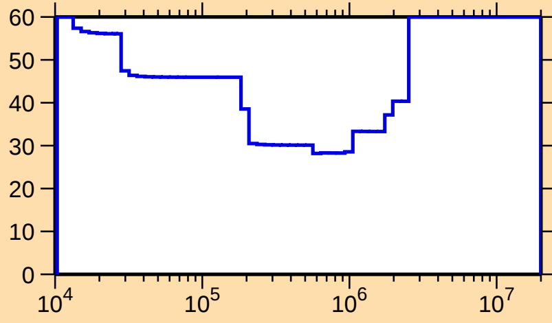
\Delta\sigma/\sigma vs. E for ^{71}\text{Br}(n,\text{inel.})
