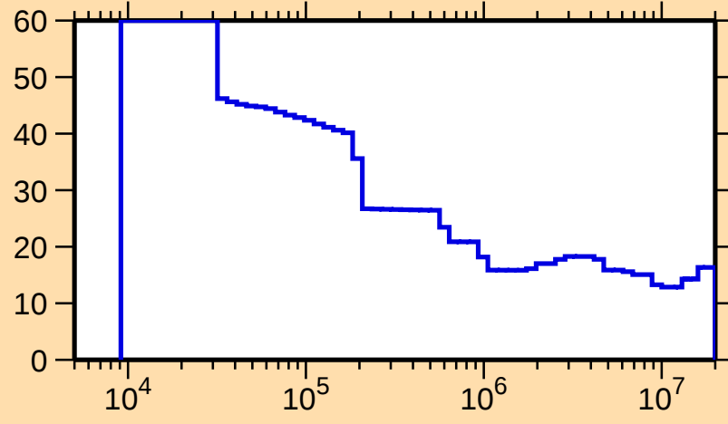
\Delta\sigma/\sigma vs. E for ^{71}\text{Br}(n,\text{nonel.})
