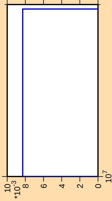
\Delta\sigma/\sigma vs. E for ^{71}\text{Br}(n,\text{nt})
