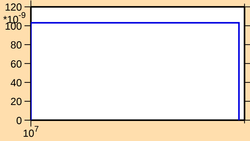
\sigma vs. E for ^{71}\text{Br}(n,2np)
