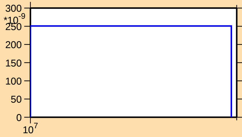
\sigma vs. E for ^{71}\text{Br}(n,\text{pt})
