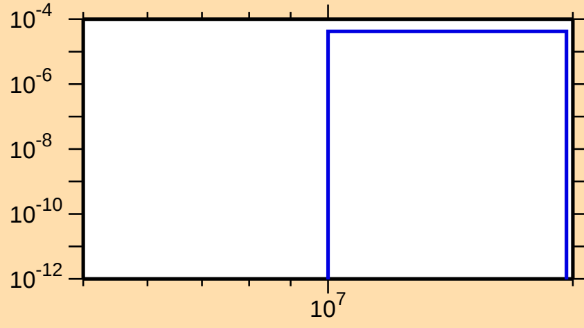
\sigma vs. E for ^{71}\text{Br}(\text{mt } 45)
