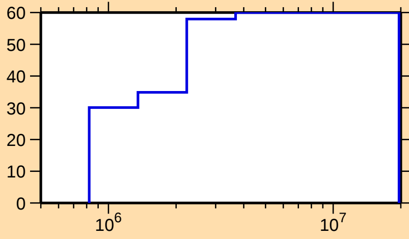
\Delta\sigma/\sigma vs. E for ^{71}\text{Br}(\text{n},\text{inel.})
