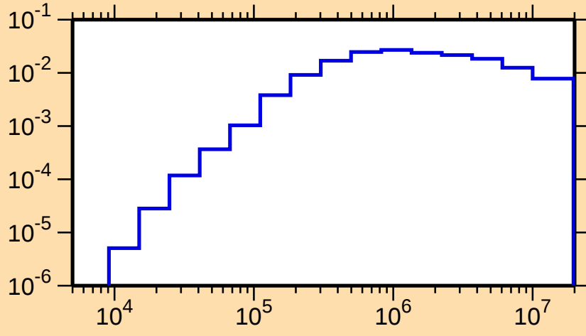
\sigma vs. E for ^{71}\text{Br}(n,n_1)
