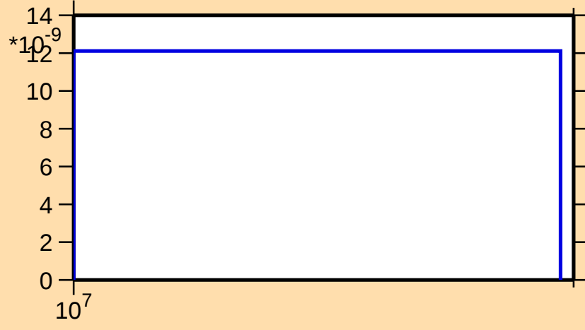
\sigma vs. E for ^{71}\text{Br}(n,\text{nd})
