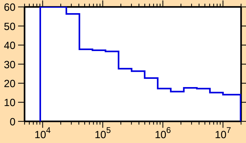
\Delta\sigma/\sigma vs. E for ^{71}\text{Br}(\text{n,nonel.})
